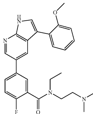
MS: m/z 461 (M+H + )
