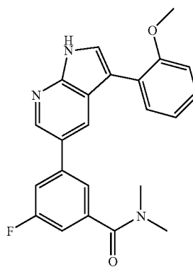
MS: m/z 390 (M+H + )
