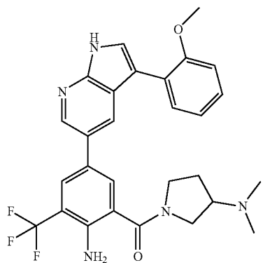
AE118 MS: m/z 524 (M+H + )
