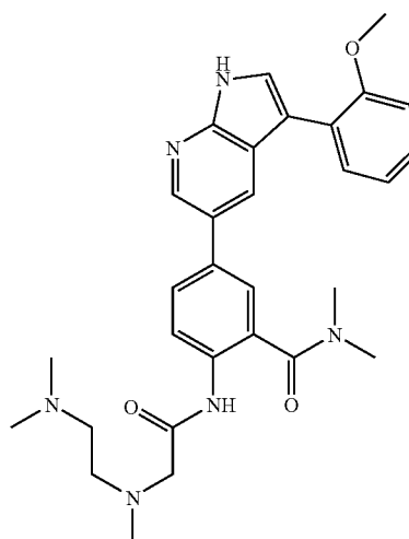
AE120 MS: m/z 529 (M+H + )
