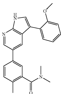
MS: m/z 386 (M+H + )
