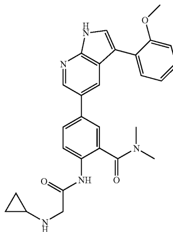
MS: m/z 484 (M+H + )
