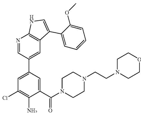
MS: m/z 575 (M+H + )
