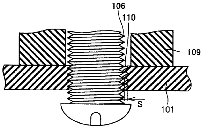
FIG.9 PRIOR ART
