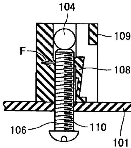
FIG.11 PRIOR ART
