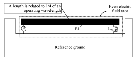
Magnetic current loop monopole antenna
