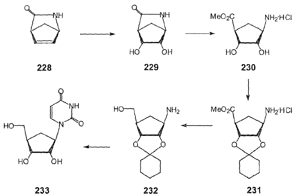
Scheme 31
