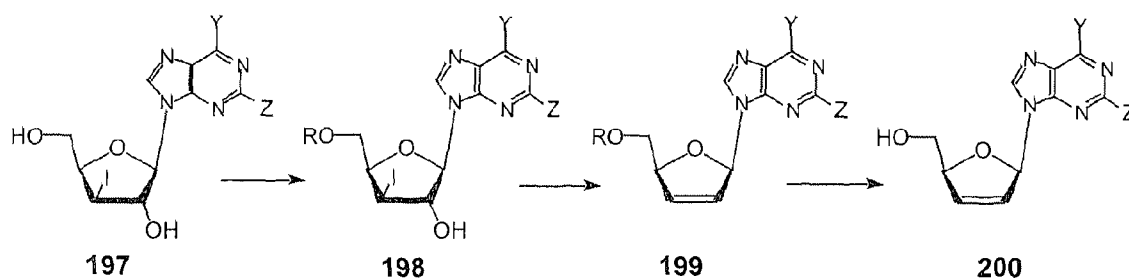
Scheme 27
