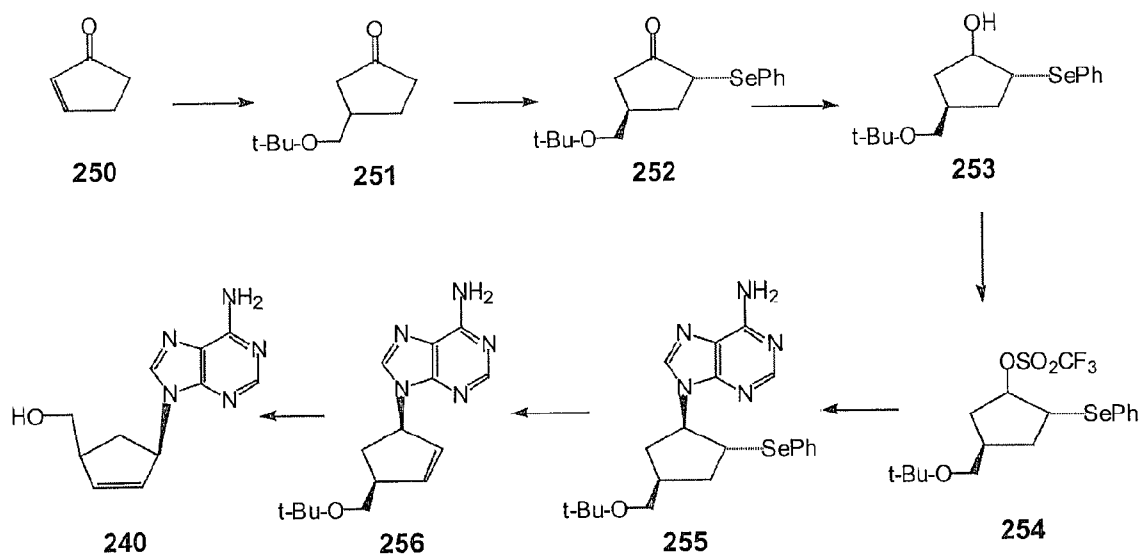
Scheme 34
