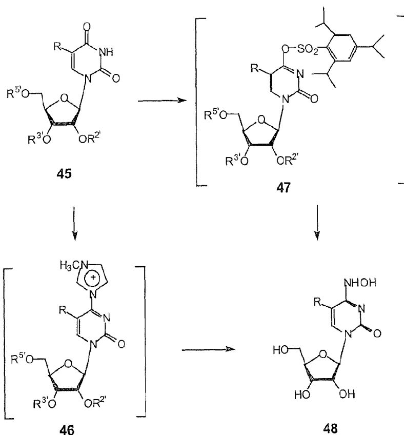
Scheme 8
