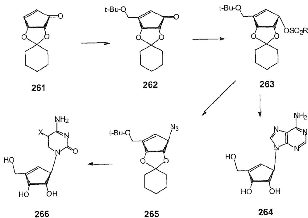
Scheme 36
