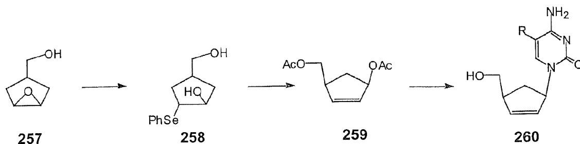
Scheme 35
