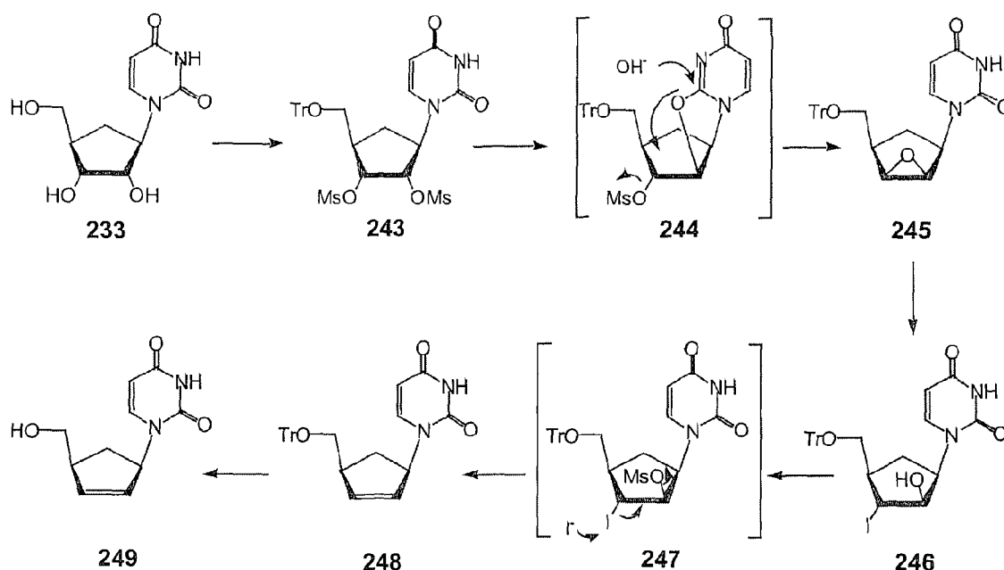
Scheme 33
