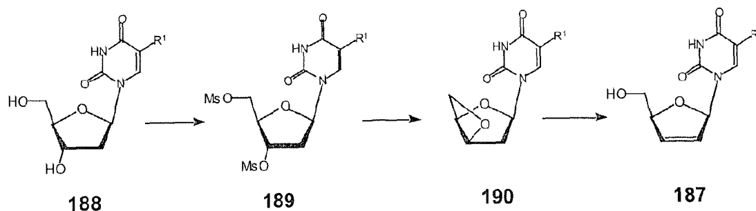
Scheme 25
