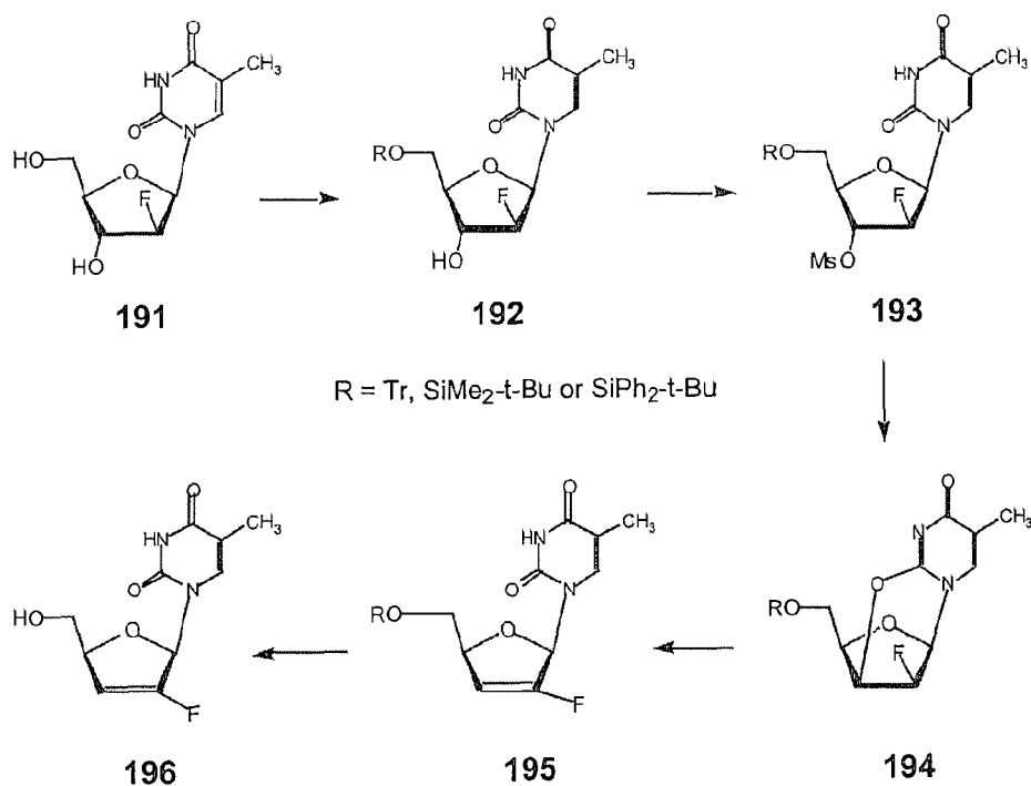
Scheme 26
