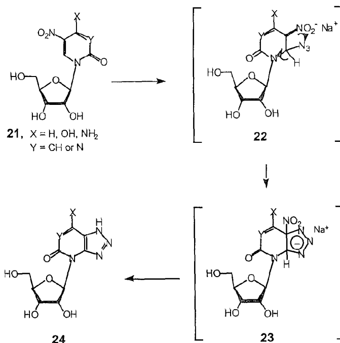
Scheme 4
