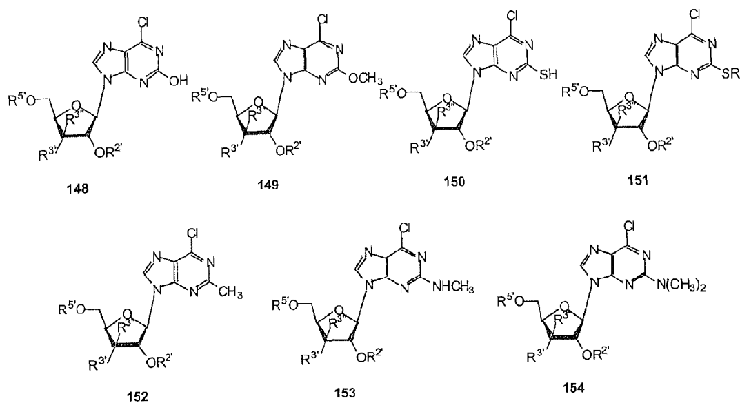
Scheme 20
