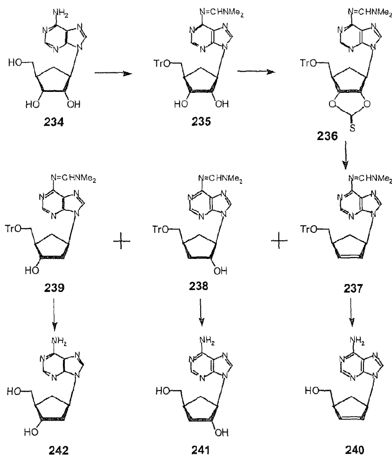
Scheme 32
