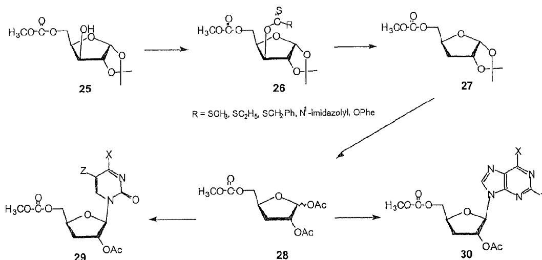
Scheme 5
