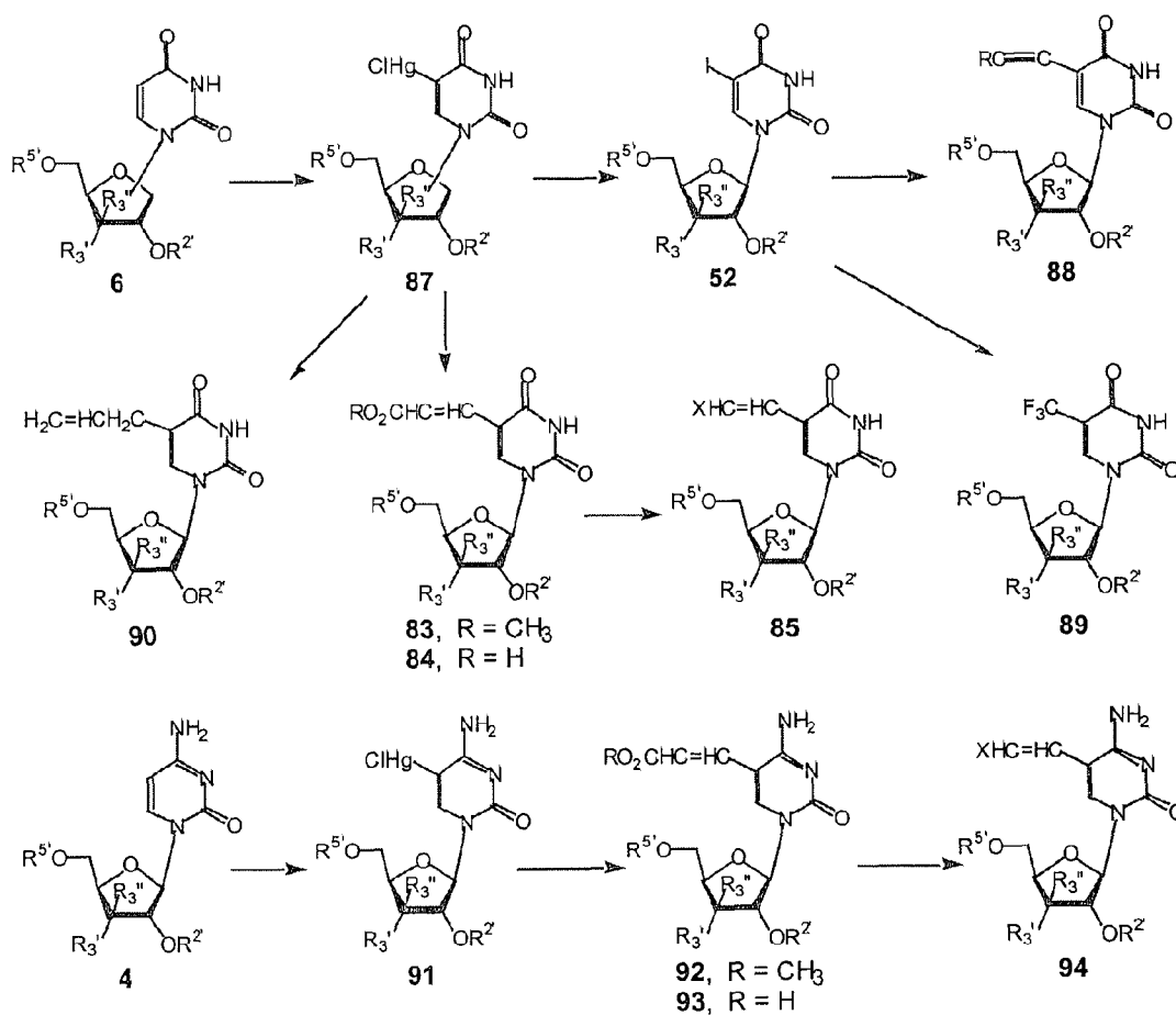
Scheme 14
