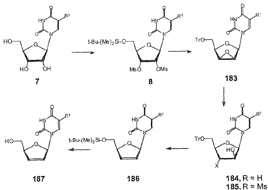
Scheme 24
