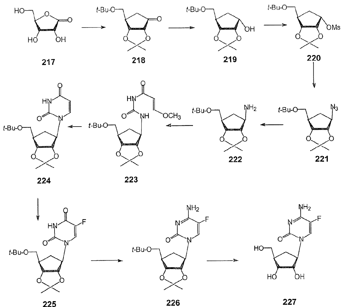
Scheme 30
