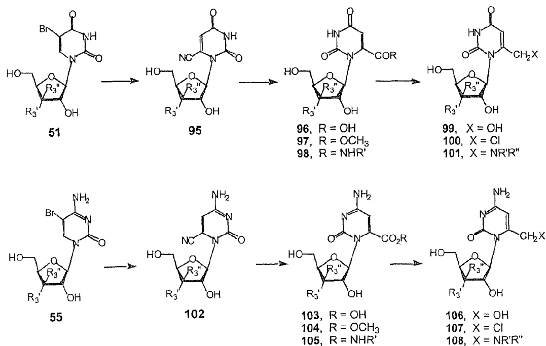
Scheme 15
