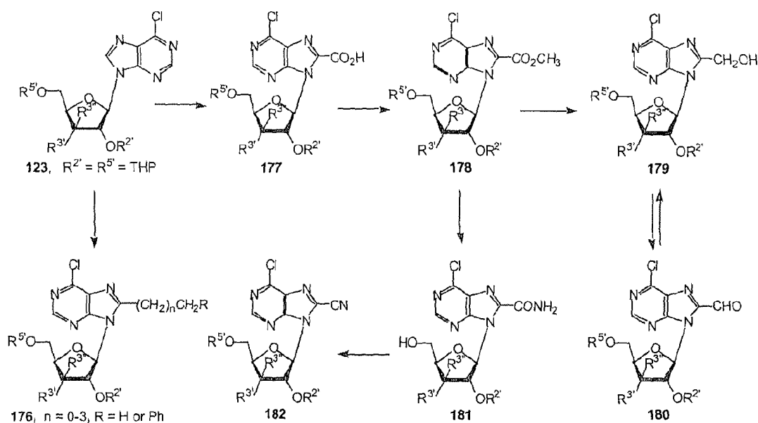
Scheme 23
