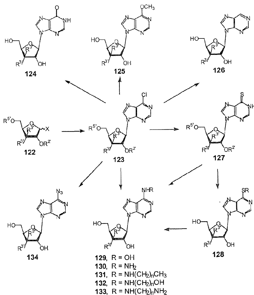
Scheme 18
