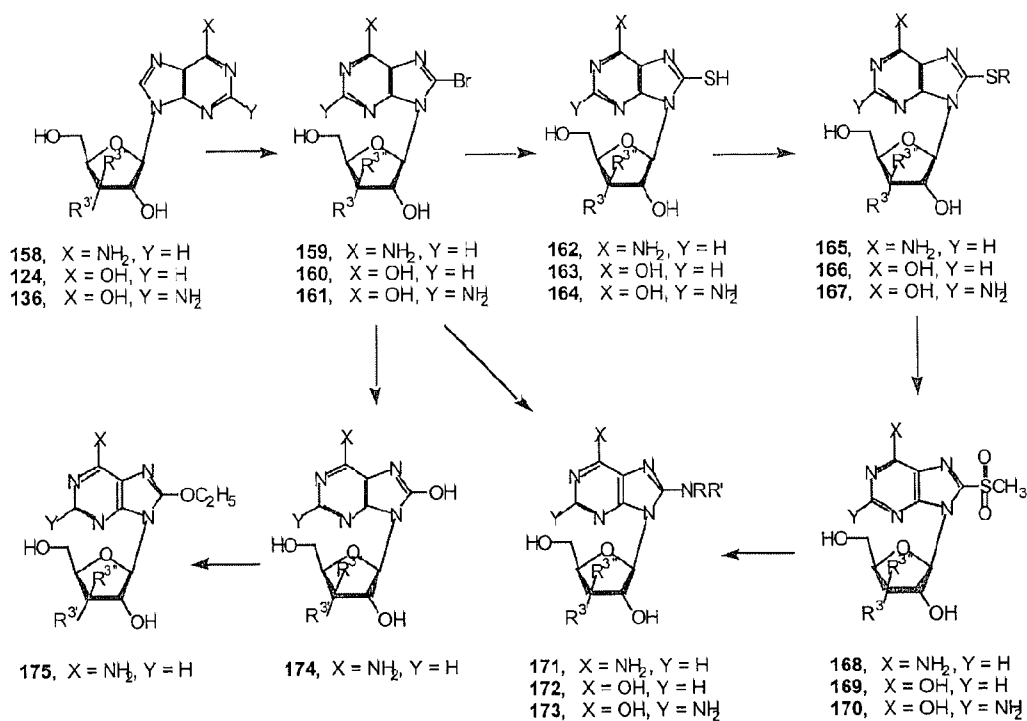
Scheme 22
