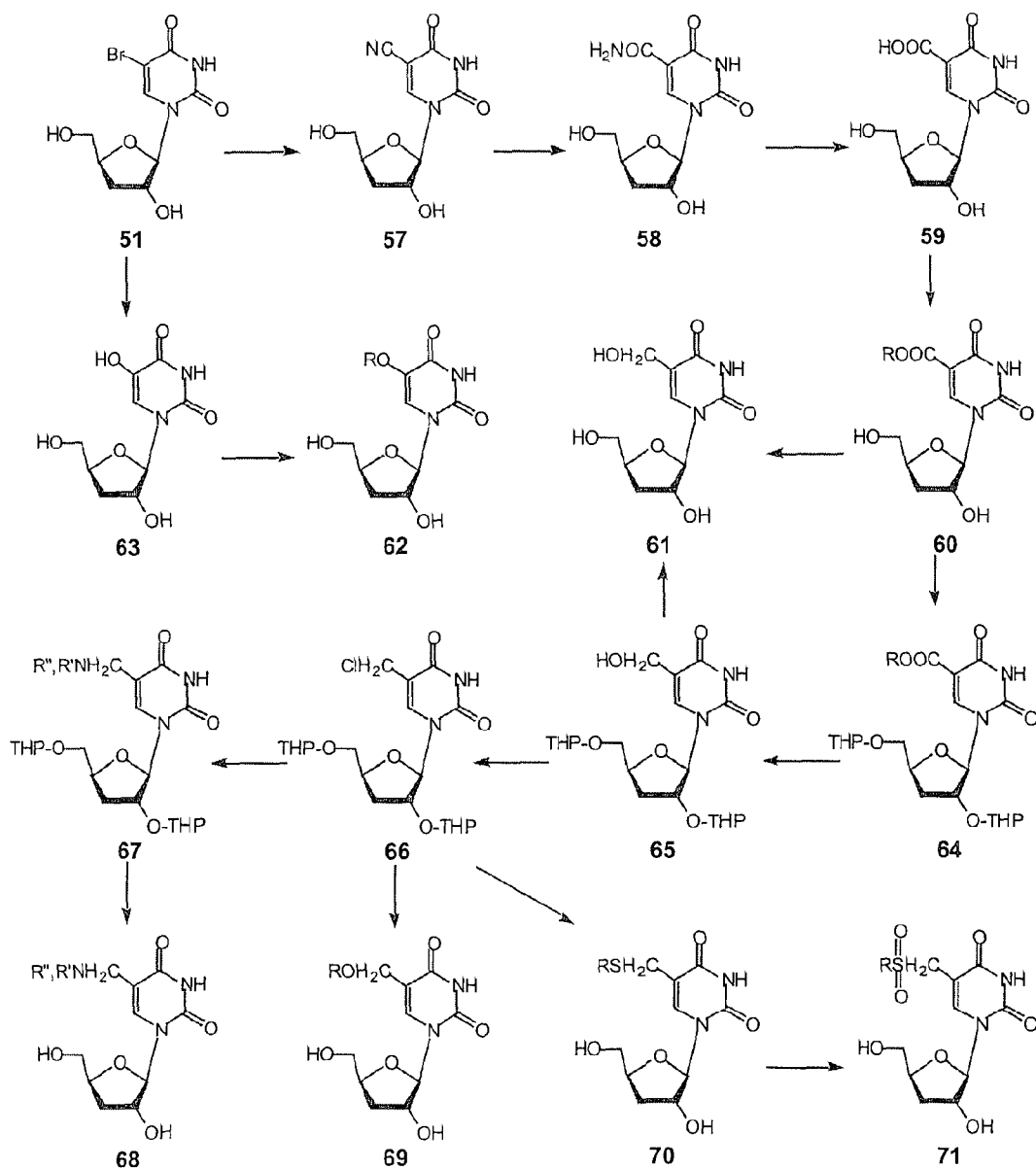
Scheme 10
