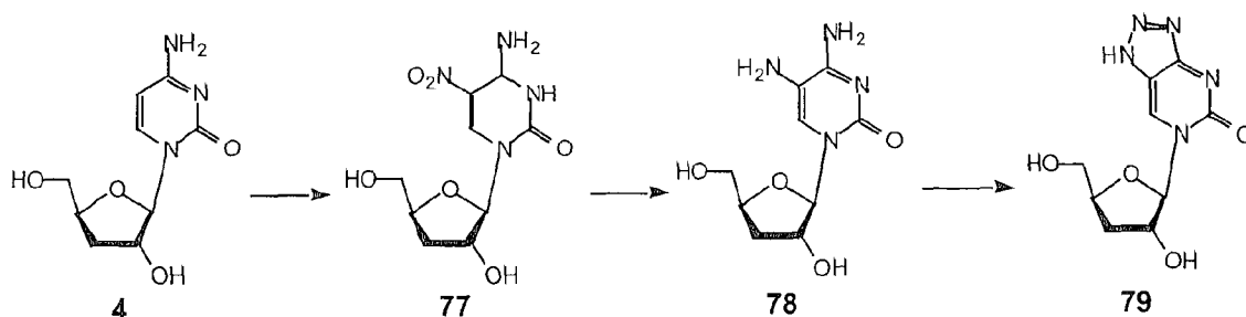
Scheme 12
