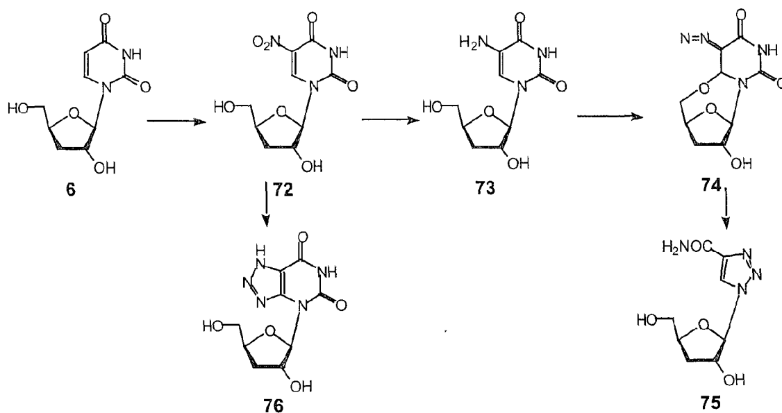
Scheme 11
