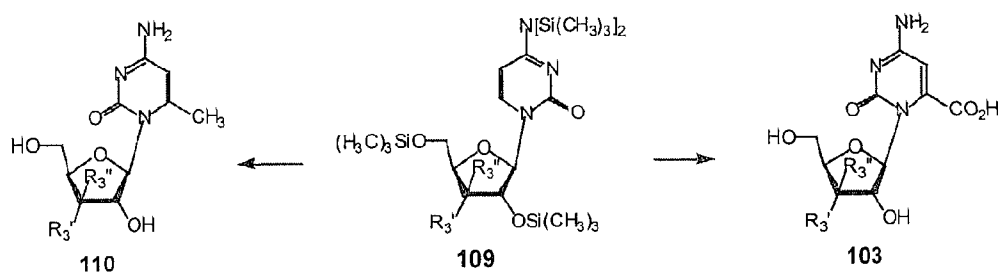
Scheme 16
