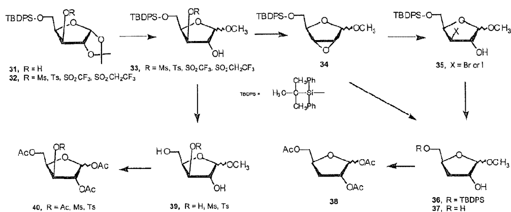
Scheme 6
