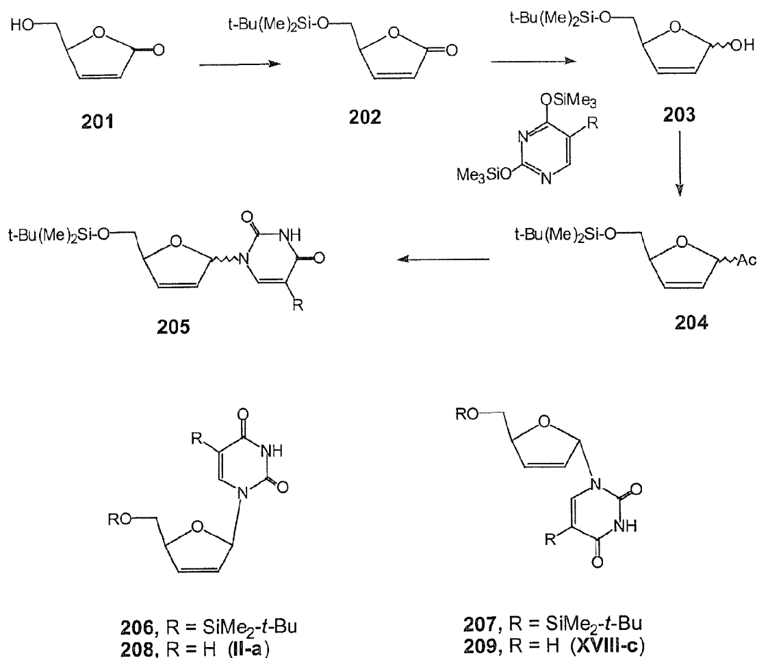
Scheme 28
