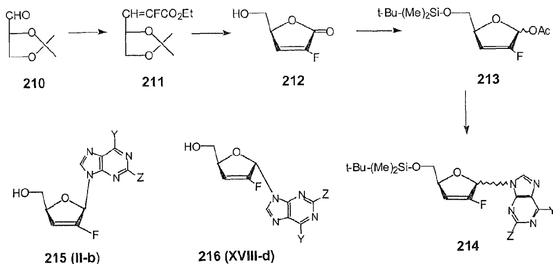
Scheme 29
