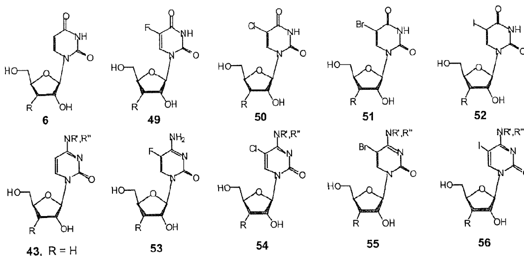
Scheme 9
