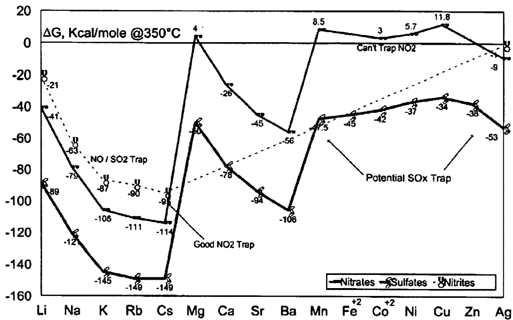
Fig. 1: Free Energies of Formation of Nitrates, Sulfates, &amp; Nitrites
