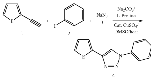
Scheme 2: Synthetic scheme for the preparation of compounds of Formula Ia
