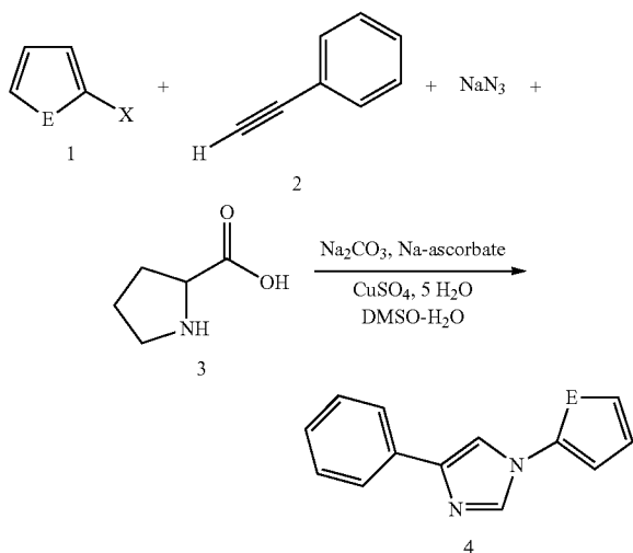
Scheme 6: Synthetic scheme for the preparation of compounds of Formula IIa
