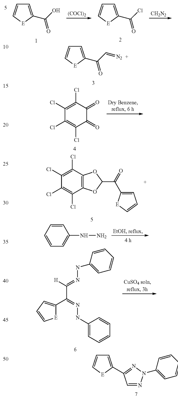
Scheme 5: Synthetic scheme for the preparation of compounds of Formula Id
