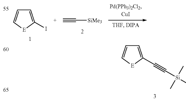
Scheme 1: Synthetic scheme for the preparation of compounds of Formula Ia
