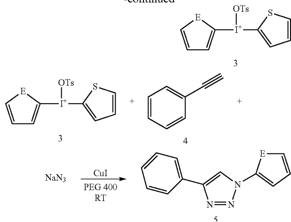
5 Scheme 8: Synthetic scheme for the preparation of compounds of Formula IIc
