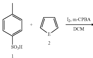
Scheme 7: Synthetic scheme for the preparation of compounds of Formula IIa
