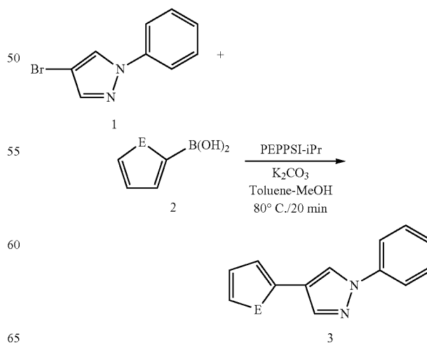
Scheme 3: Synthetic scheme for the preparation of compounds of Formula Ib
