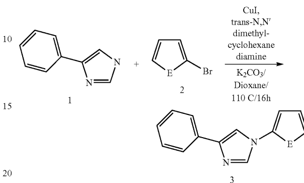
5 Scheme 8: Synthetic scheme for the preparation of compounds of Formula IIc
