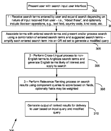
Combined Semantic Search Expansion/Query Modification; Cross-Lingual Searching; and Relevancy Ranking Process
