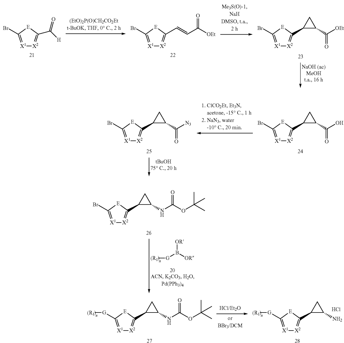
SCHEME 3: ACN (acetonitrile), DCM (dichloromethane), DMSO (Dimethyl sulfoxide), THF (Tetrahydrofuran)
