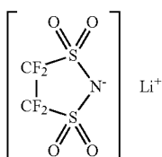
[Chemical formula 35]
