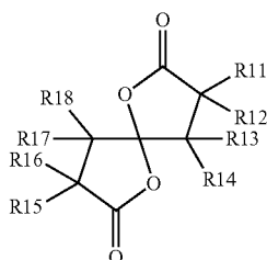
[Chemical formula 39]
