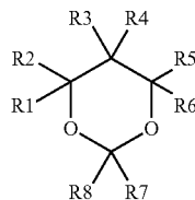
[Chemical formula 8]
