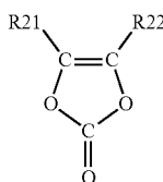
[Chemical formula 22]
