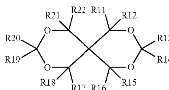
[Chemical formula 9]
