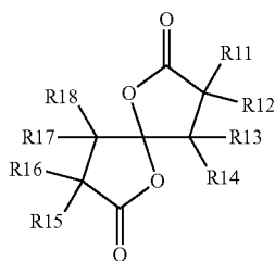
[Chemical formula 7]
