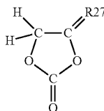
[Chemical formula 24]
