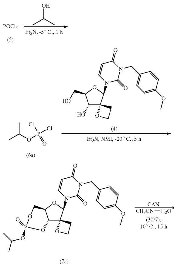
Scheme 2 Synthesis of compound (8a)
