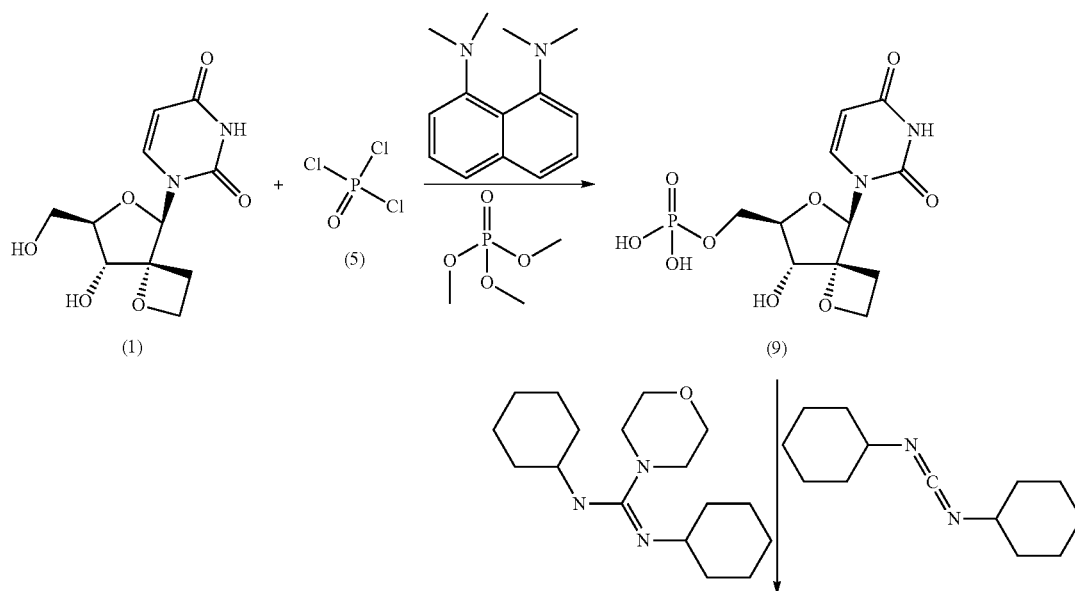
Scheme 3 Synthesis of compound (VI)
