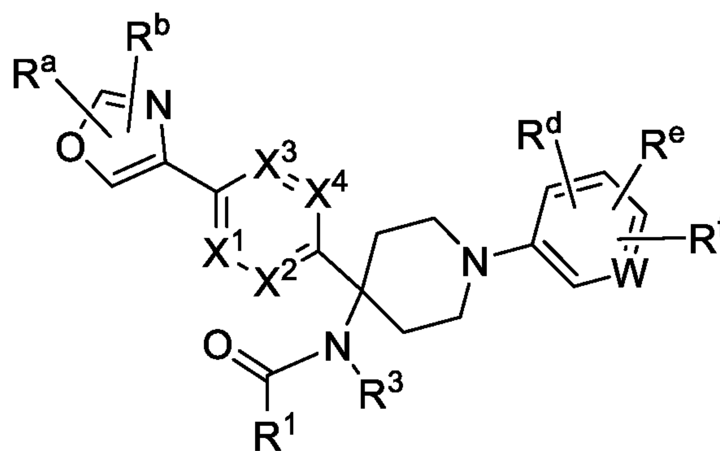
Formula (Vn)
