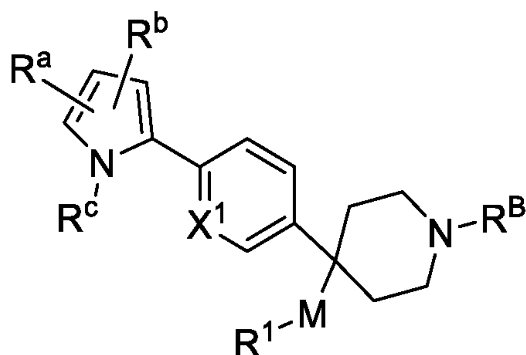
Formula (Xc)
