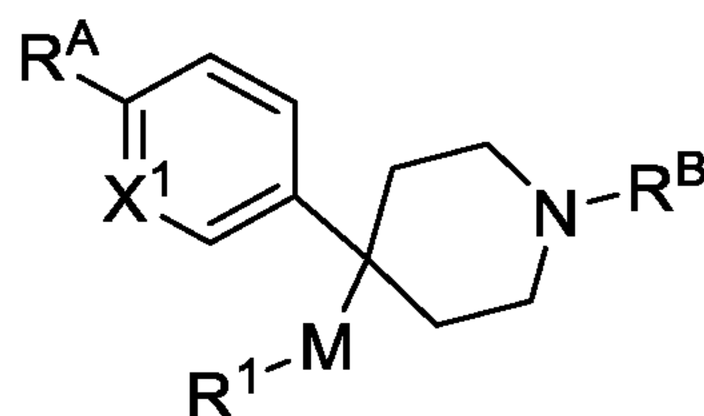
Formula (IXa)
