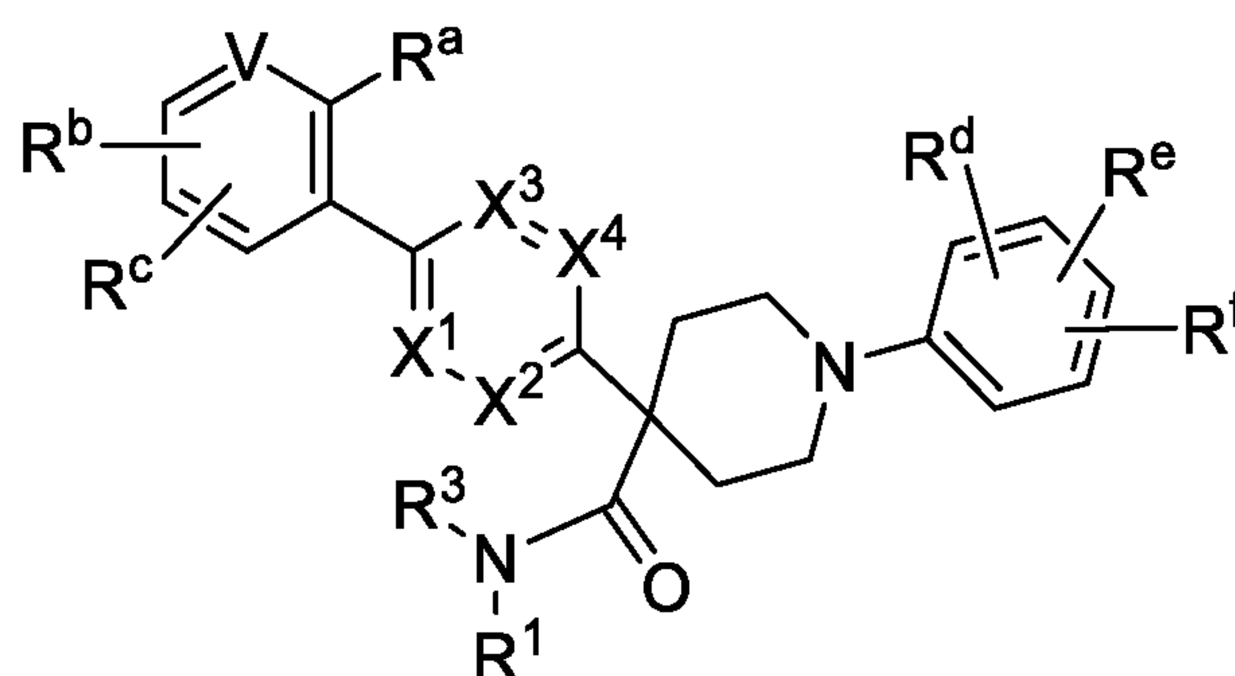
Formula (VIb)
