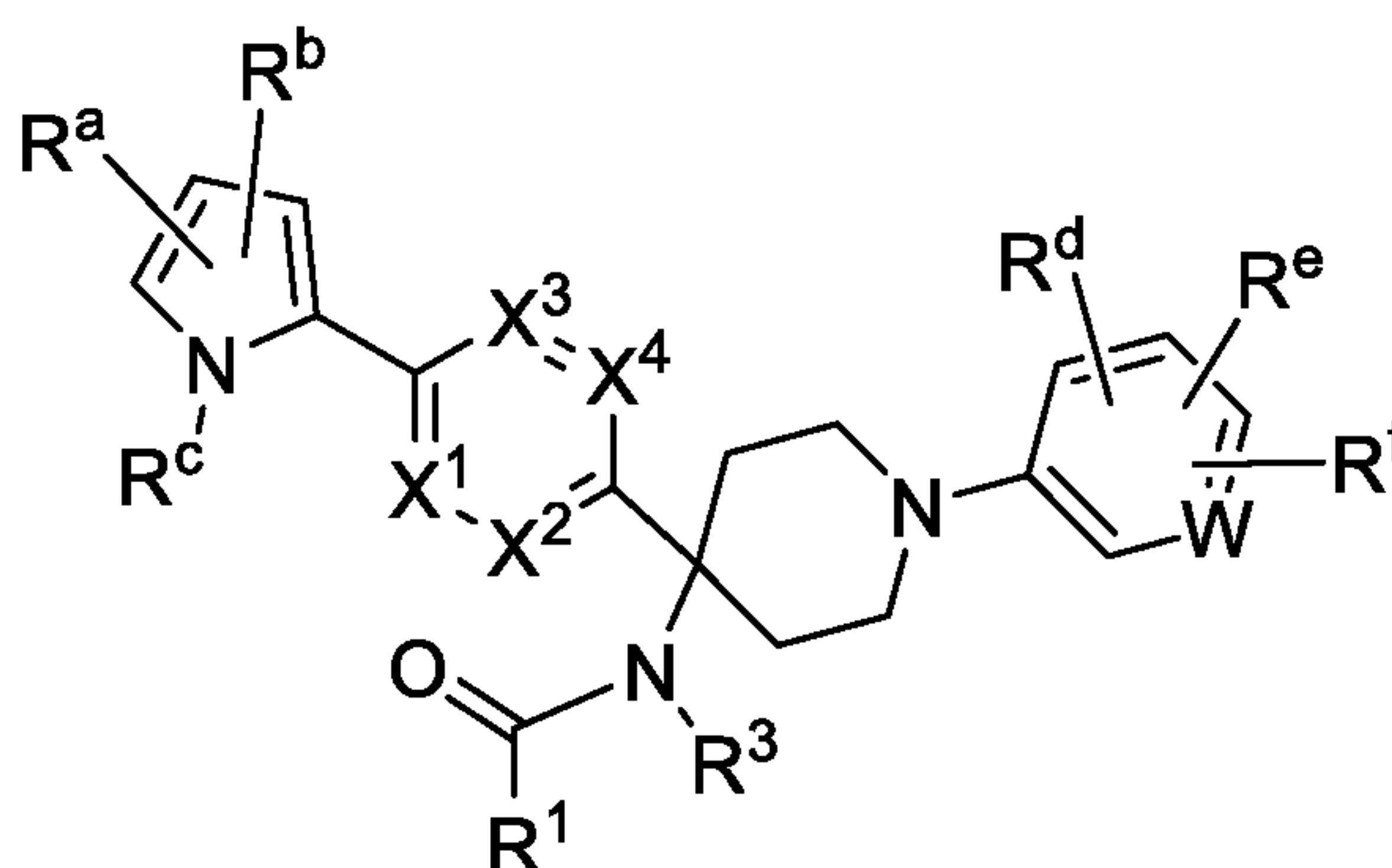
Formula (Vk)
