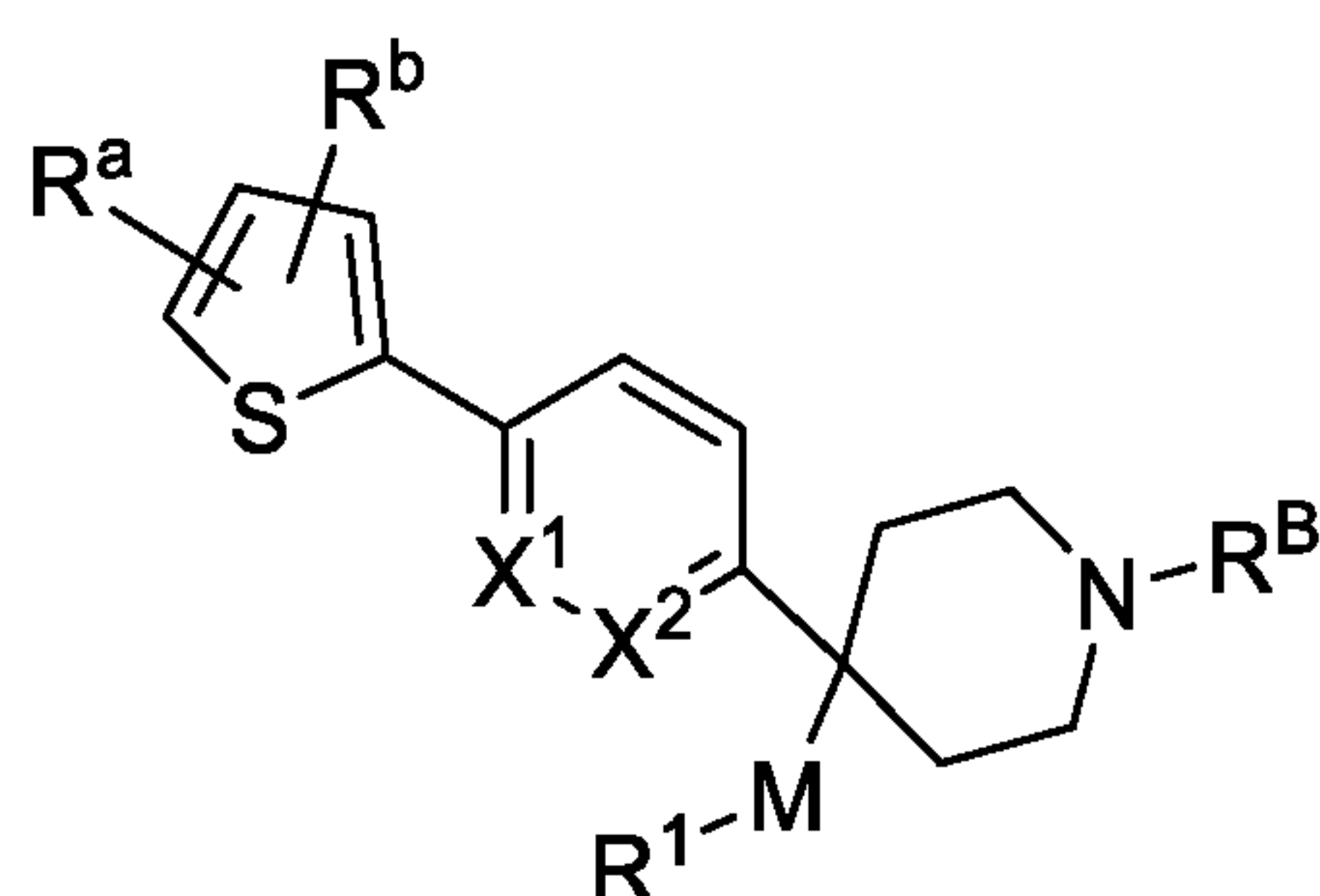
Formula (XII).
