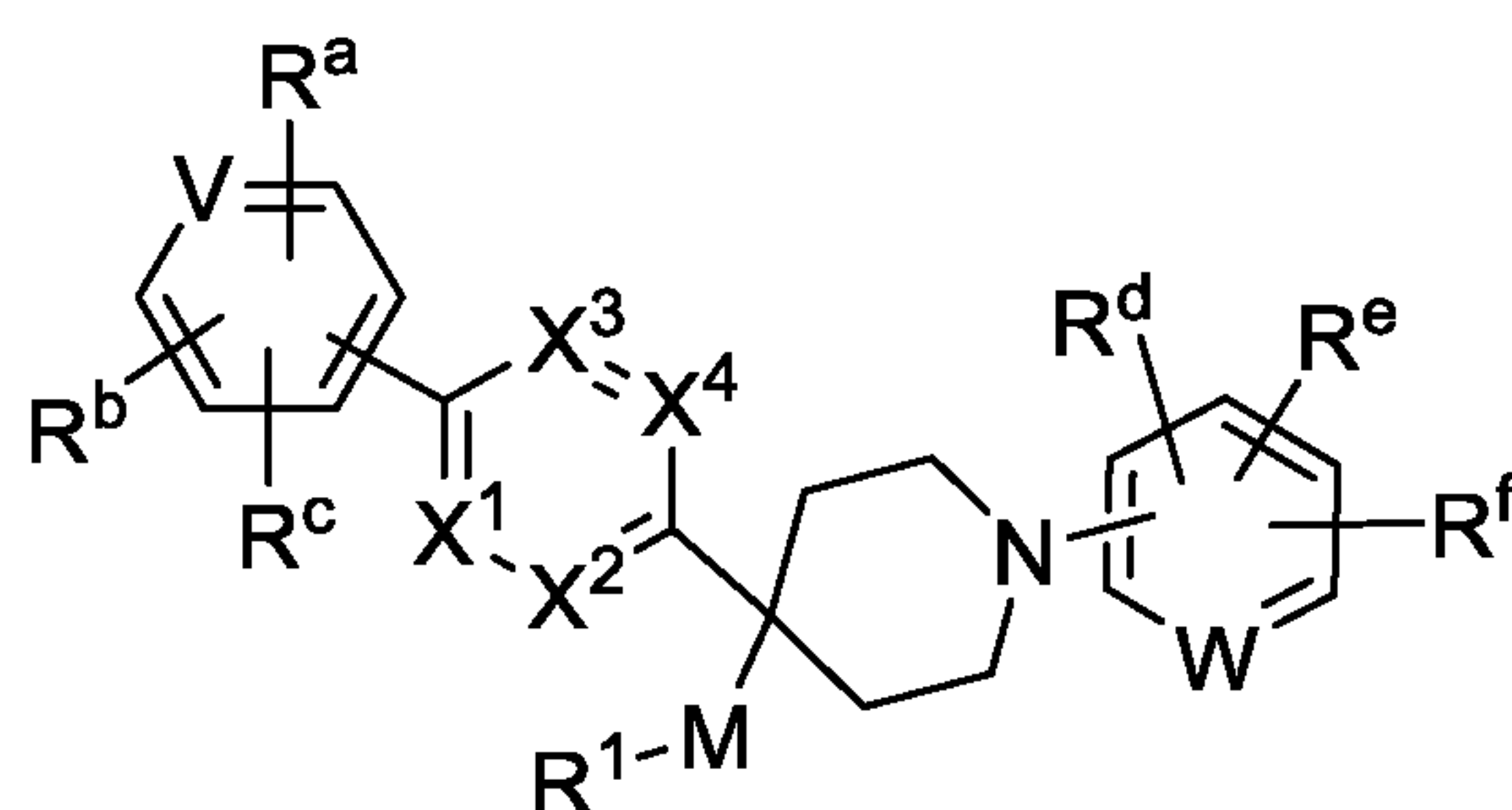
Formula (VI)
