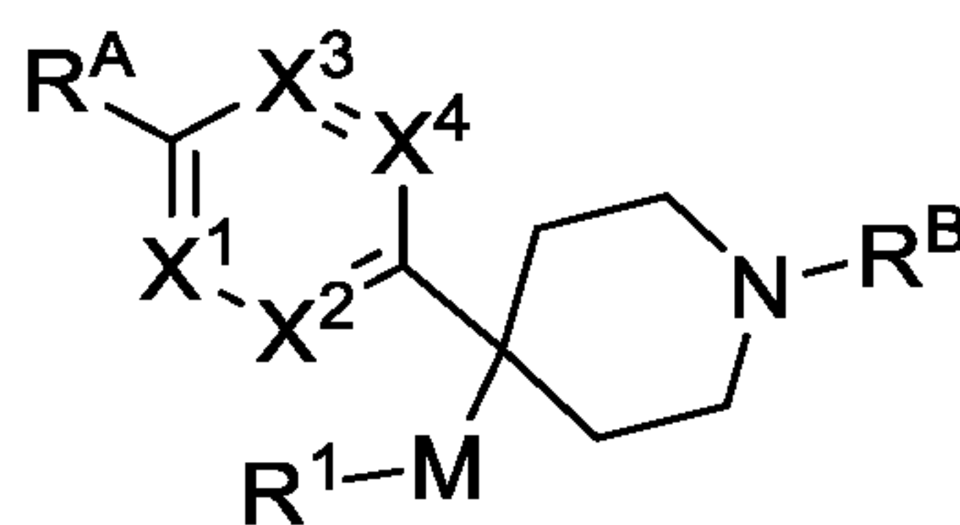
Formula (I)
