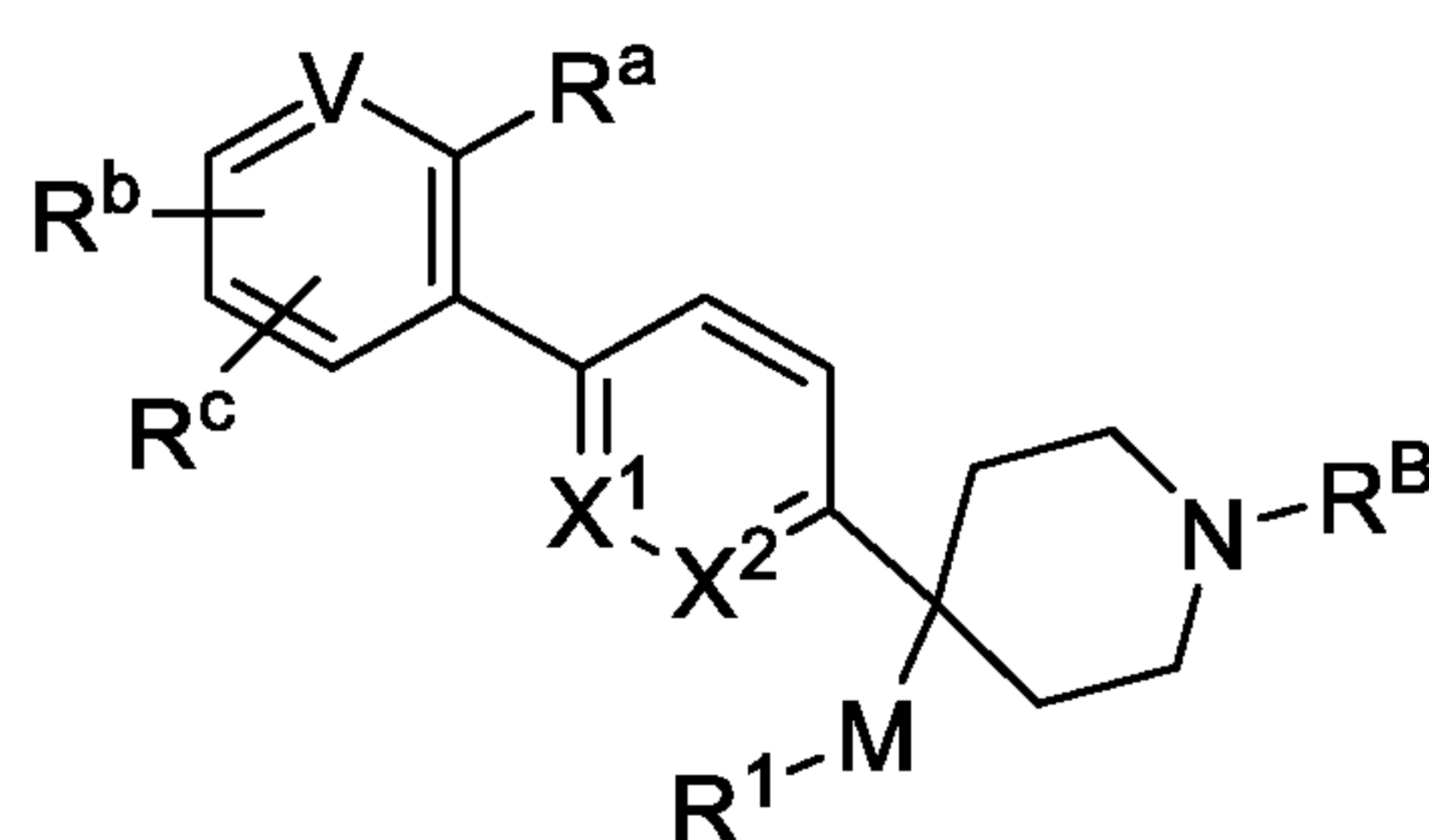
Formula (XI)
