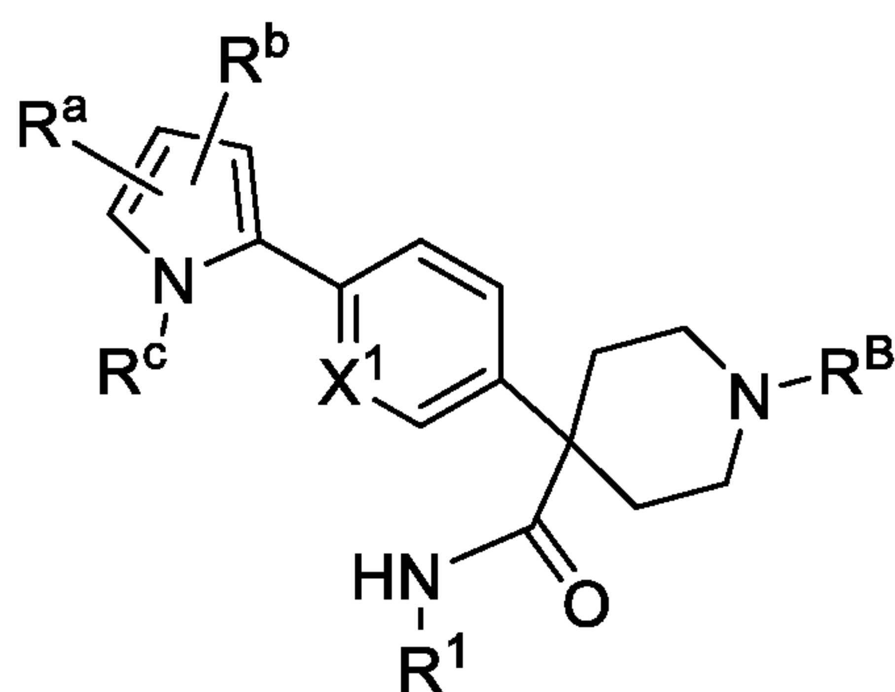
Formula (Xd)
