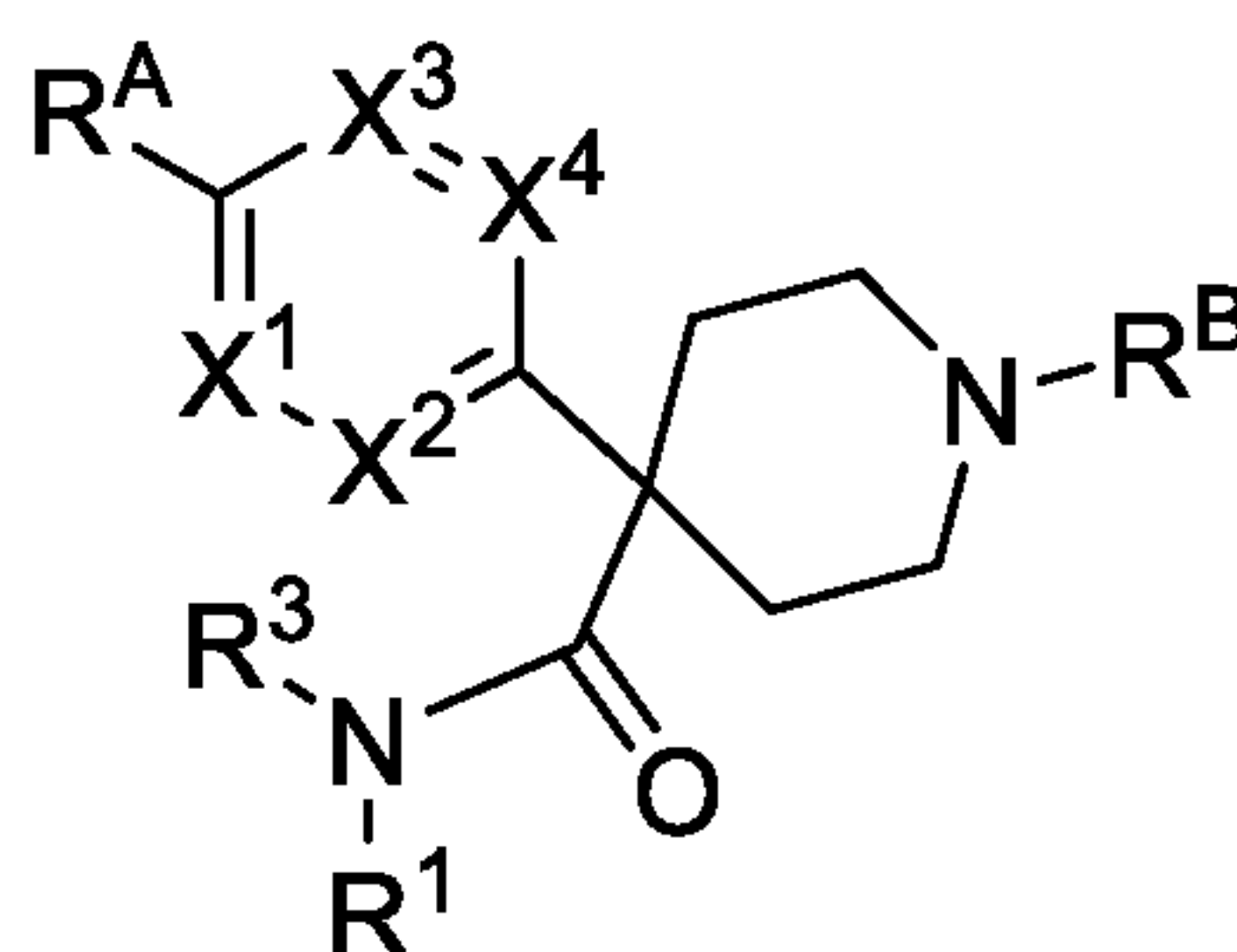
Formula (IIa).
