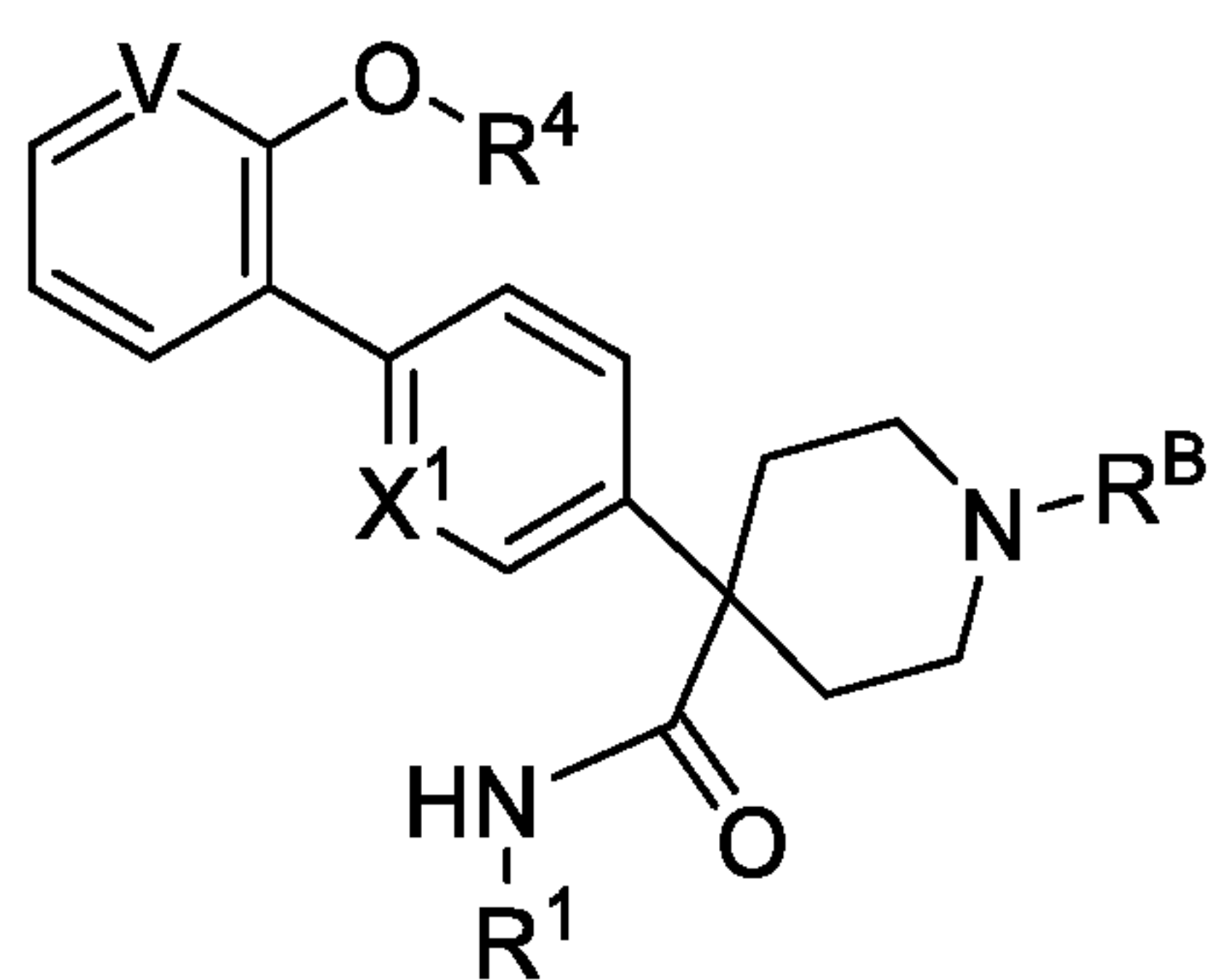
Formula (XIe)
