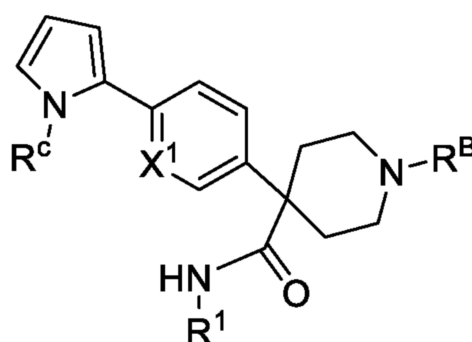
Formula (Xe)
