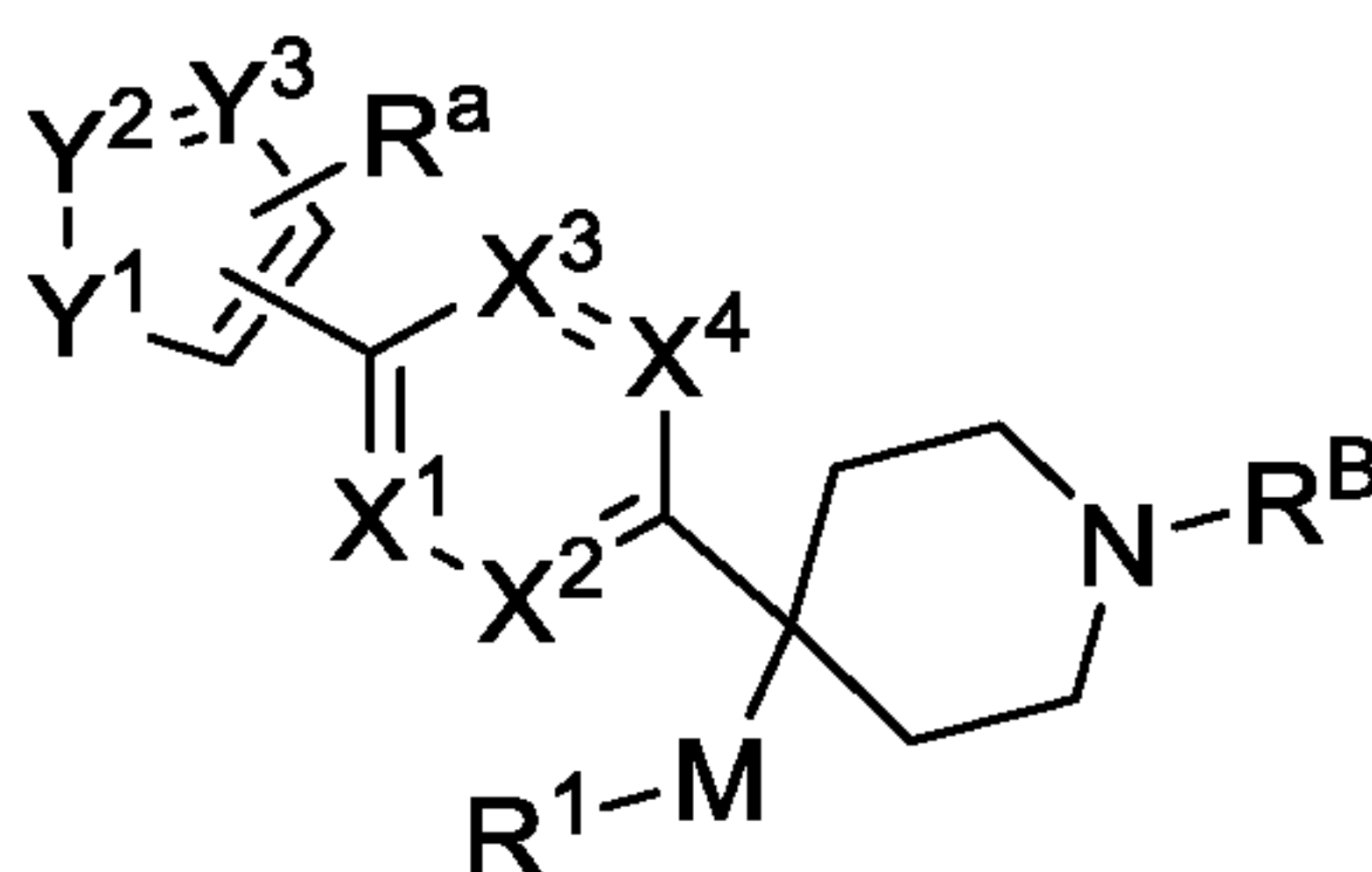
Formula (III)
