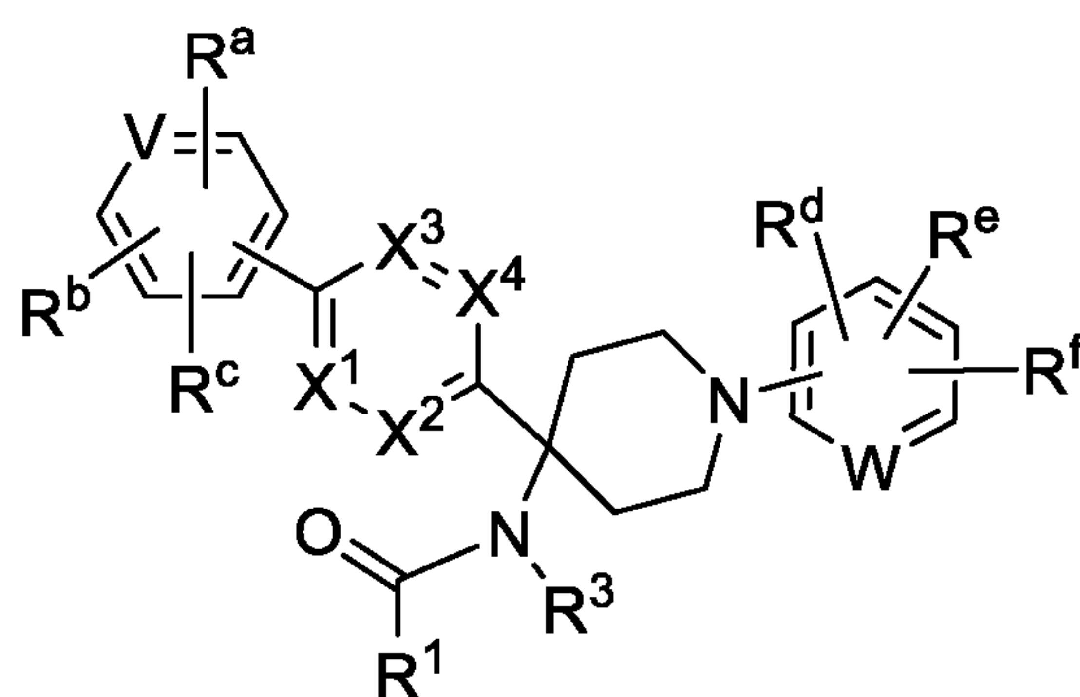
Formula (VIc)
