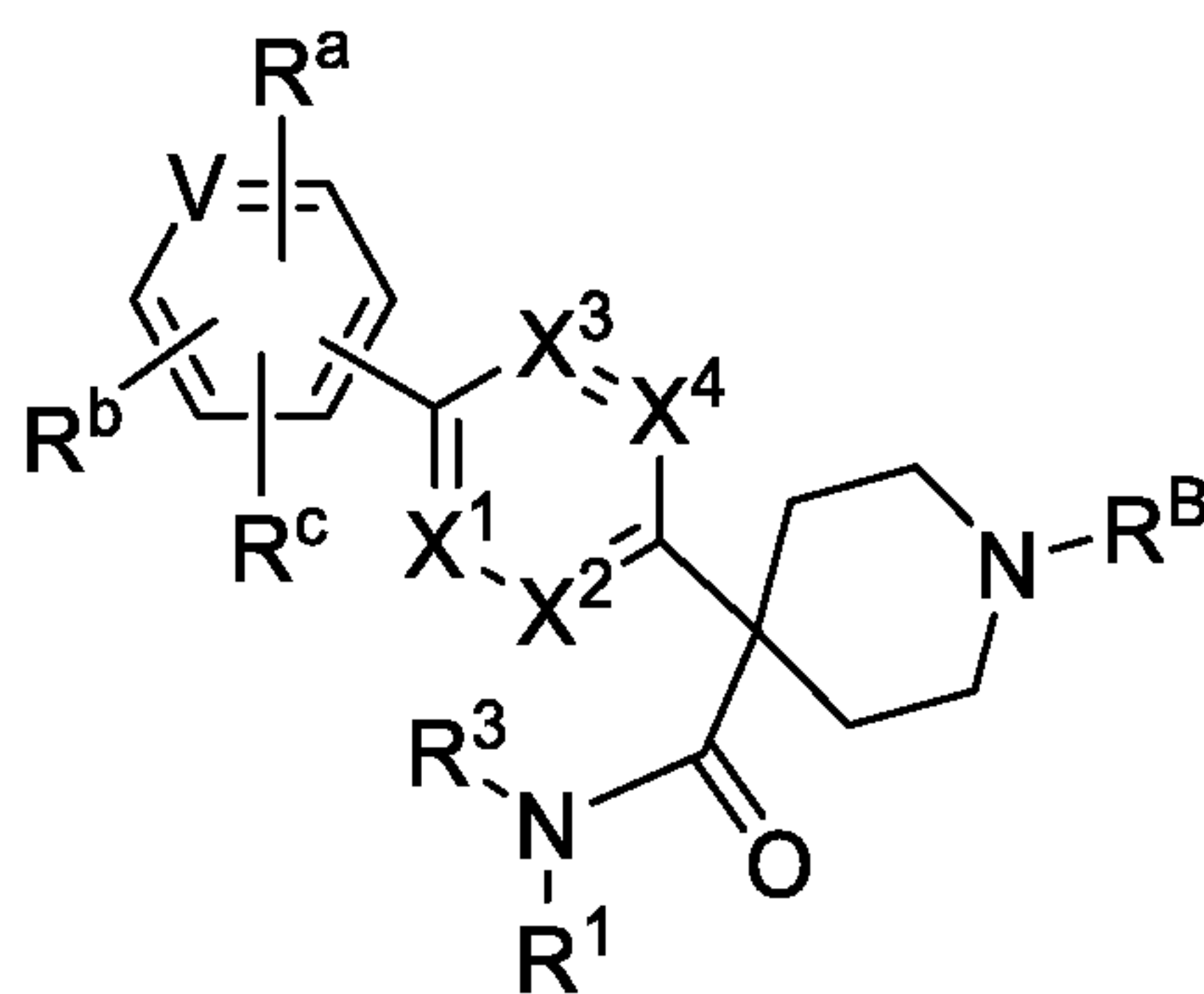
Formula (IVa)
