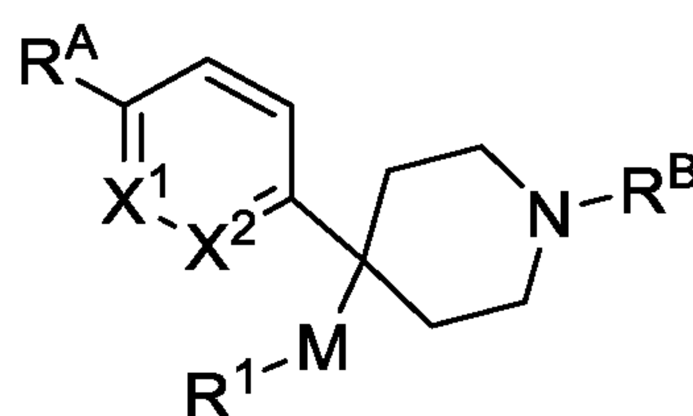
Formula (IX)
