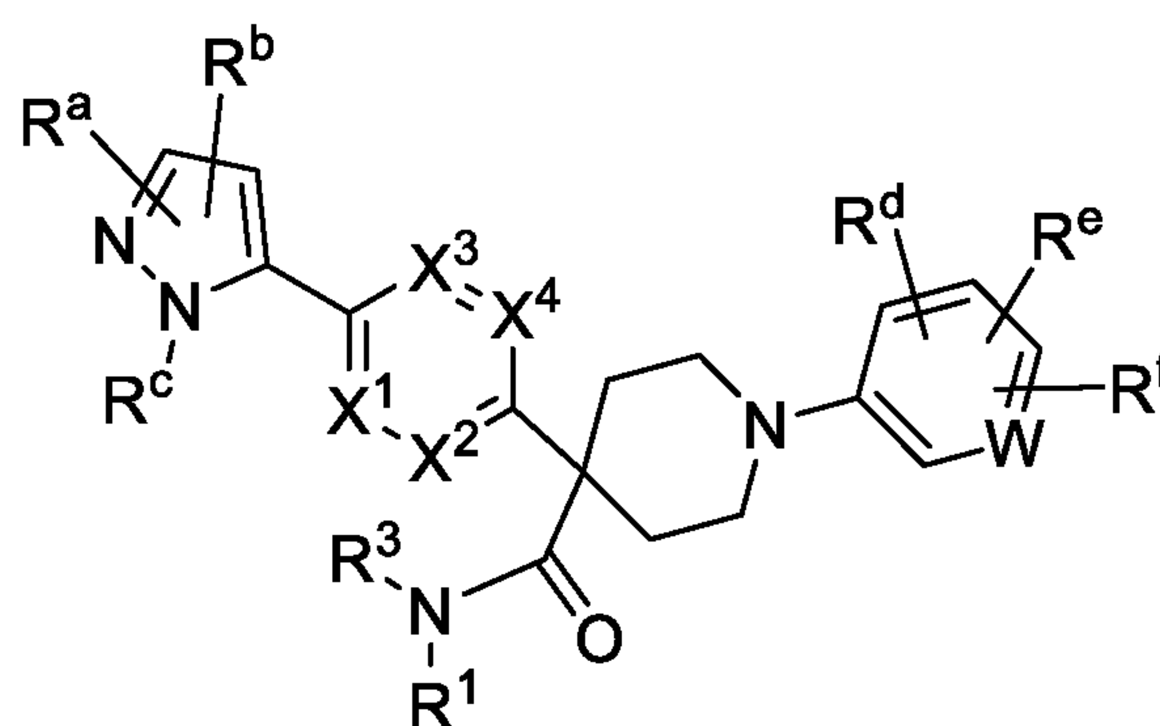
Formula (Vd)
