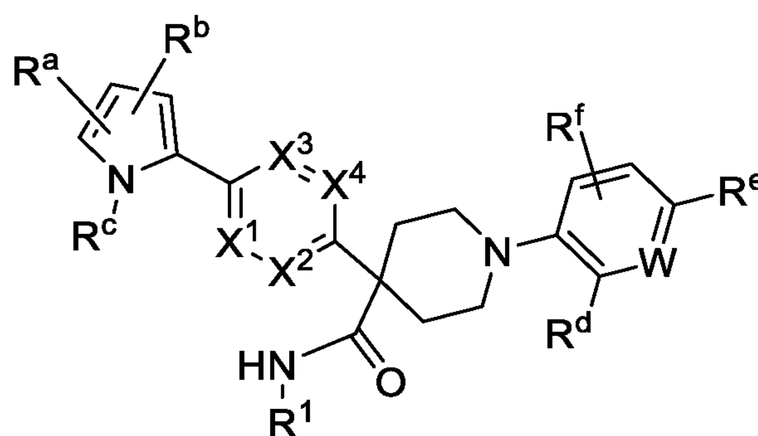
Formula (VIIa)
