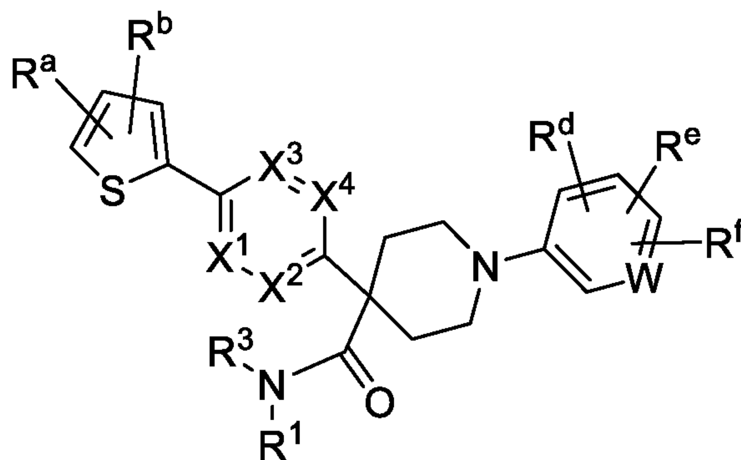
Formula (Vi)
