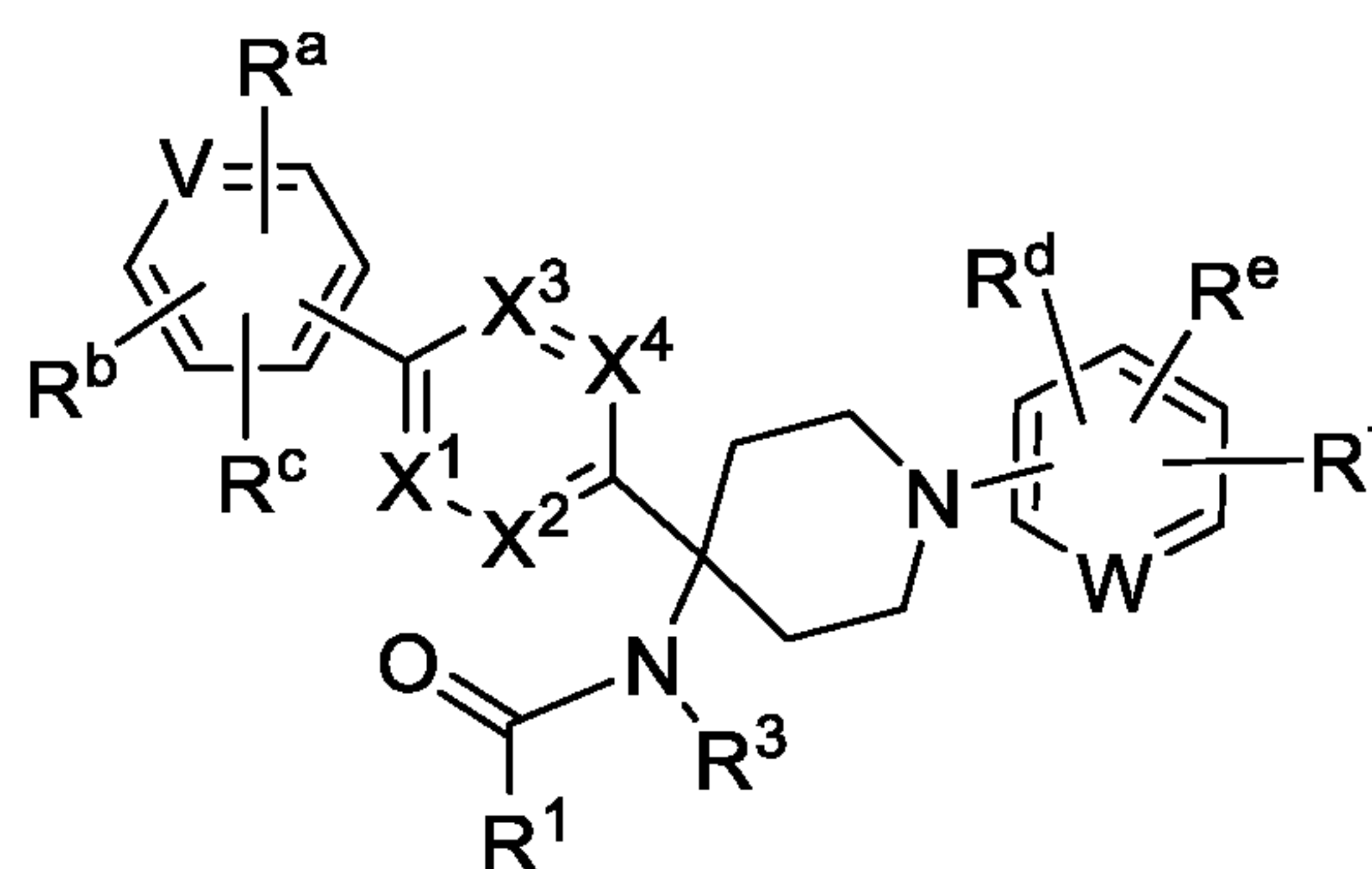
Formula (VIc)
