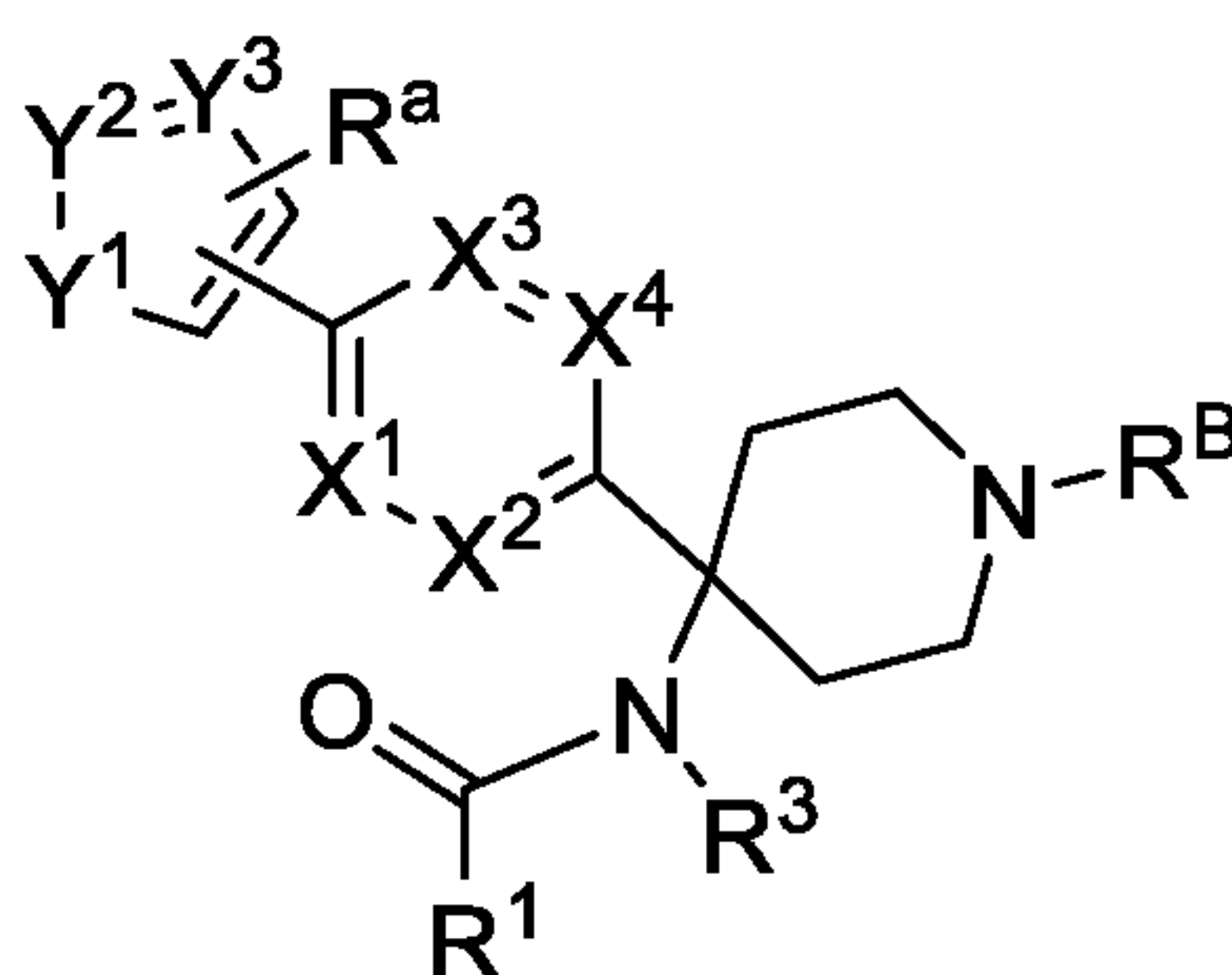
Formula (IIIb)
