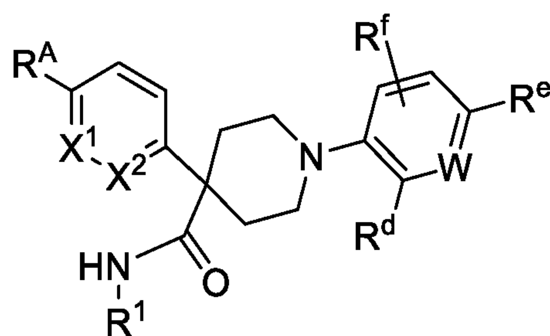
Formula (XIIIa)
