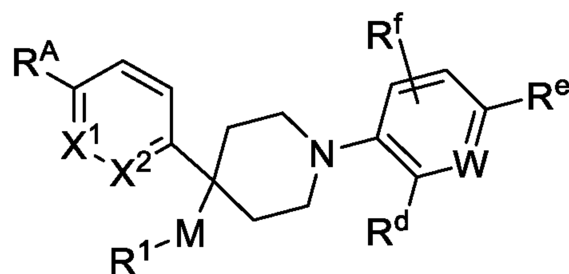
Formula (XIII)
