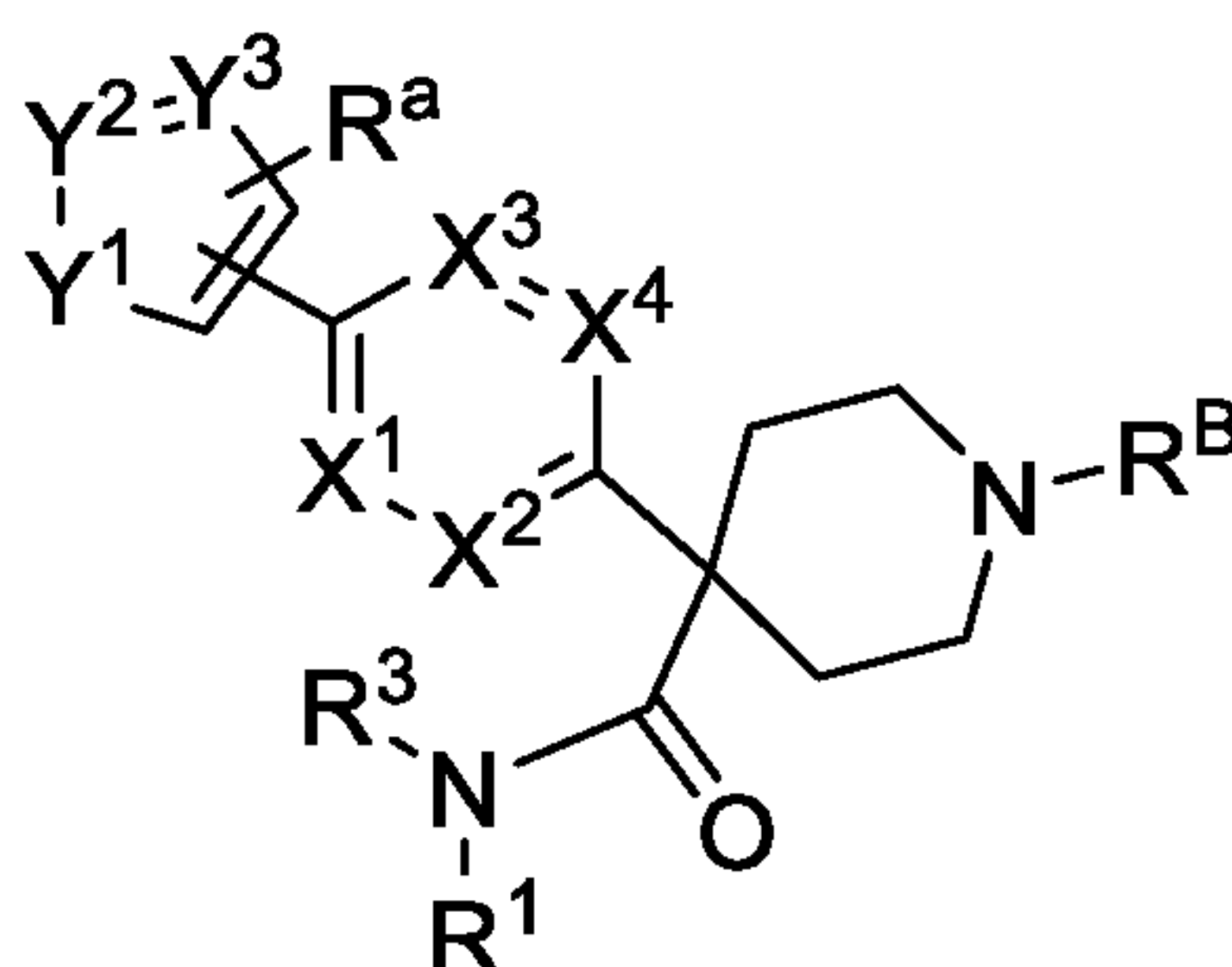
Formula (IIIa)
