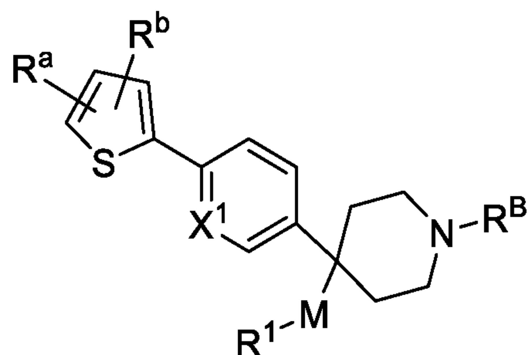
Formula (XIIb).
