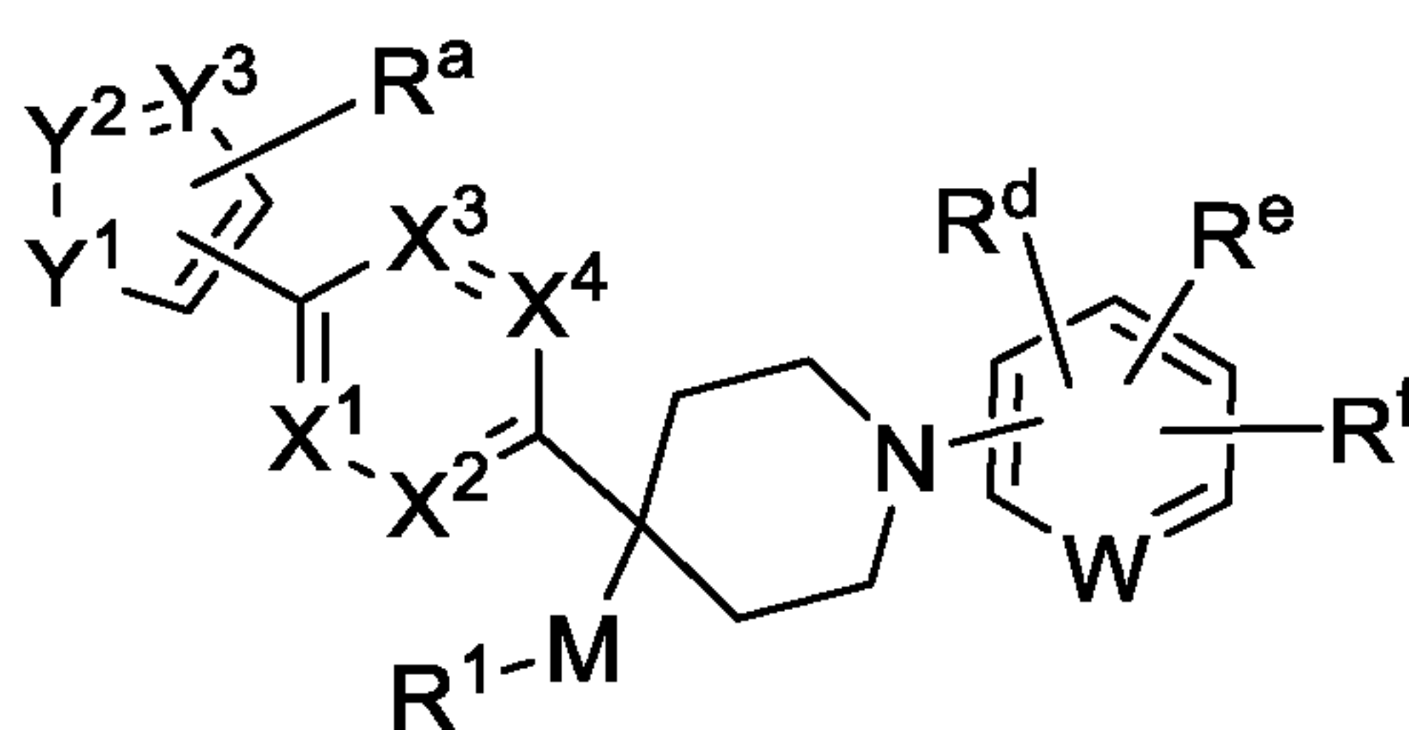
Formula (V)
