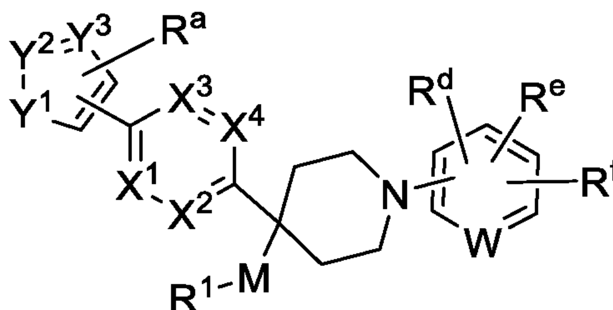
Formula (V)
