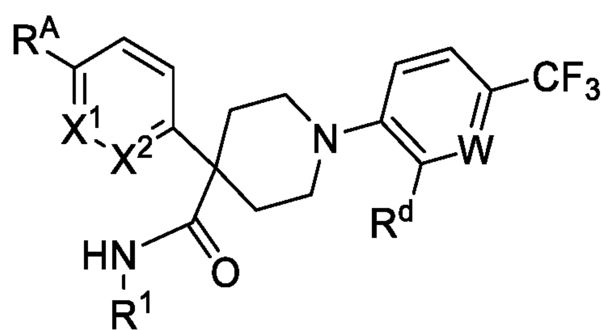
Formula (XIIIb)
