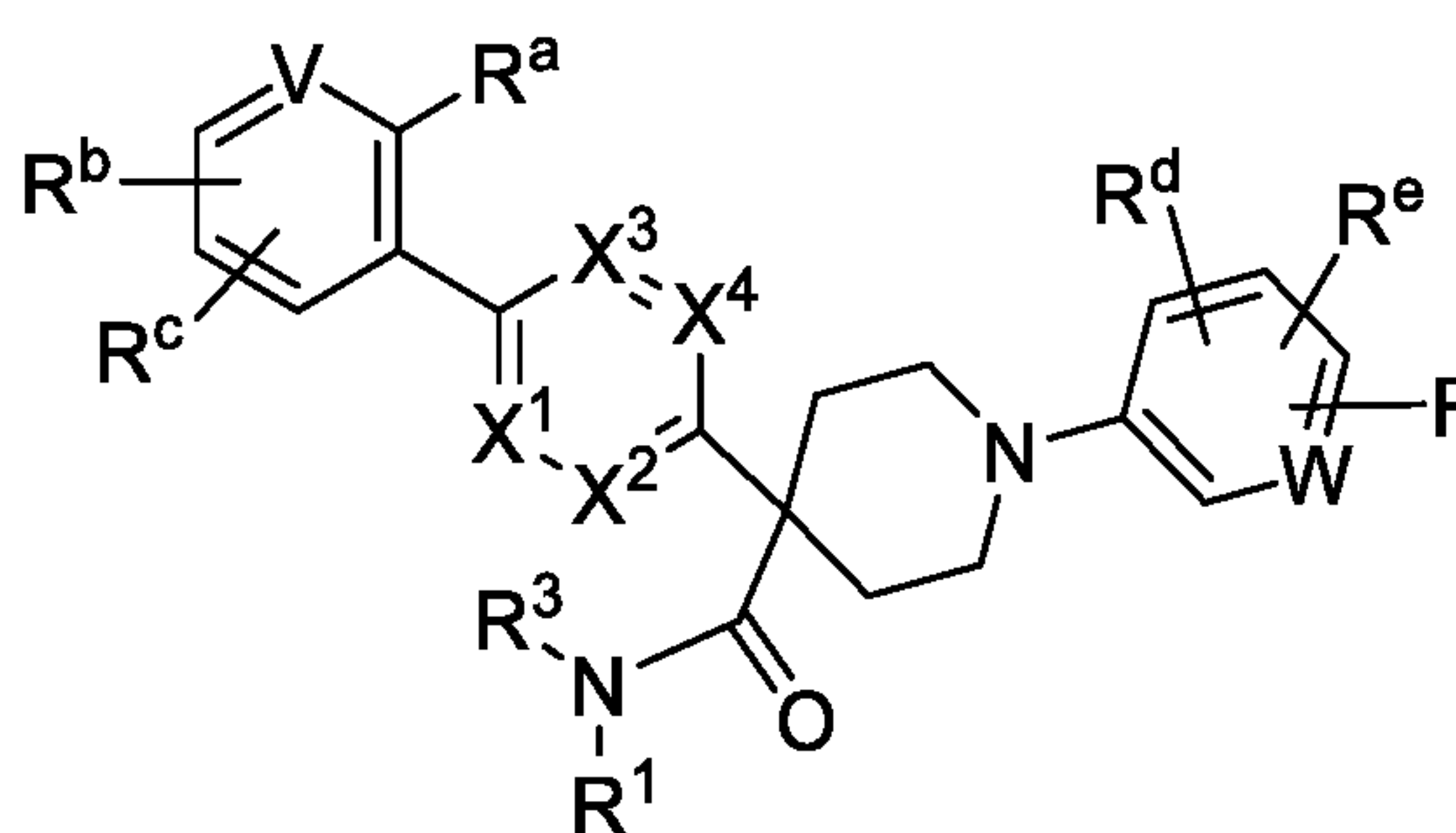
Formula (VIb)
