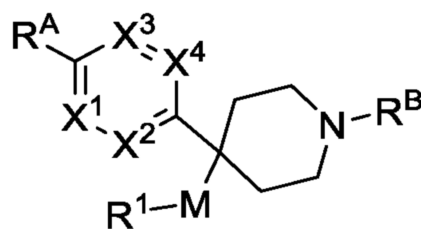
Formula (I)
