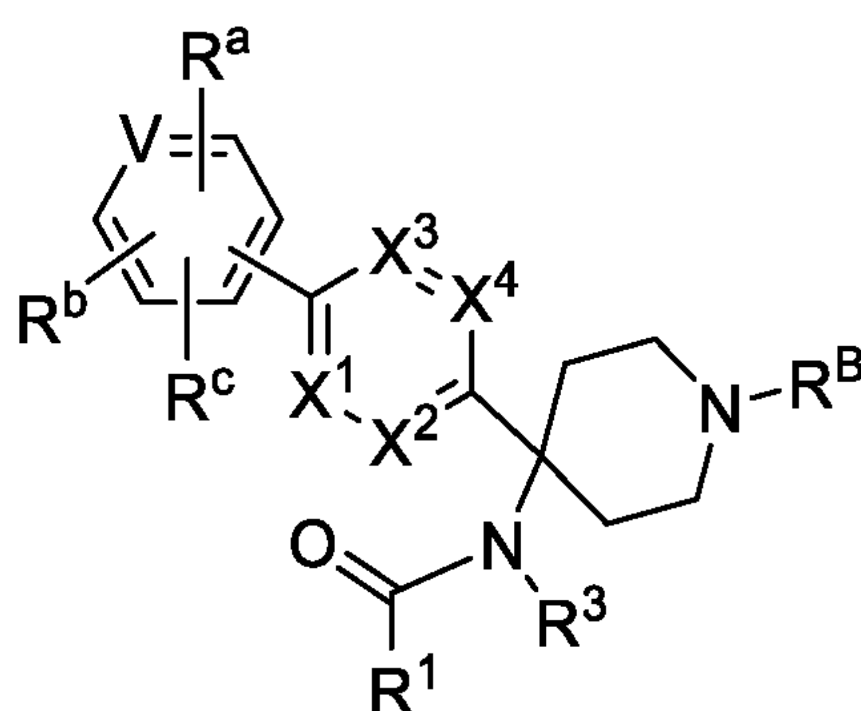
Formula (IVb)
