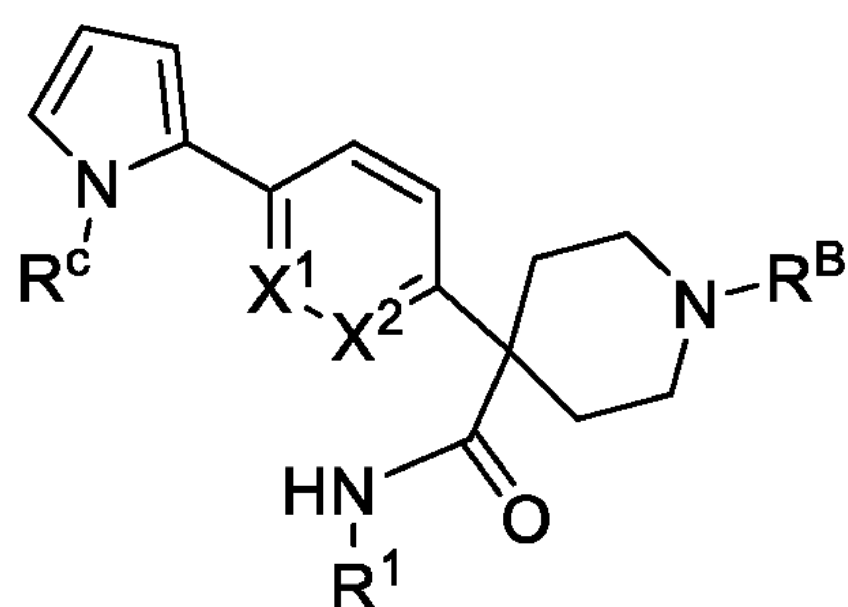
Formula (Xb)
