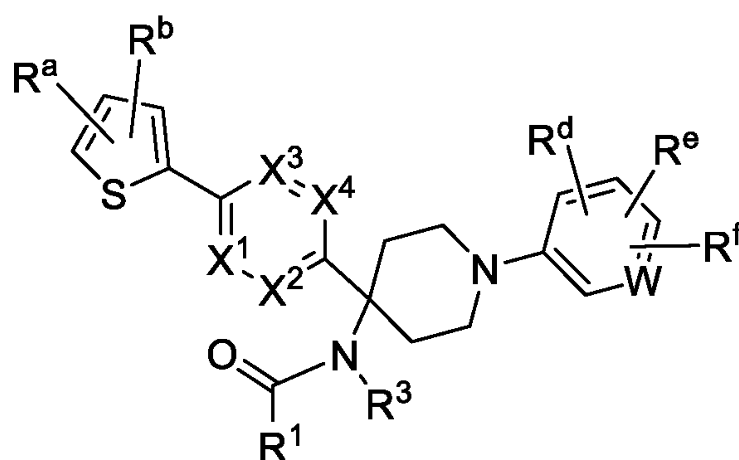
Formula (Vp)
