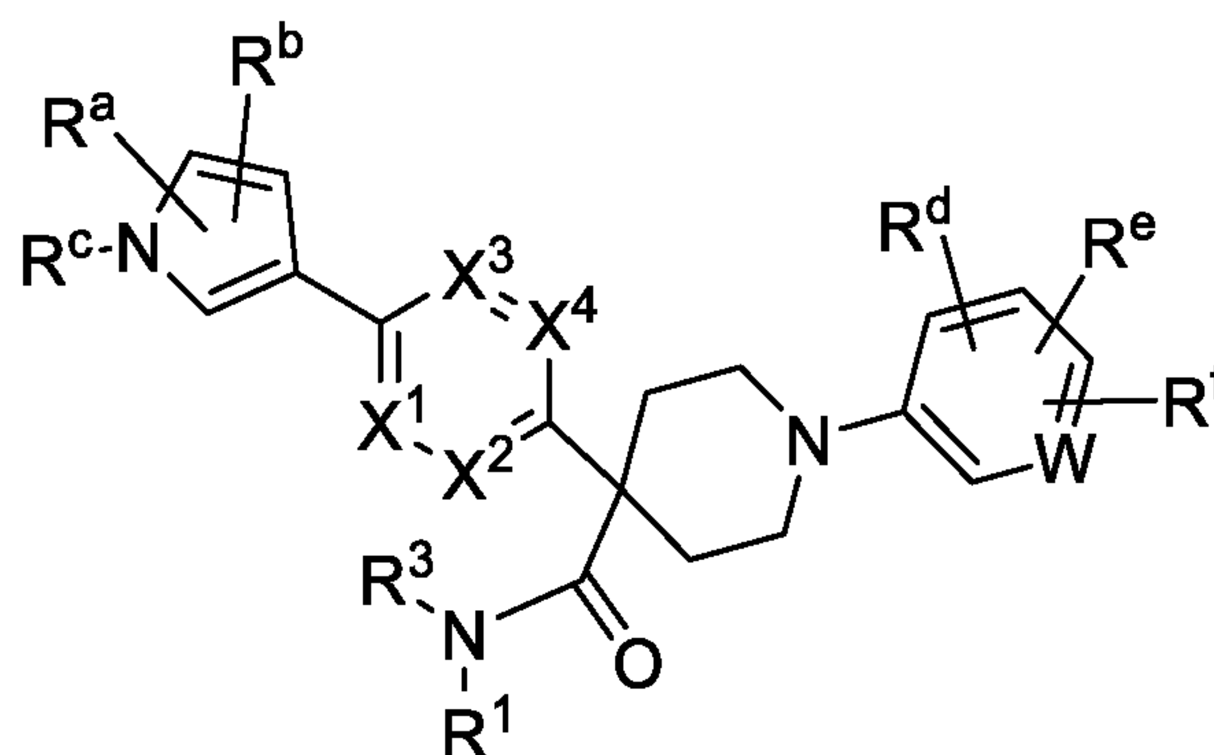
Formula (Vc)
