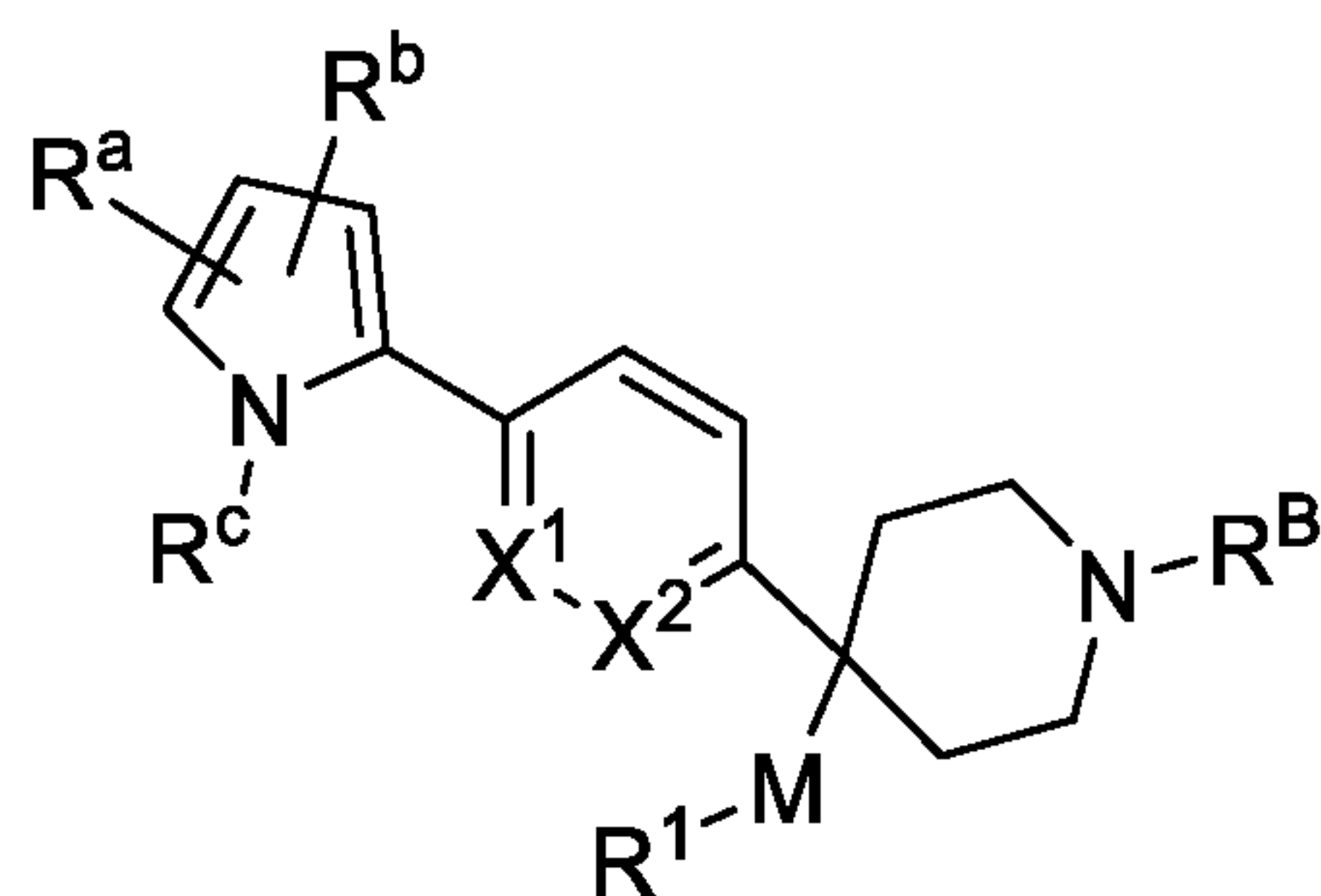
Formula (X)
