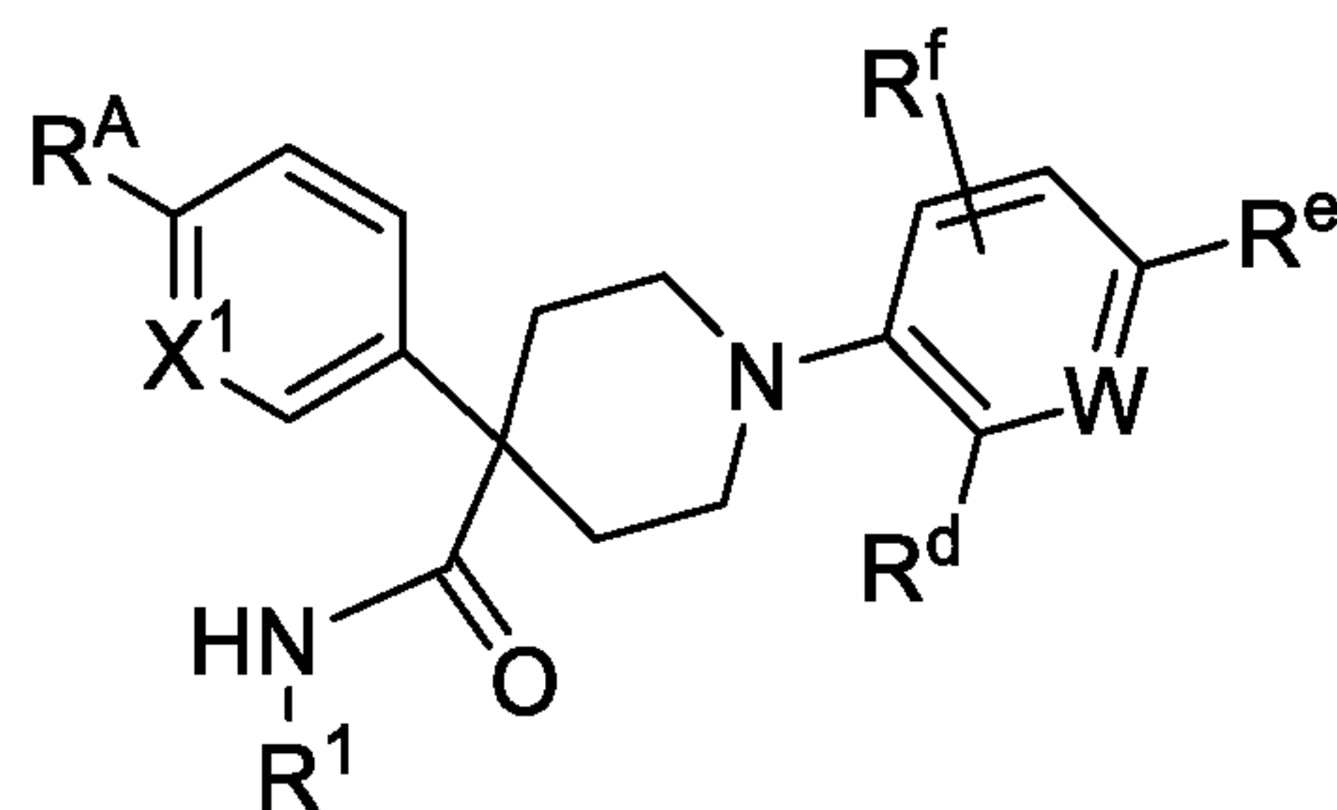
Formula (XIIId)
