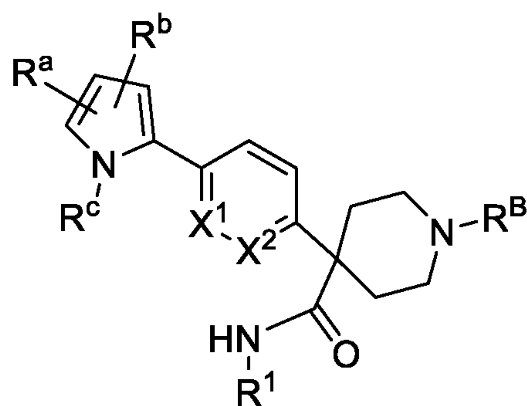
Formula (Xa)
