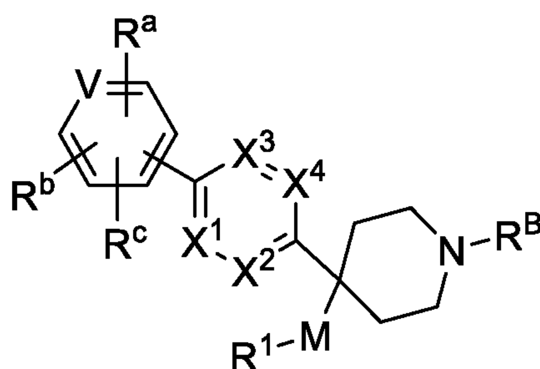
Formula (IV)
