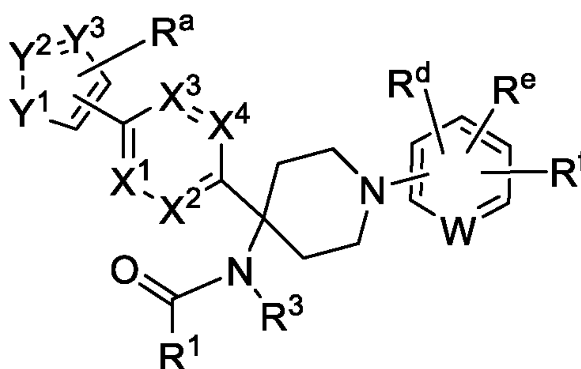
Formula (Vj)
