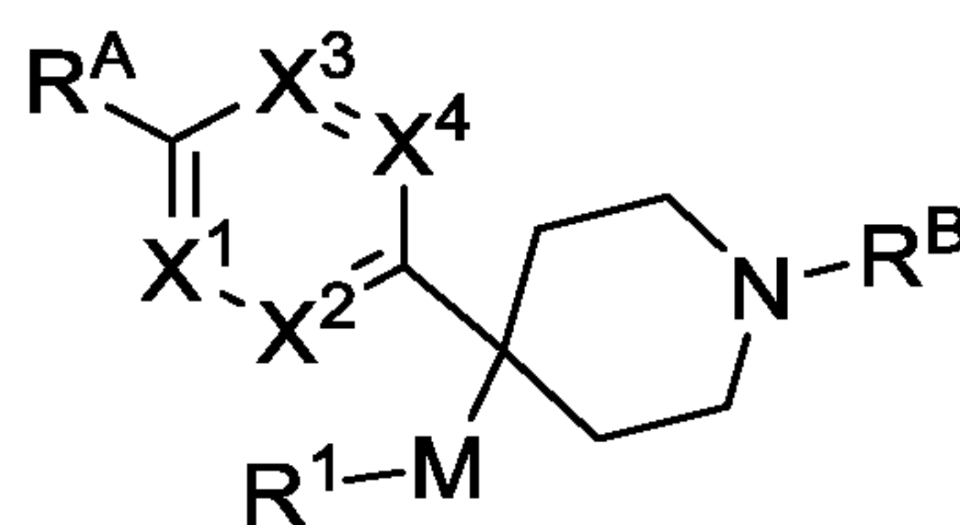
Formula (VIII)
