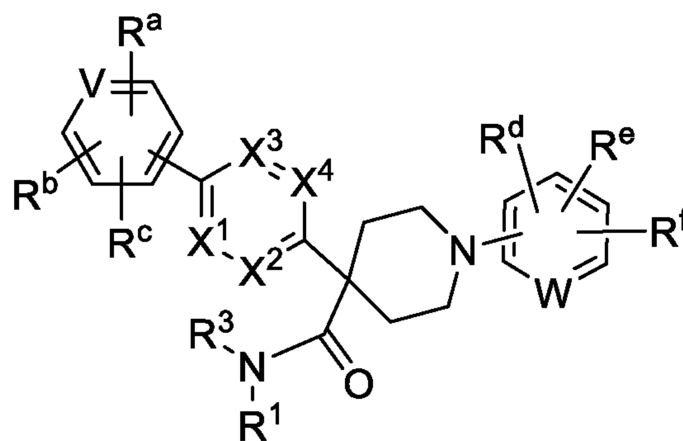
Formula (VIa)
