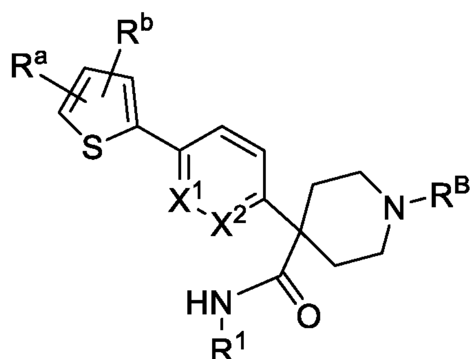
Formula (XIIa)
