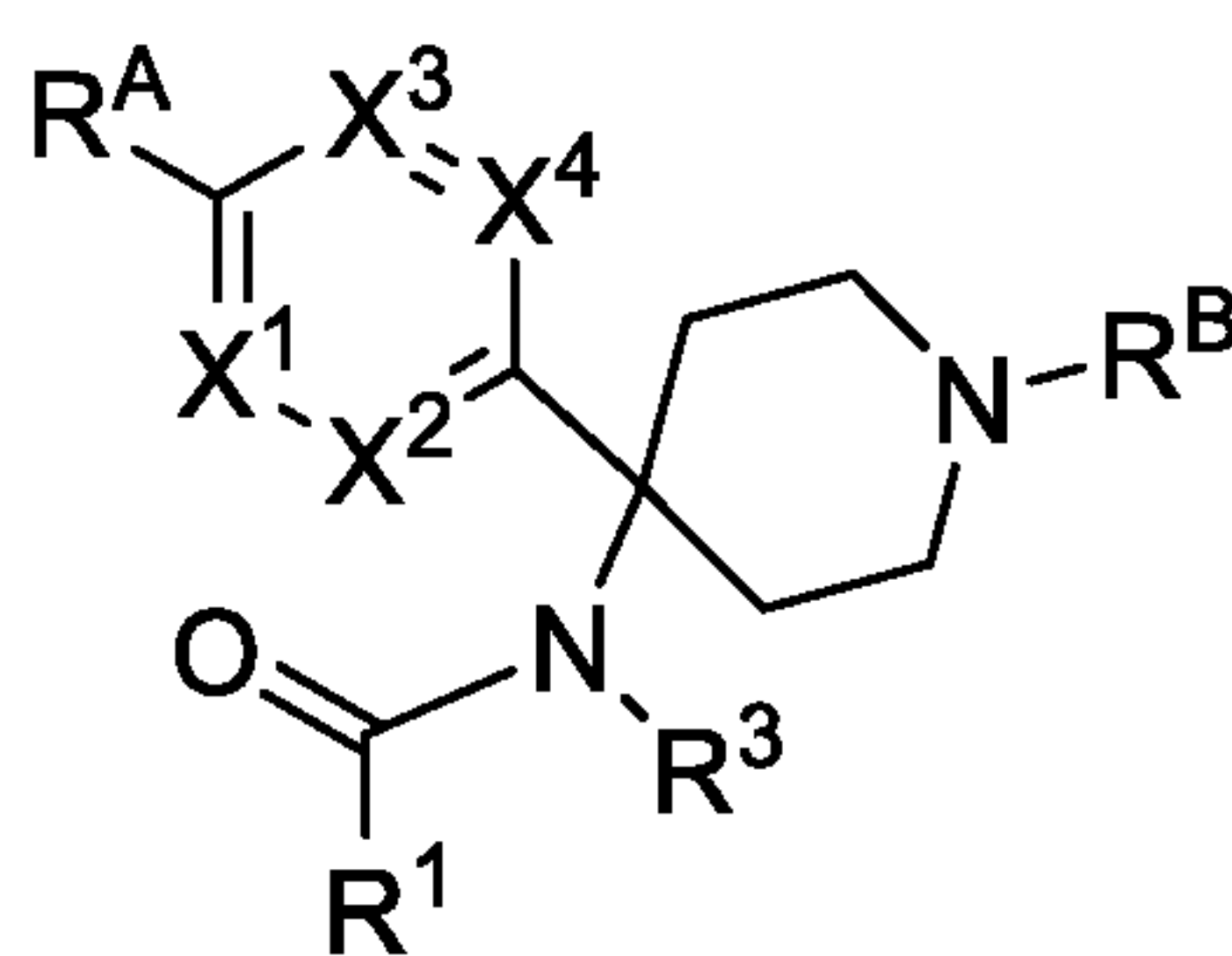
Formula (IIb).
