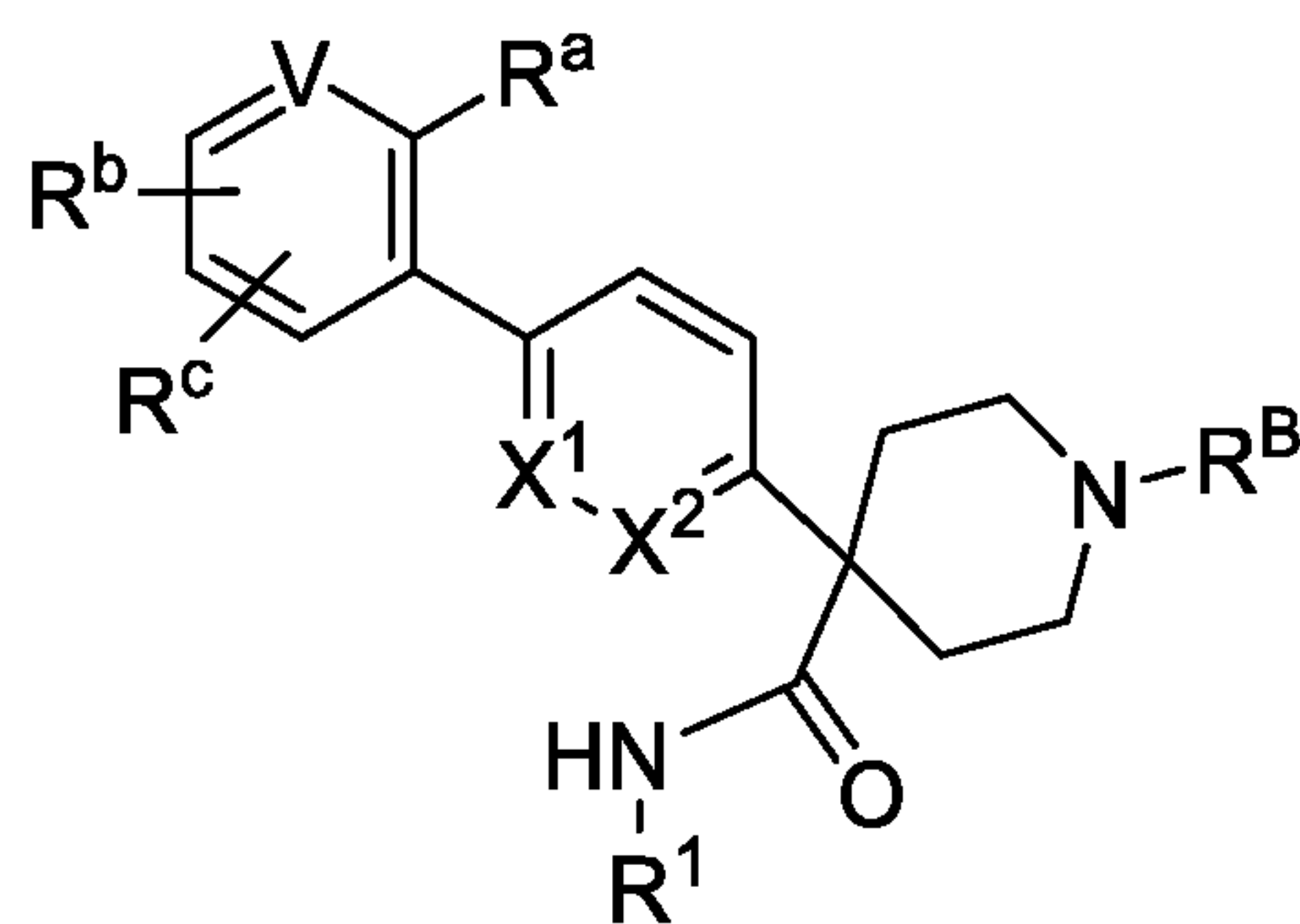
Formula (XIa)
