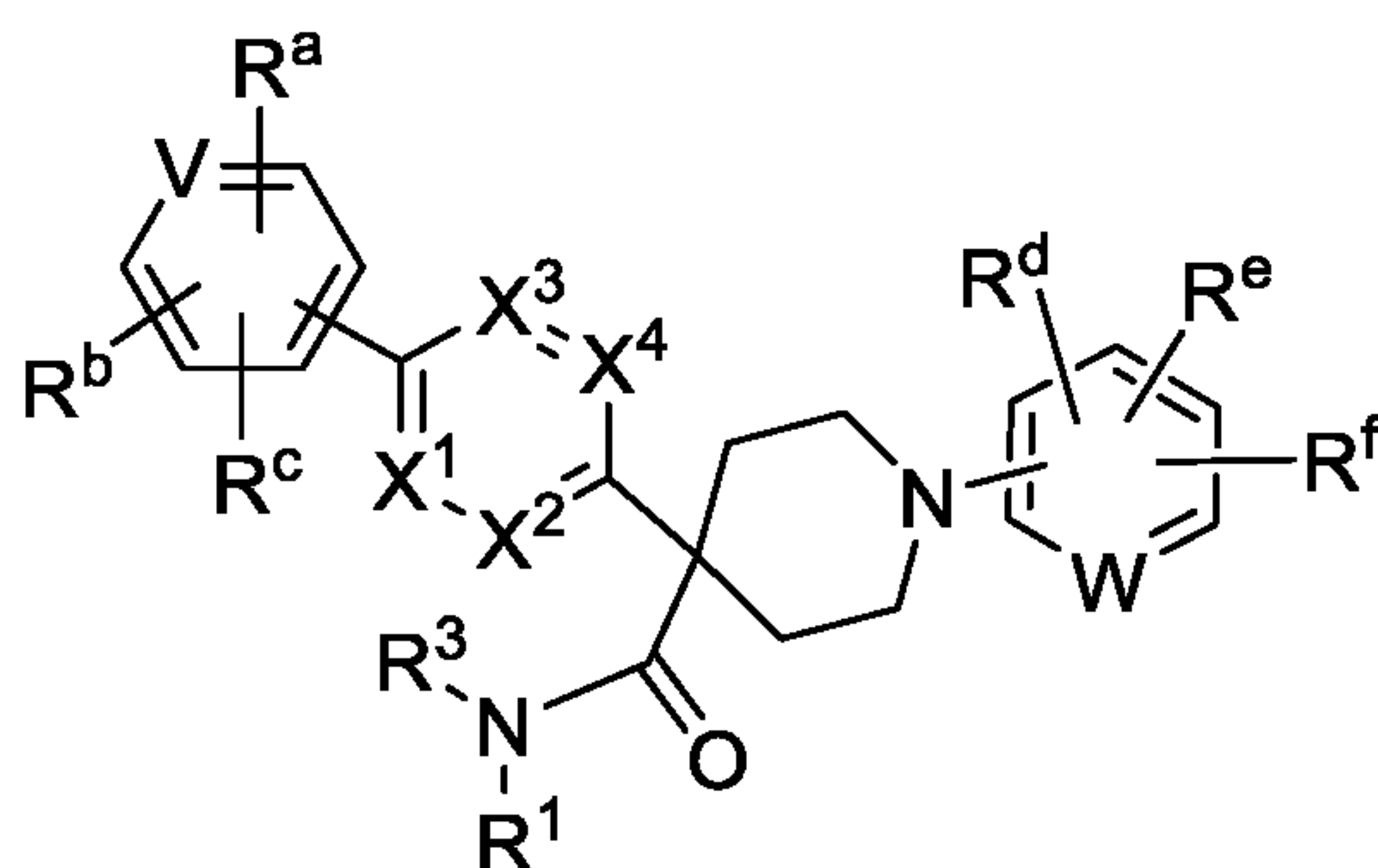
Formula (VIa)
