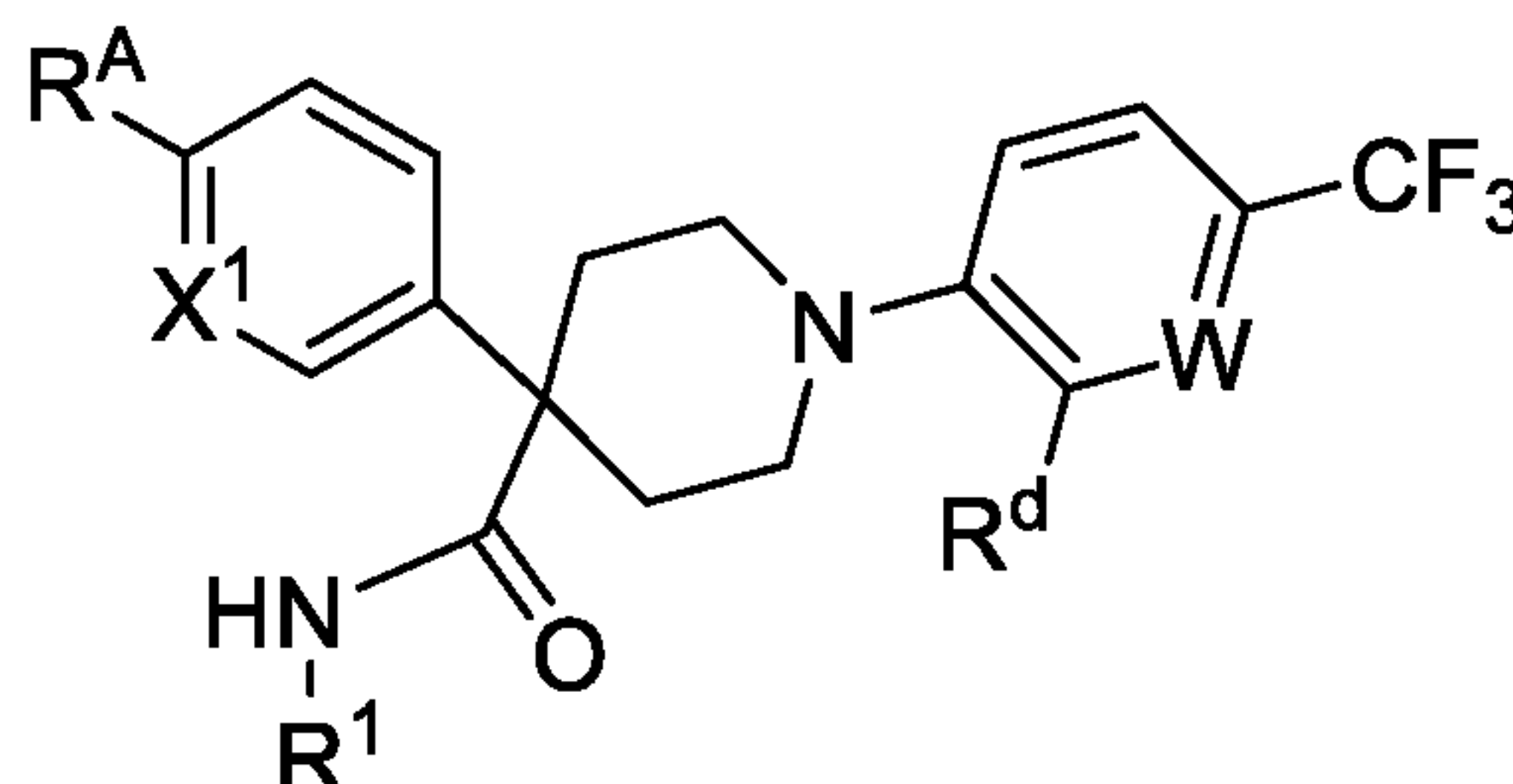
Formula (XIIIe)
