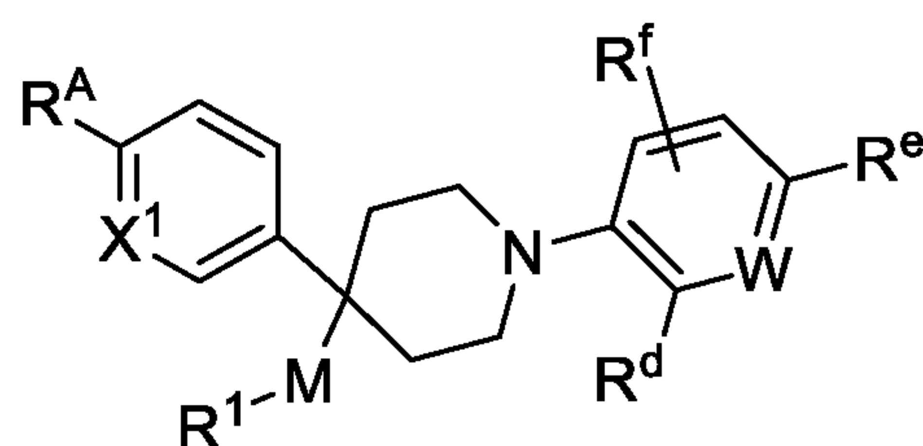
Formula (XIIIc)
