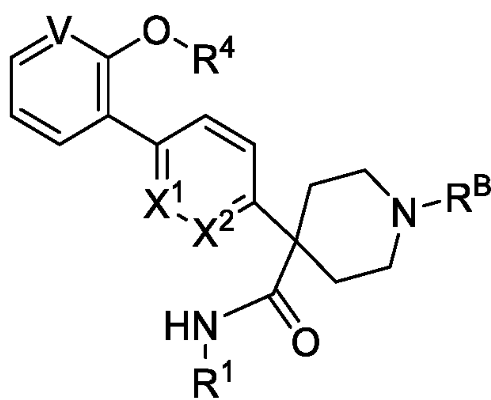
Formula (XIb)
