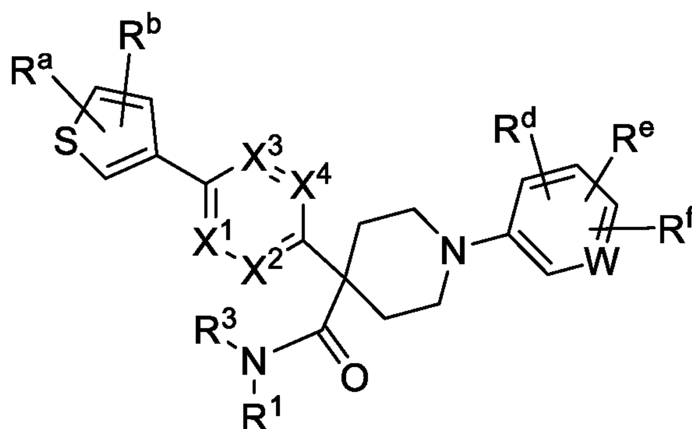
Formula (Vh)
