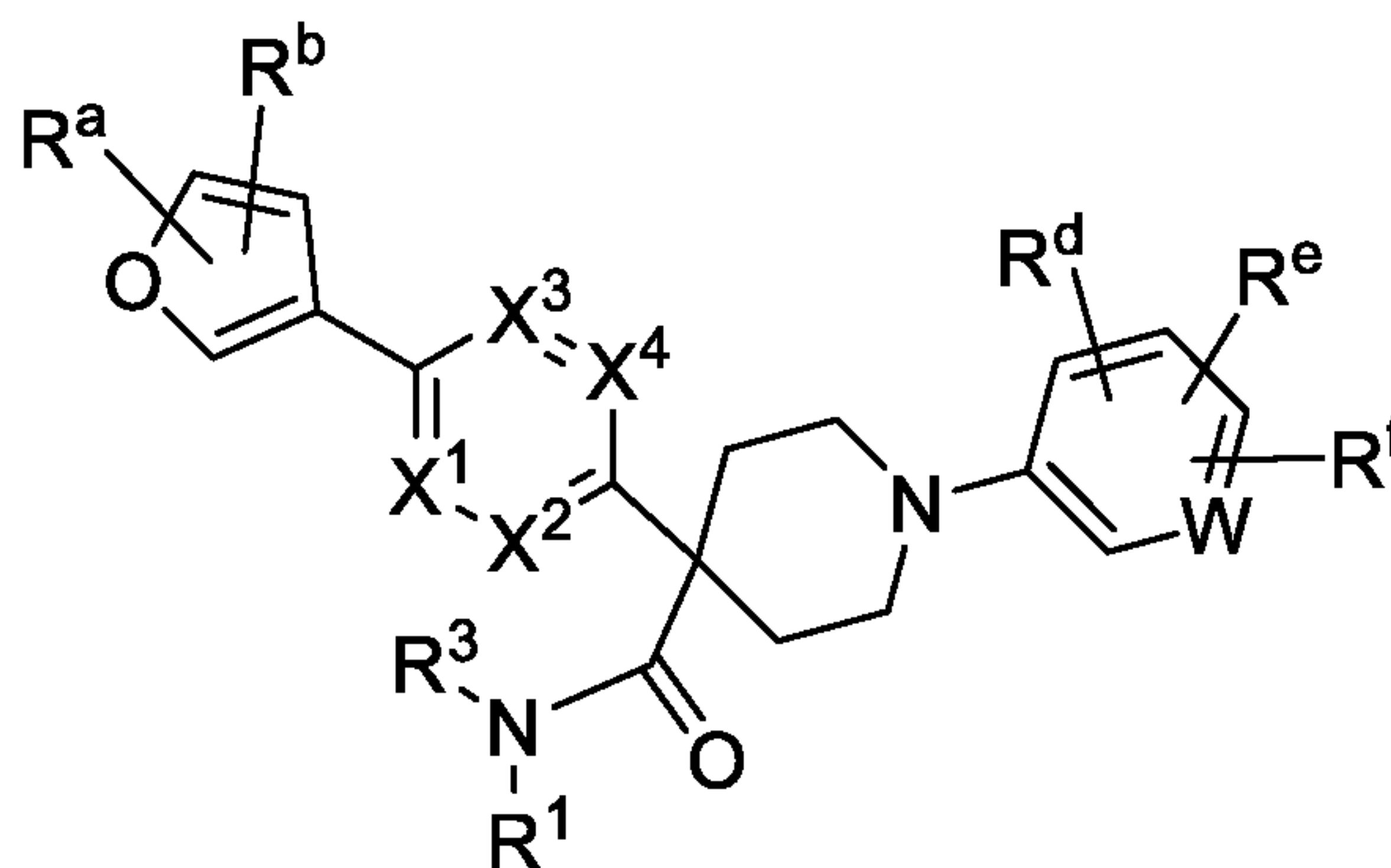
Formula (Vg)
