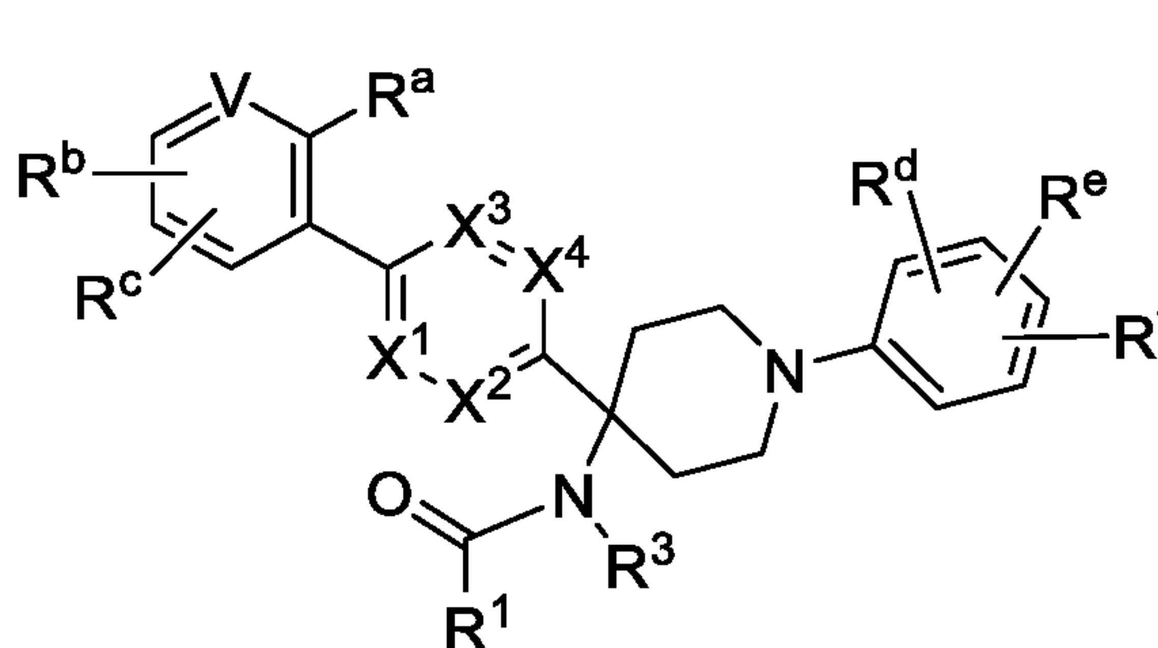
Formula (VIe)
