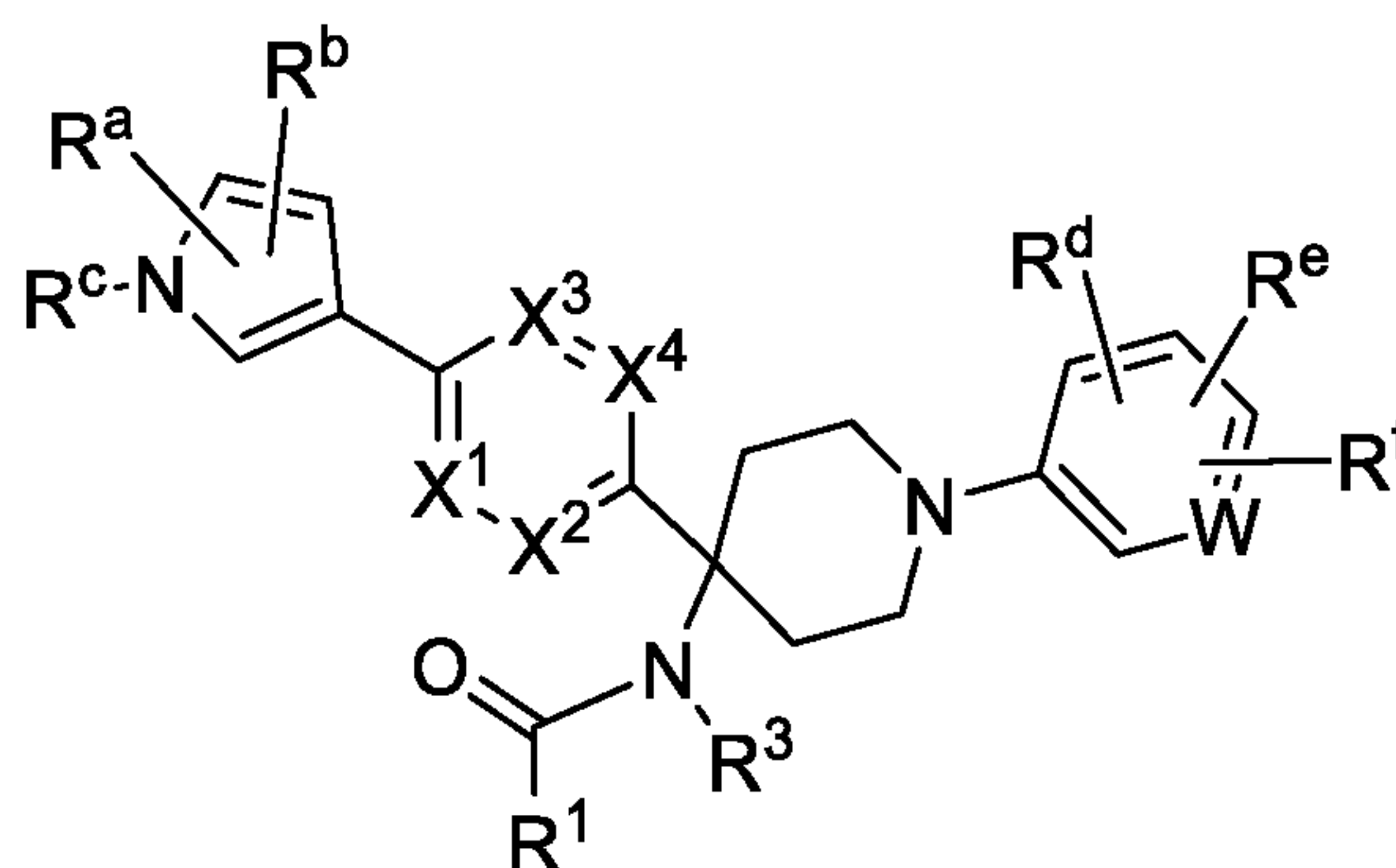
Formula (VI)
