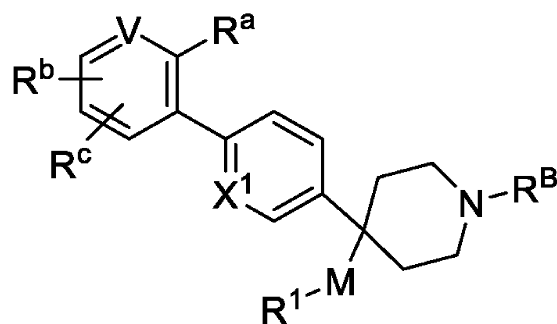
Formula (XIc)
