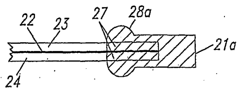
FIG. 3A (Prior Art)
