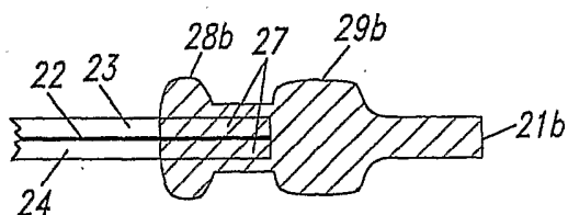
FIG. 3B (Prior Art)
