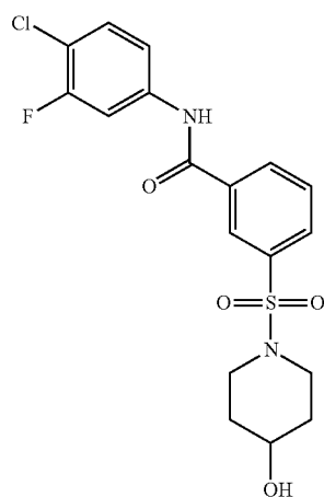
413/415 GA A10B01C83 1 H NMR (400 MHz, DMSO-d 6 ) δ 10.79(s, 1H), 8.27(d, 1H), 7.95 (m, 2 H), 7.83 (m, 1H), 7.59 (d, 2H), 3.16(d, 2H), 2.77 (m, 2H), 1.73(m, 2H), 1.43(m, 2H), 1.17(m, 1H)
