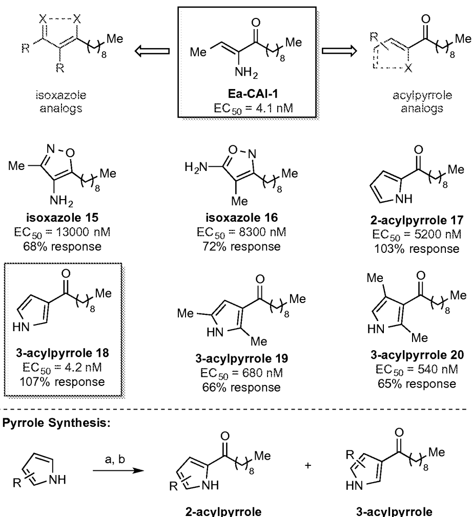
Scheme 2. Variation of the Ea-CAI-1 head group: isoxazole and acylpyrrole analogs. Reagents and conditions: (a) MeMgBr, Et 2 O; (b) n -C 9 H 19 COCl.
