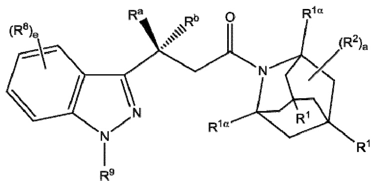
Formula (IVc)
