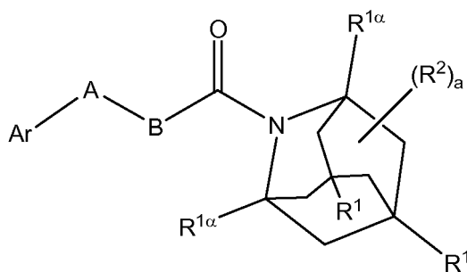
Formel (I)
