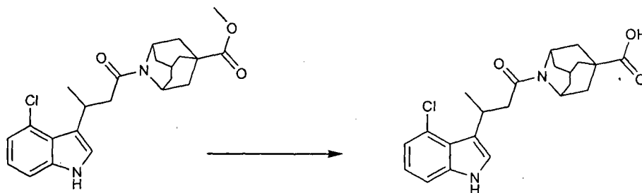
Intermediate 45
