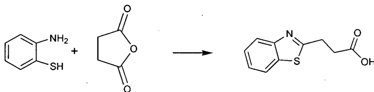
Starting material 6
