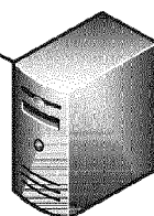
Scheduling Platform
