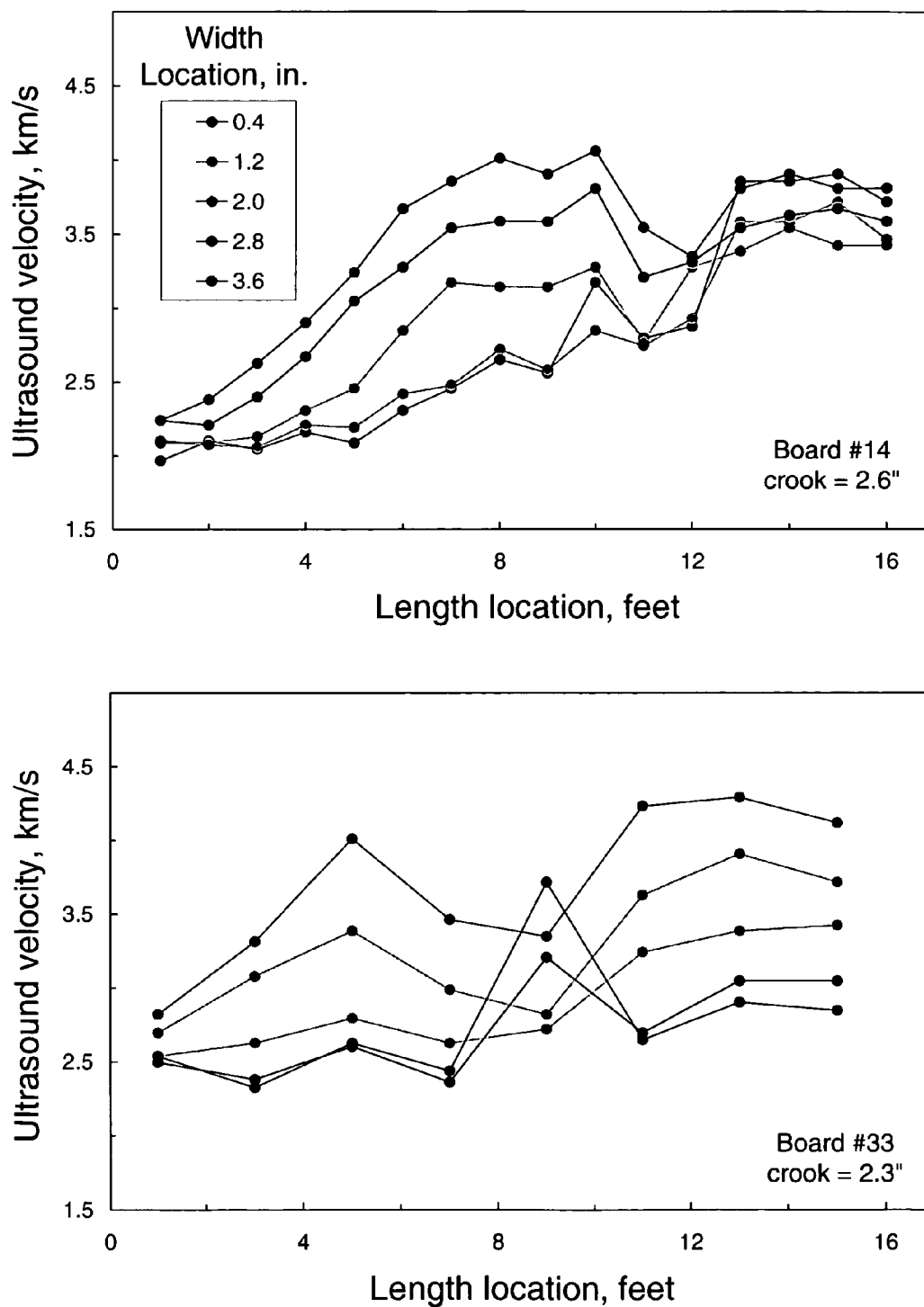
Figure 5. Typical patterns of sound velocity variation in crook-prone lumber. (16-ft. 2x4's from the Wright City mill)
