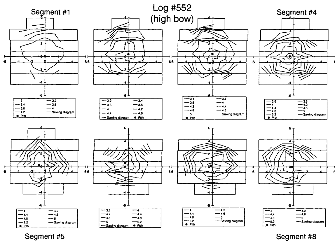
Figure 14. Sound velocity maps for 24-inch-long segments from log #552.
