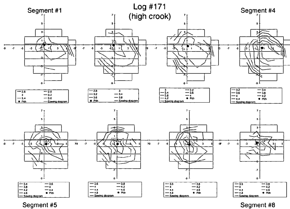
Figure 11. Sound velocity maps for 24-inch-long segments from log #171.
