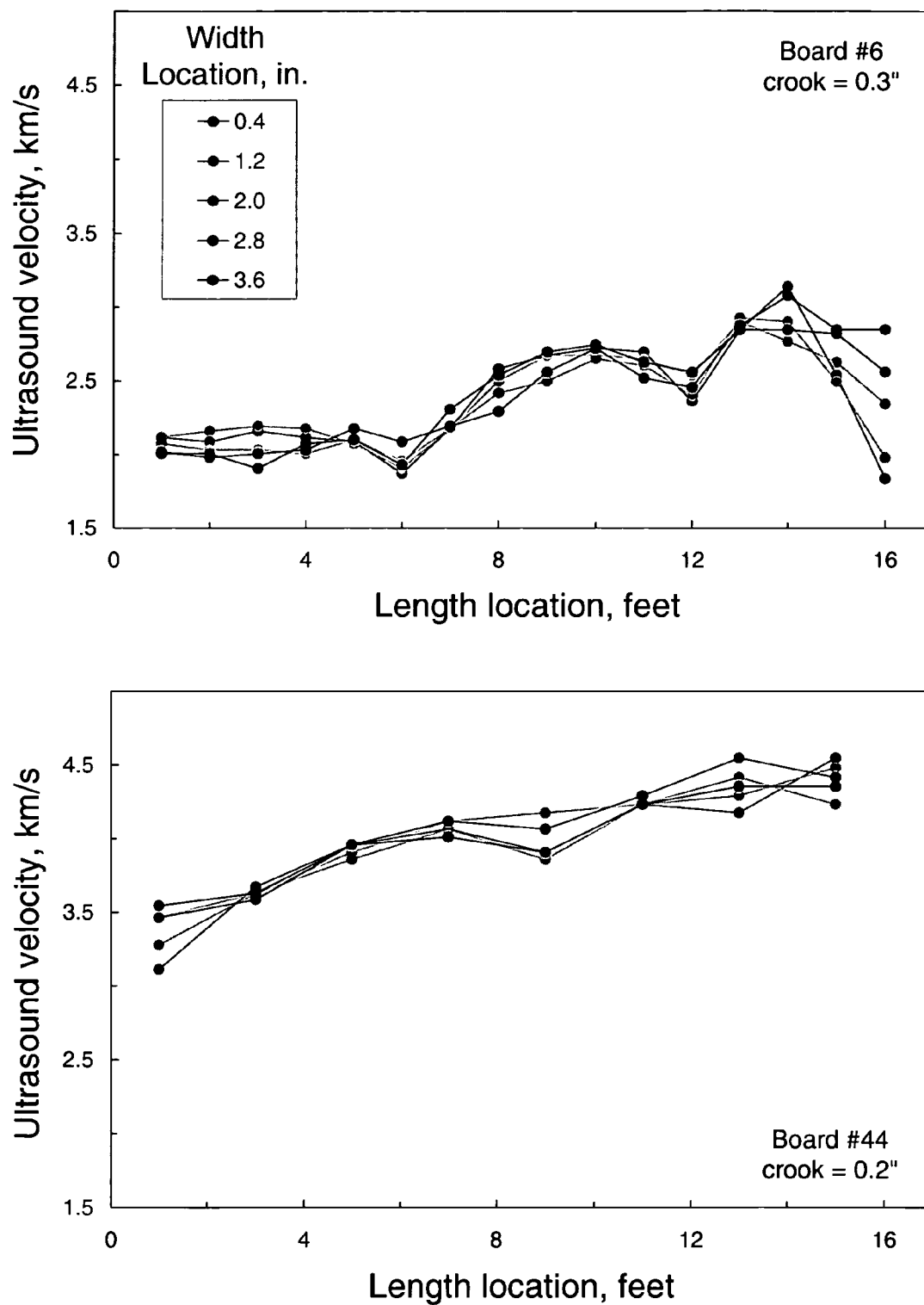
Figure 6. Typical patterns of sound velocity variation in straight lumber. (16-ft. 2x4's from the Wright City mill)
