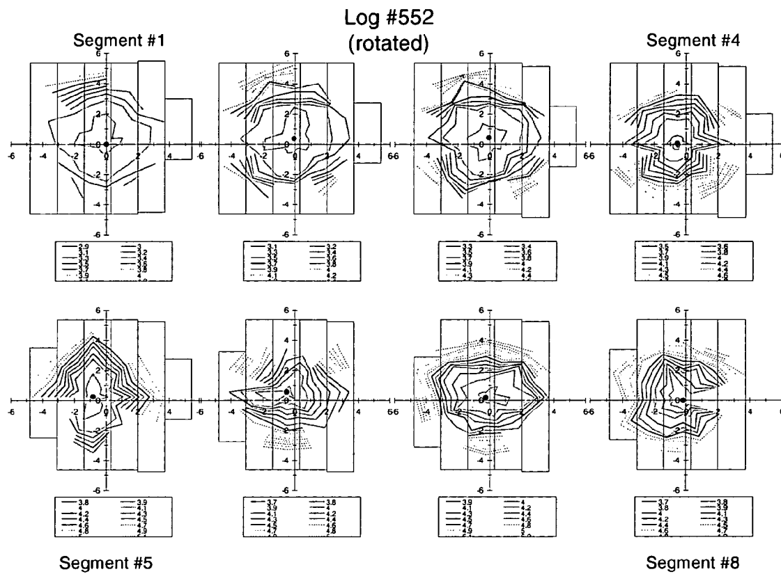
Figure 15. Sound velocity maps for log #552, after rotation and translation of the sawing diagram.
