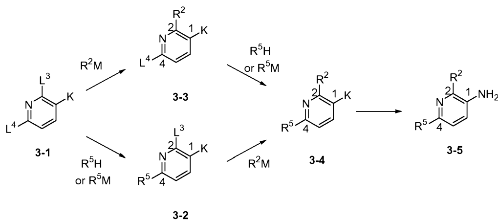
Scheme 3
