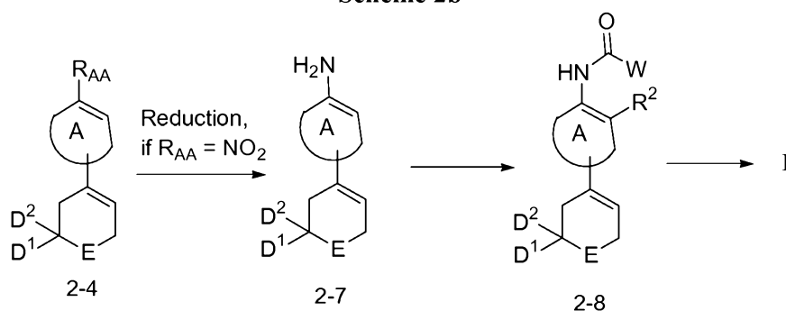
Scheme 2b
