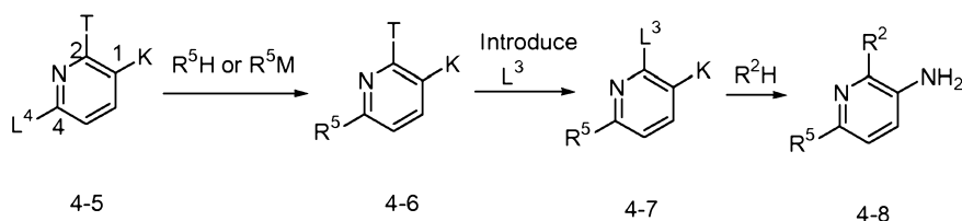
Scheme 4b
