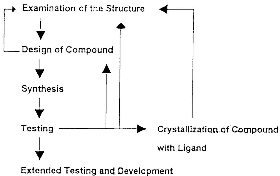
Figure 1. Design of Ligands that Interact with Nuclear Superfamily Members
