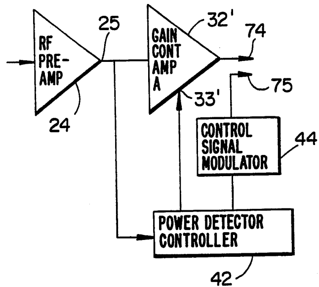
Fig - 10 PRE-TRANSMISSION PROCESSOR
