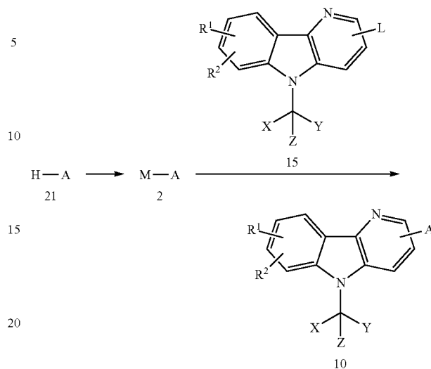
Scheme 8
