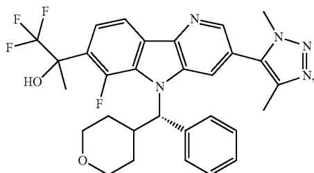
Diastereomer B
