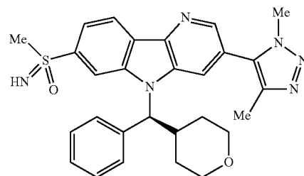
Diastereomer B
