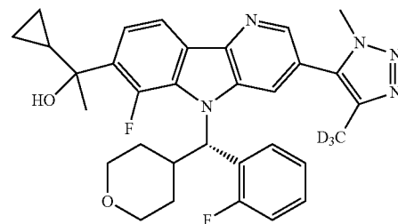
Diastereomer A
