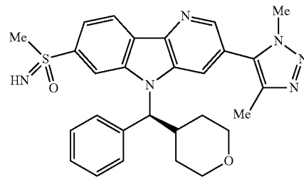
Diastereomer A
