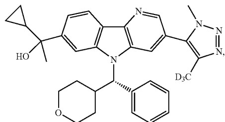
Diastereomer B
