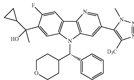
Diastereomer B
