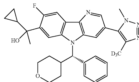
Diastereomer A
