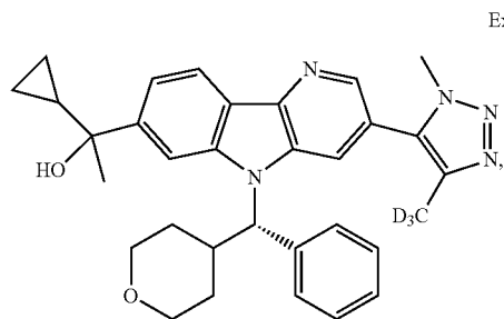
Diastereomer A
