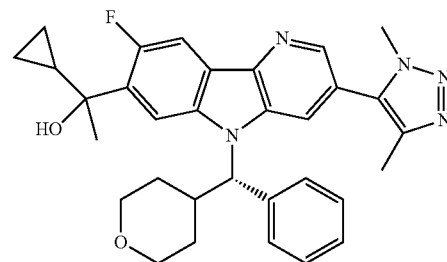
Diastereomer A
