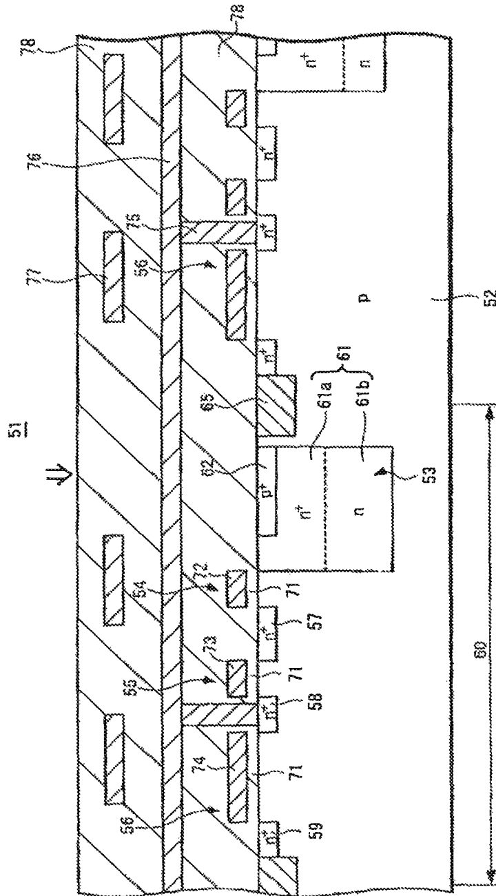
FIG. 1 (RELATED ART)
