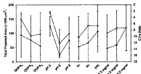
Figure 6. Results of Robust Design experiment on 316L stainless steel. (●: total projected cellular area, □: C/Fe ratio)
