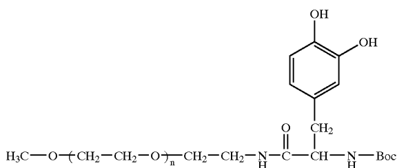
Example 10b
