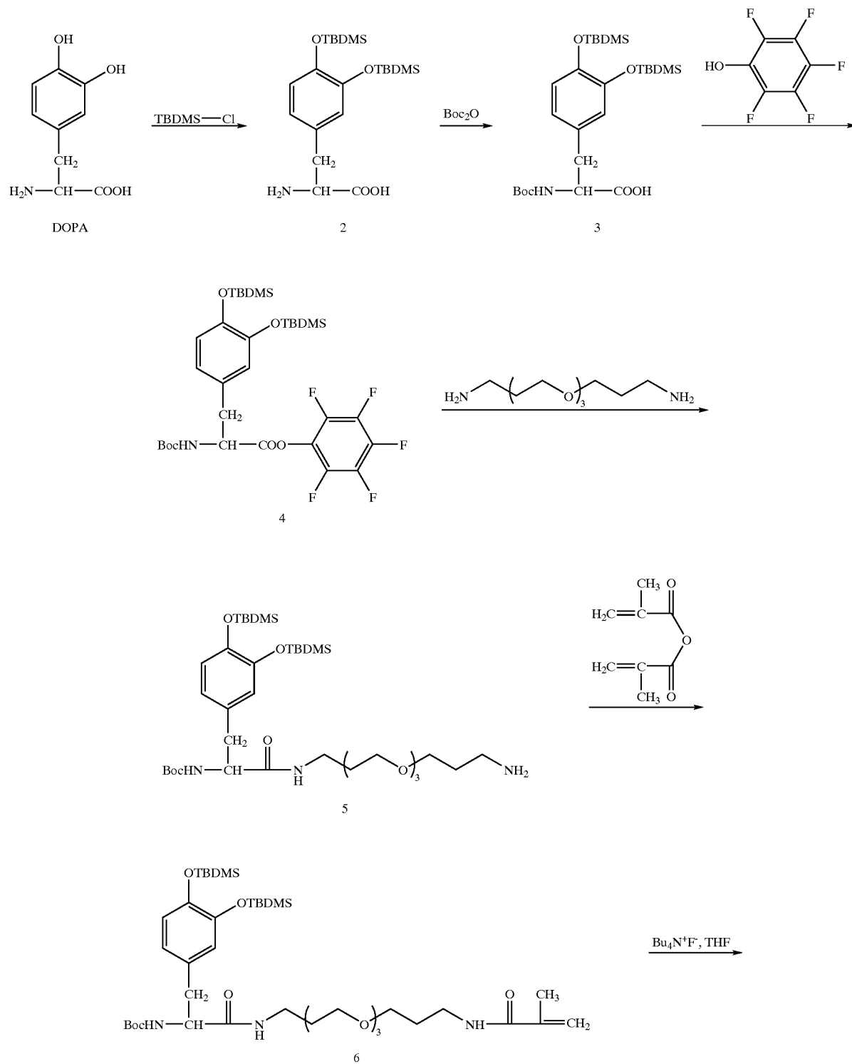
SCHEME 3
