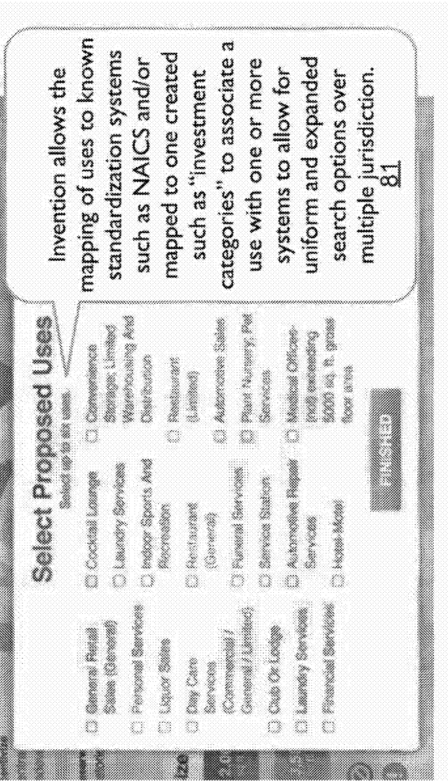
Fig 37 - Search Capability
