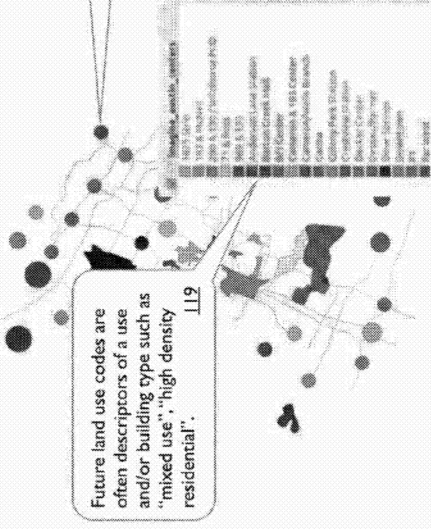
Fig 42 - Future Determinations
