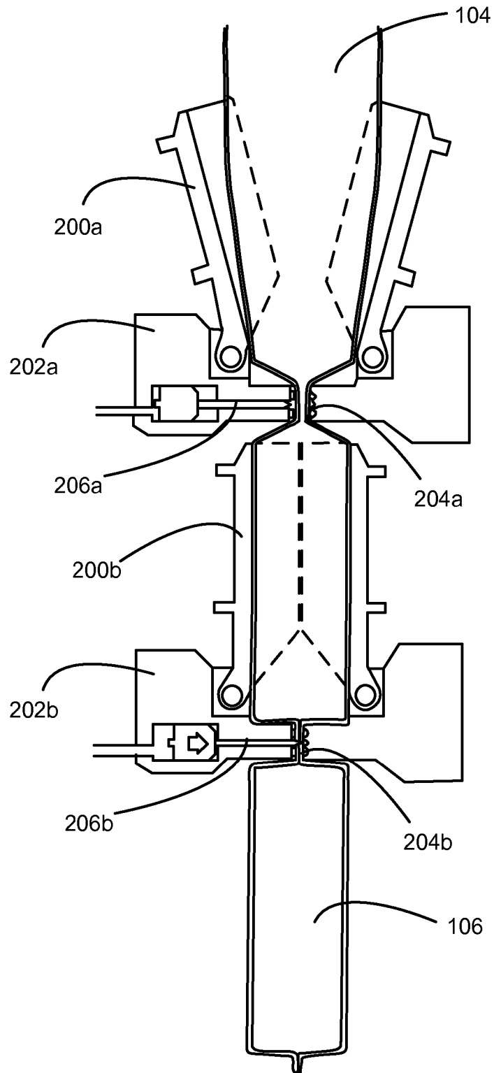
Fig 2 PRIOR ART
