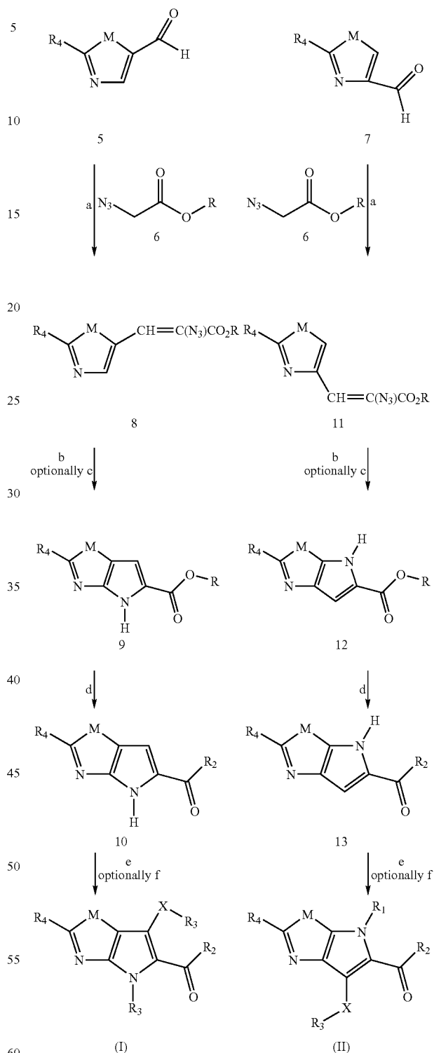
Scheme 2
