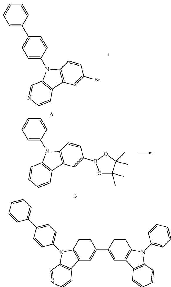
Reaction Scheme 1
