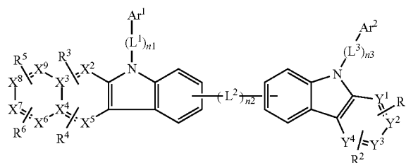
Chemical Formula 5
