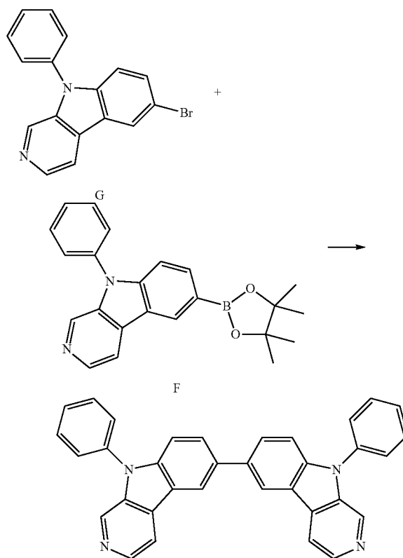
Reaction Scheme 6
