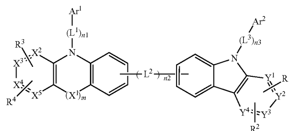
Chemical Formula 2
