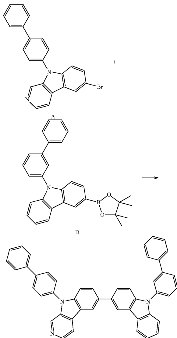
Reaction Scheme 3
