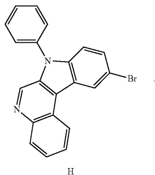
Reaction Scheme 7
