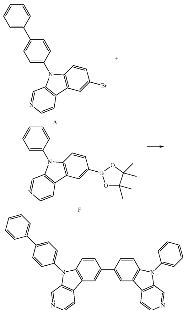
Reaction Scheme 5
