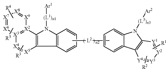
Chemical Formula 6
