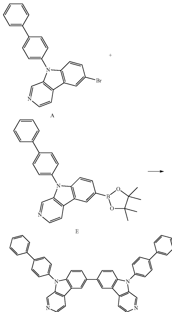
Reaction Scheme 4
