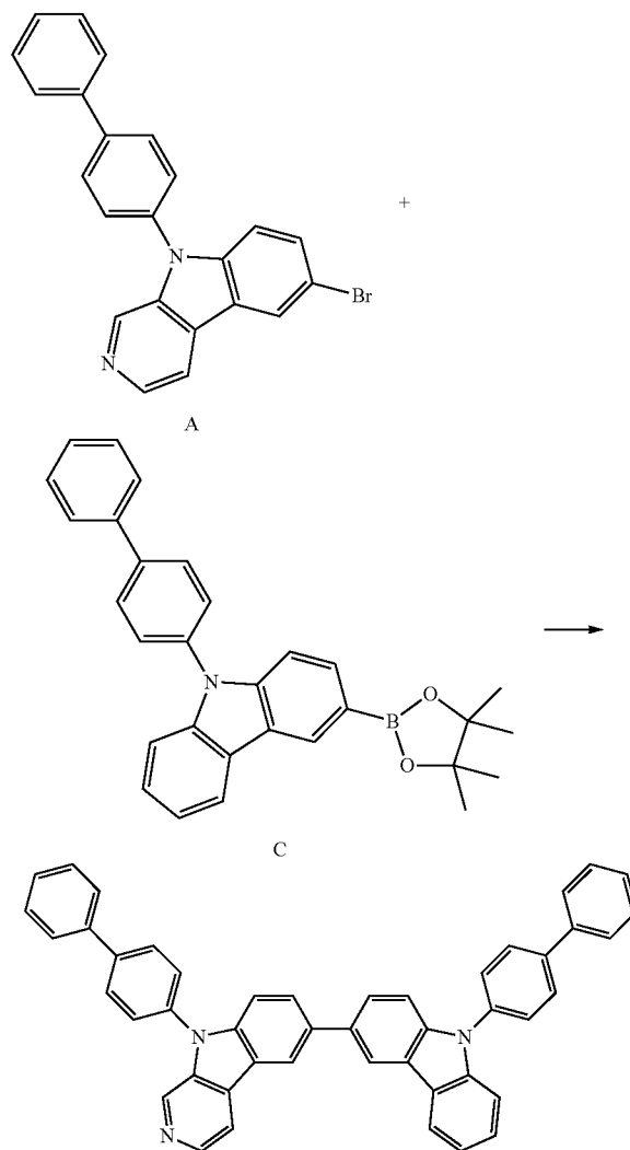
Reaction Scheme 2
