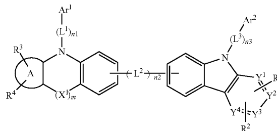
Chemical Formula 1
