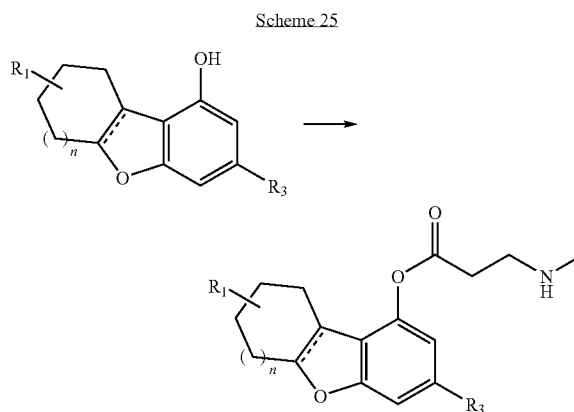
Synthesis of Compound C6S-39: 3-Methylamino-propionic acid 3-(1,1-dimethylheptyl)-7,7-dimethyl-5a,6,7,8,9,9a-hexahydro-dibenzofuran-1-yl ester
