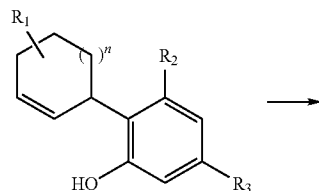
Scheme 17
