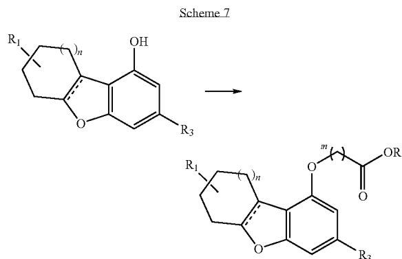
Synthesis of Compound C6S-9: [3-(1,1-Dimethylpentyl)-5a,6,7,8,9,9a-hexahydro-dibenzofuran-1-yloxy]-acetic acid
