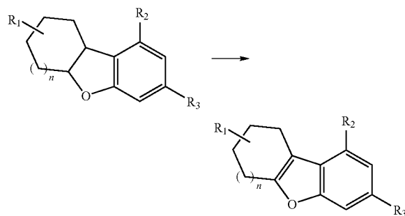
Synthesis of Compound C6M-10: 3-(1,1-Dimethylheptyl)-7,7-dimethyl-6,7,8,9-tetrahydro-dibenzofuran-1-ol
