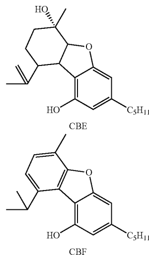
Scheme 1
