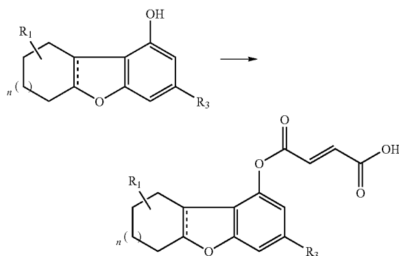
Scheme 21
