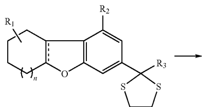
Scheme 20
