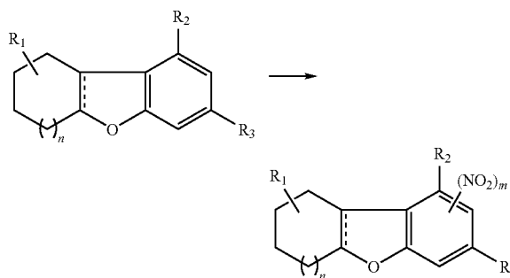
Scheme 15
