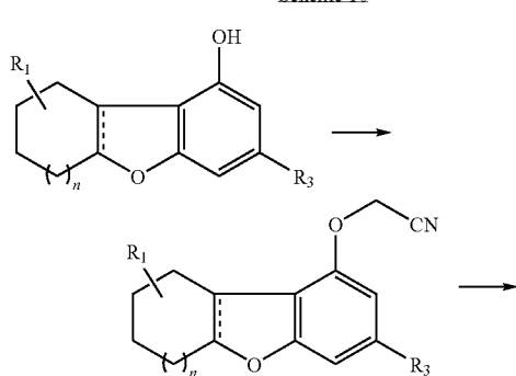
Scheme 10
