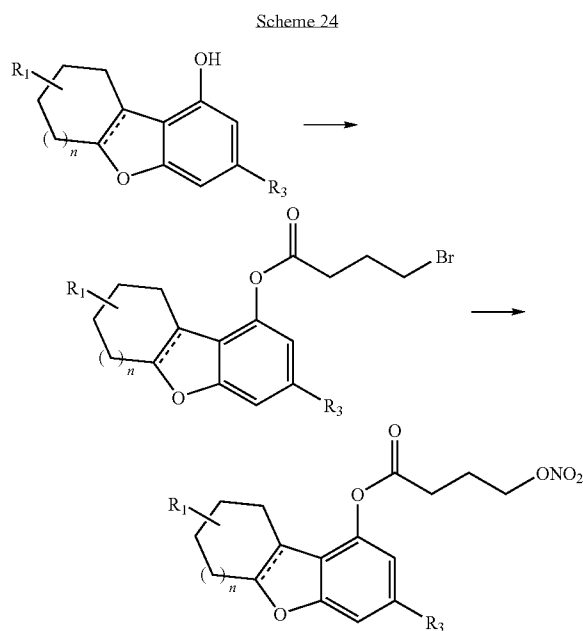
Synthesis of Compound C6S-24: 4-Nitrooxy-butyric acid 3-(1,1-dimethylpentyl)-5a,6,7,8,9,9a-hexahydro-dibenzofuran-1-yl ester
