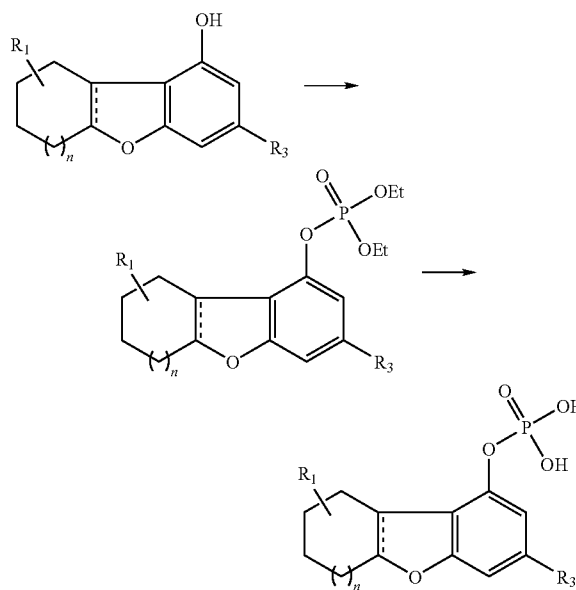
Scheme 23
