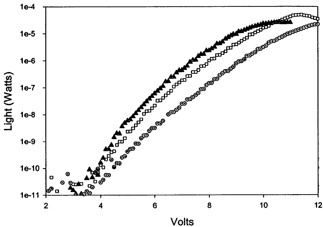
Light vs Voltage Plots for Examples 1-3
