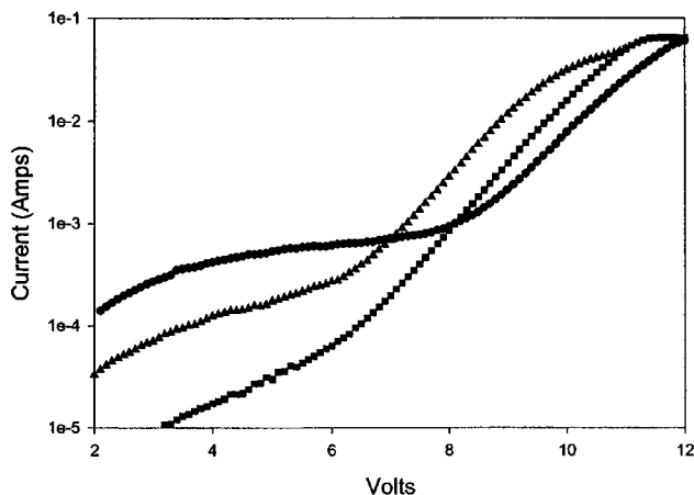
Current vs Voltage Plots for Examples 1-3
