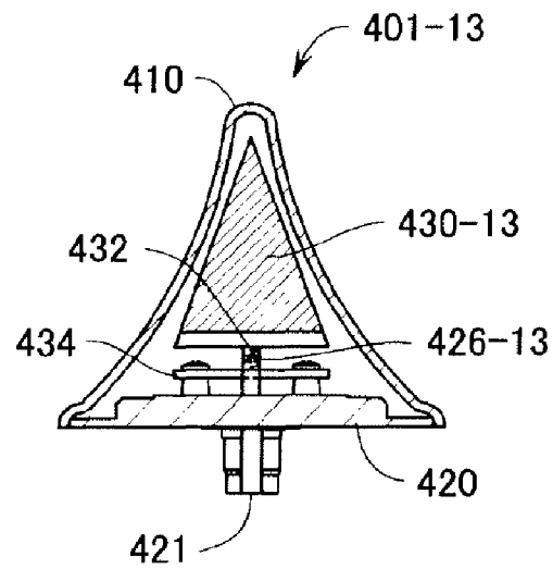
line b13-b13 sectional view
