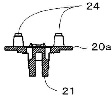
line A-A sectional view
