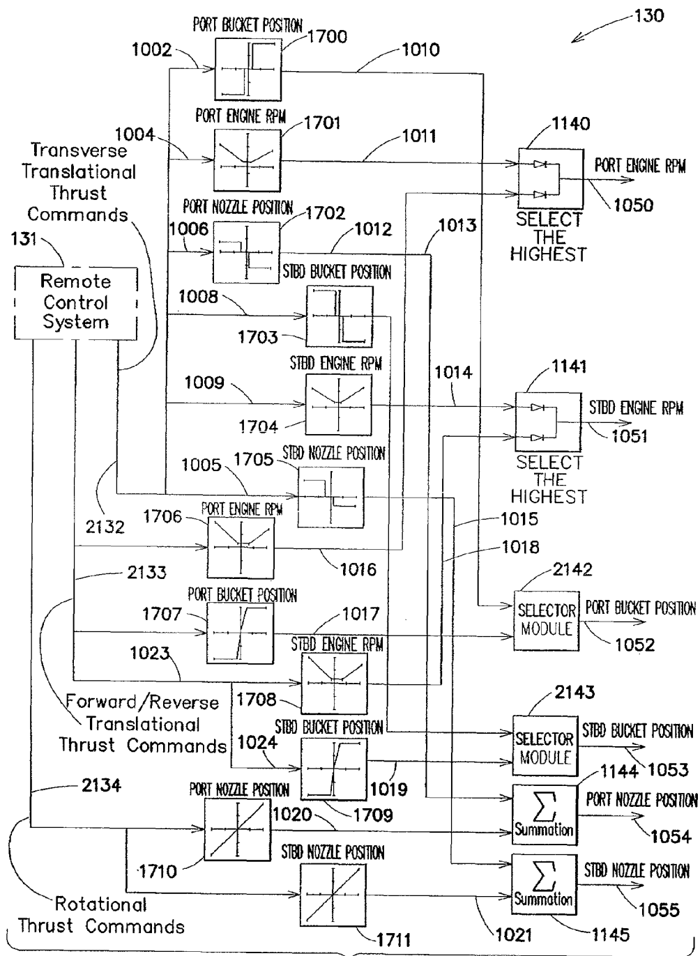
TWIN WATERJET SIGNAL DIAGRAM REMOTELY CONTROLLED
