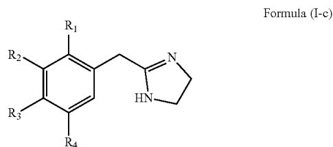
Formula (I-c)
