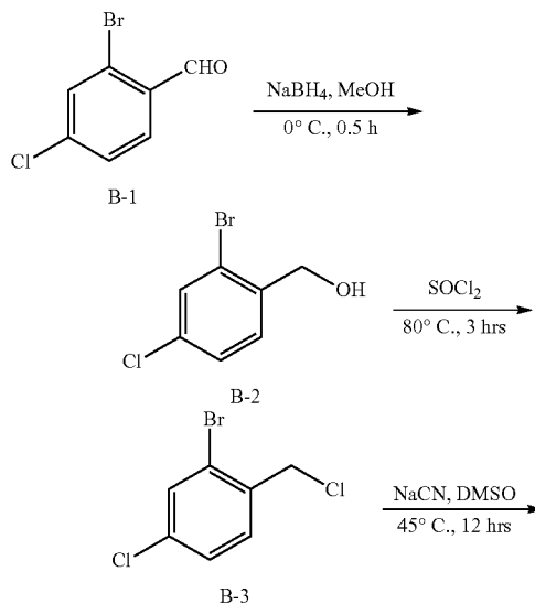
Scheme 2: Preparation of Compound 27
