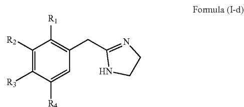
Formula (I-d)
