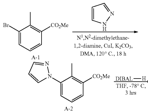
Scheme 1: Preparation of Compound 22
