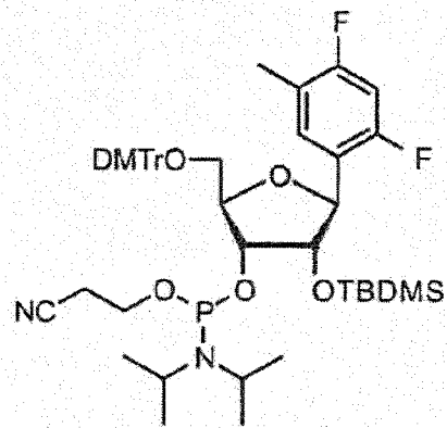
DFT Amidite
