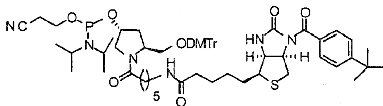
Biotin-Hyp Amidite
