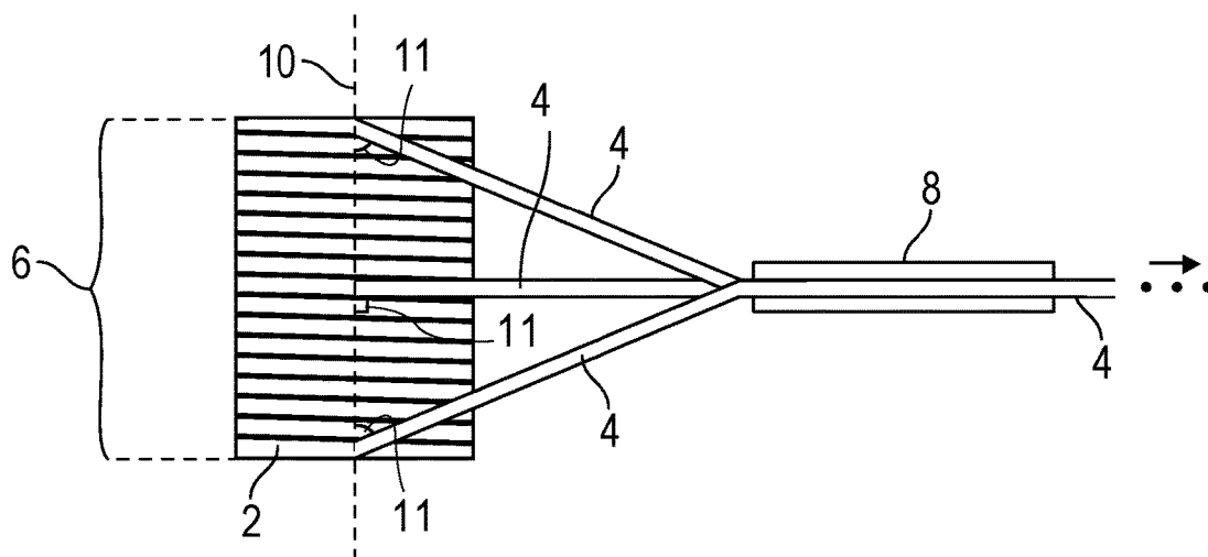
Fig. 2 (Prior Art)
