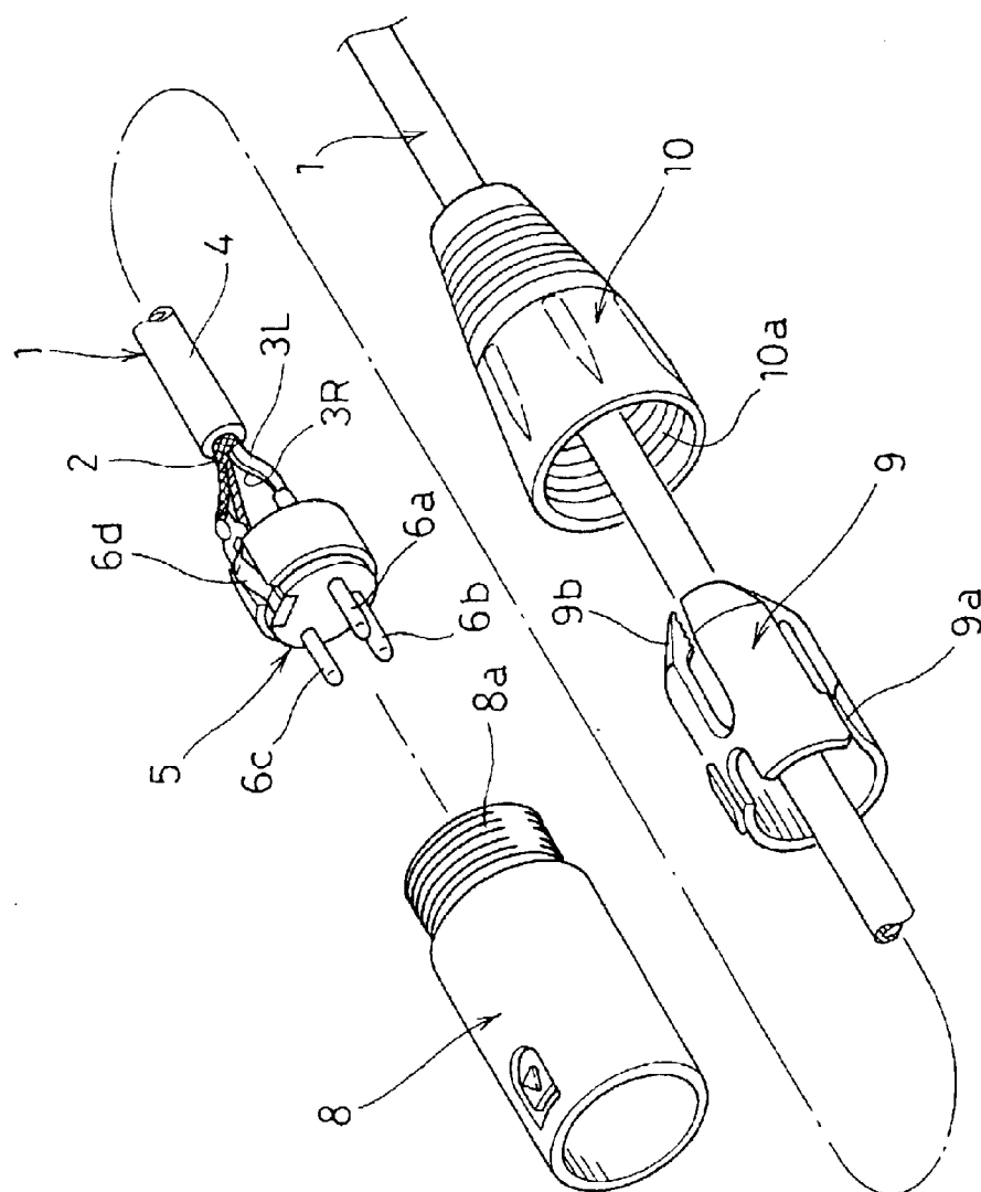
FIG. 6 PRIOR ART
