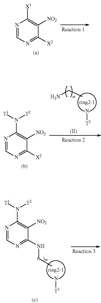
Reaction scheme 1
