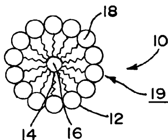
NORMAL MICELLE (L1)
