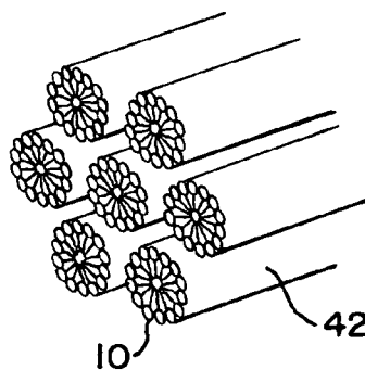
NORMAL HEXAGONAL (H1)
