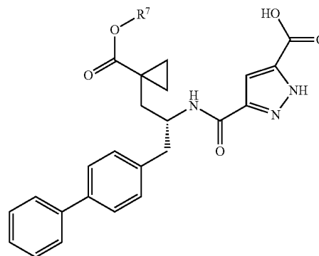
A. 5-[(R)-2-Biphenyl-4-yl-1-(1-carboxy-cyclopropylmethyl)-ethylcarbamoyl]-2H-pyrazole-3-carboxylic acid (R 7 =H)
