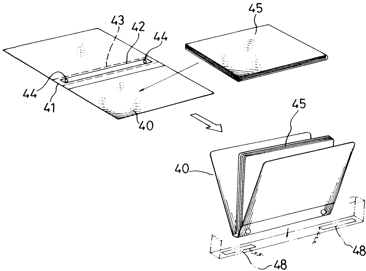
FIG. 24 (PRIOR ART)
