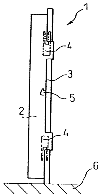
Fig. 6 (PRIOR ART)
