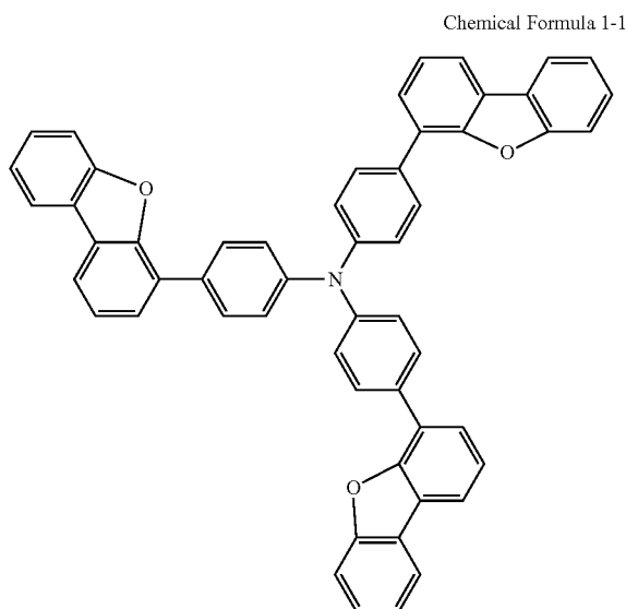
Synthetic Example
