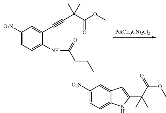
Methyl 2-methyl-2-(5-nitro-1H-indol-2-yl)propanoate
