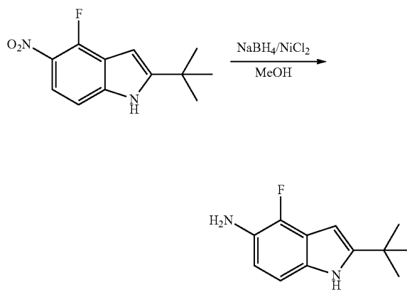
2-tert-Butyl-4-fluoro-1H-indol-5-amine
