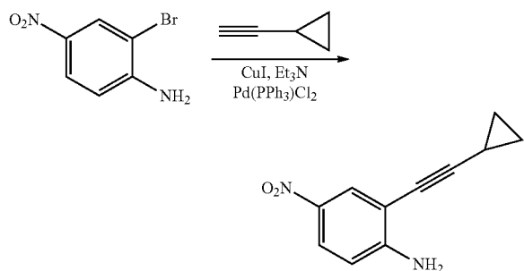
2-(Cyclopropylethynyl)-4-nitroaniline
