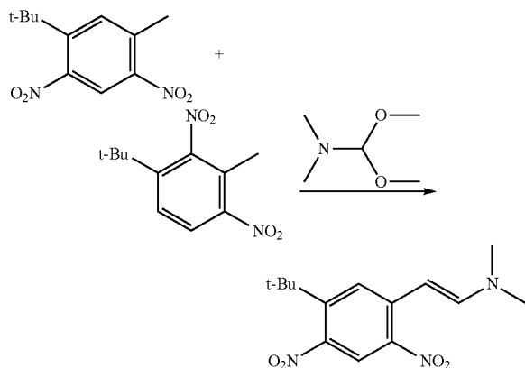
(E)-2-(5-tert-Butyl-2,4-dinitrophenyl)-N,N-dimethylethanamine
