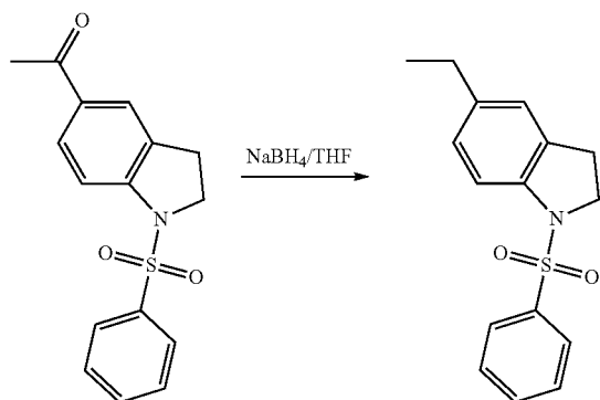
5-Ethyl-1-(phenylsulfonyl)indoline
