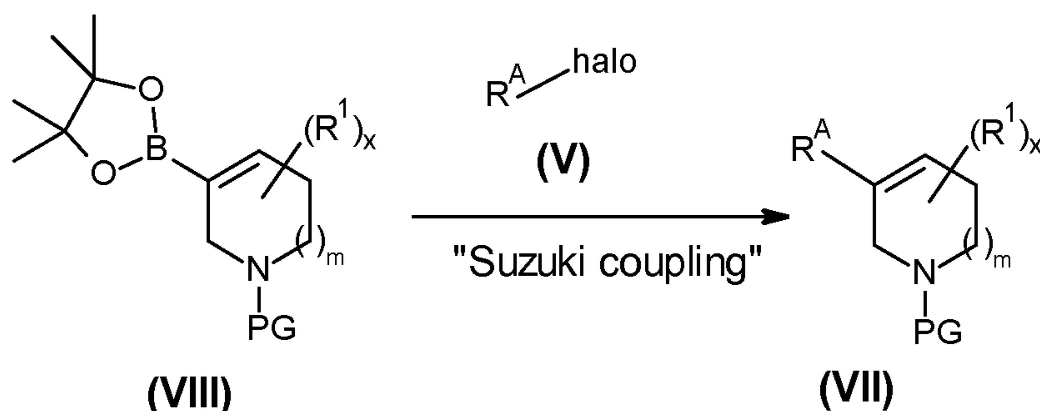
Reaction scheme 9
