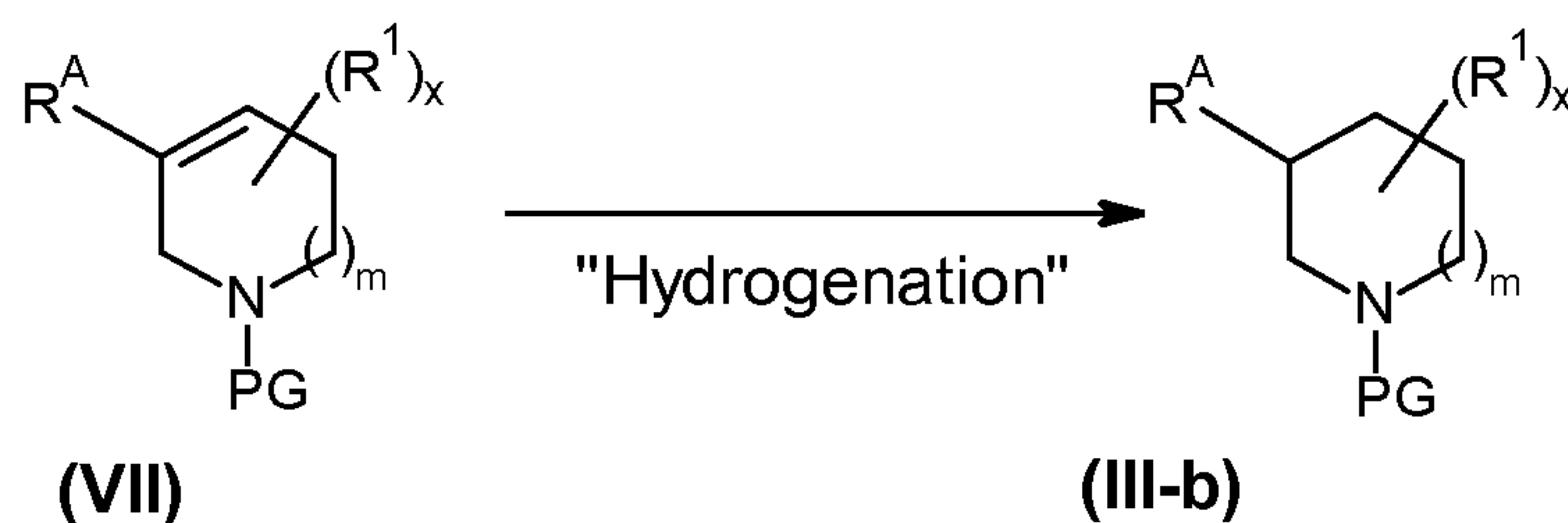
Reaction scheme 8
