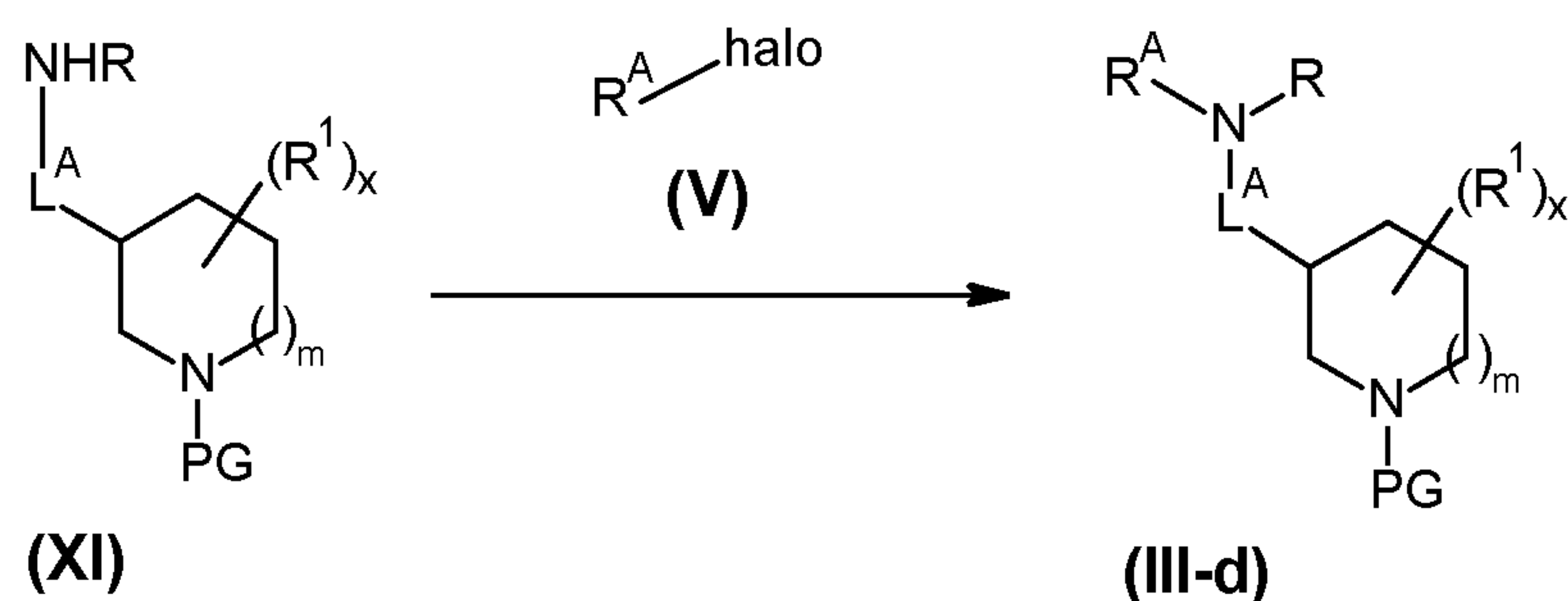
Reaction scheme 12
