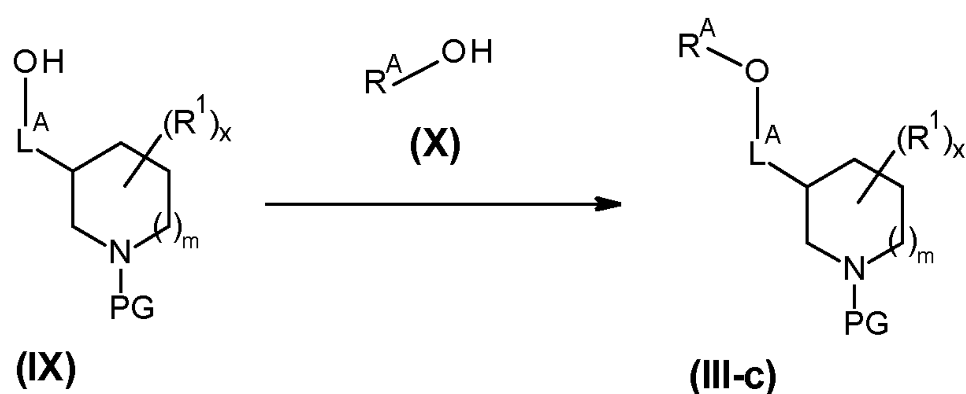
Reaction scheme 11
