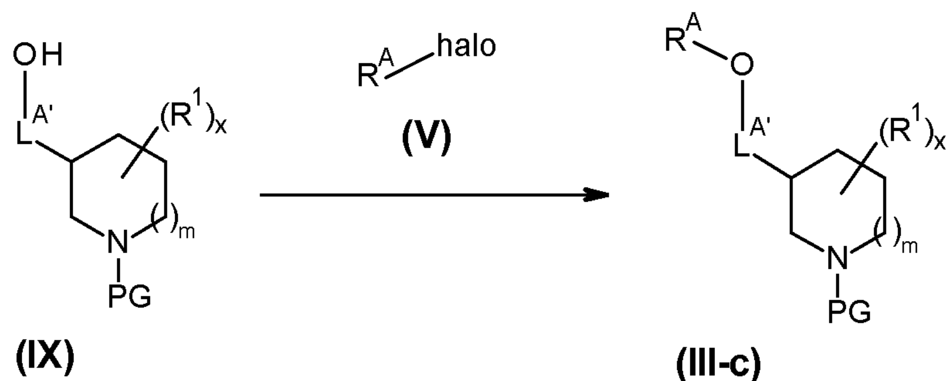
Reaction scheme 10
