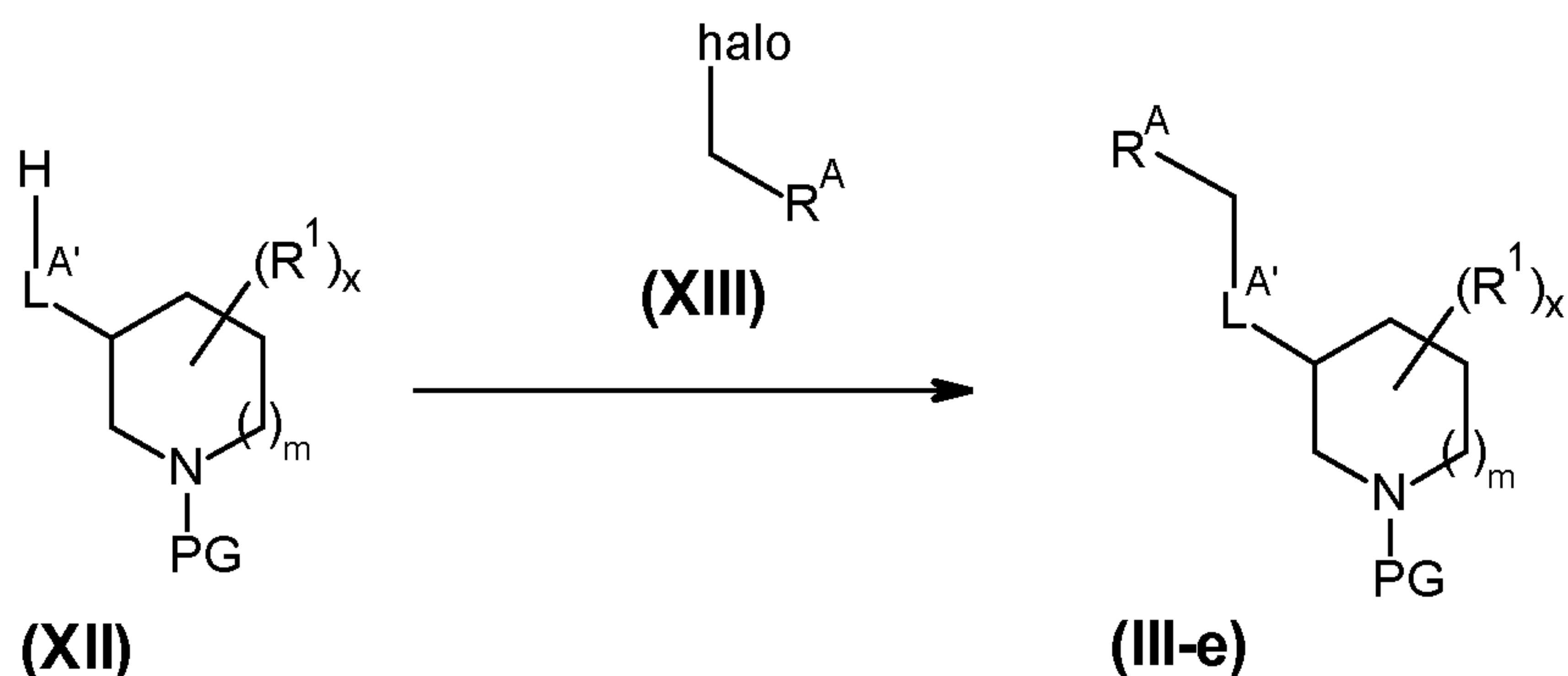
Reaction scheme 13
