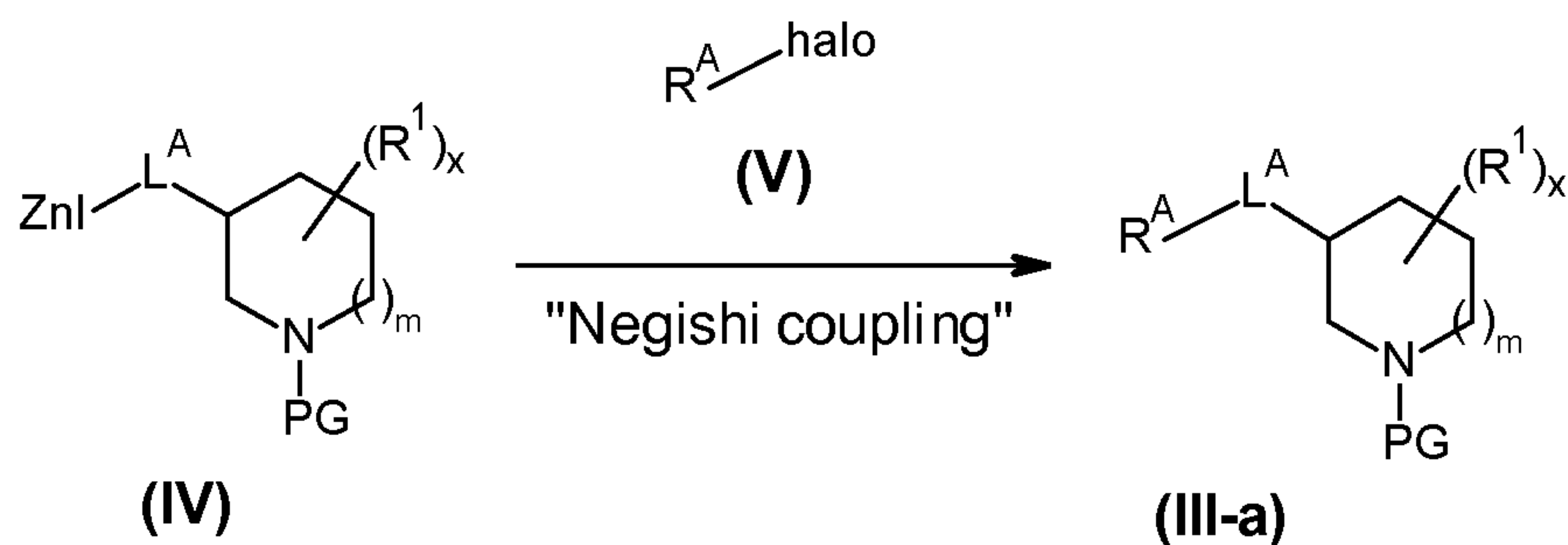
Reaction scheme 6
