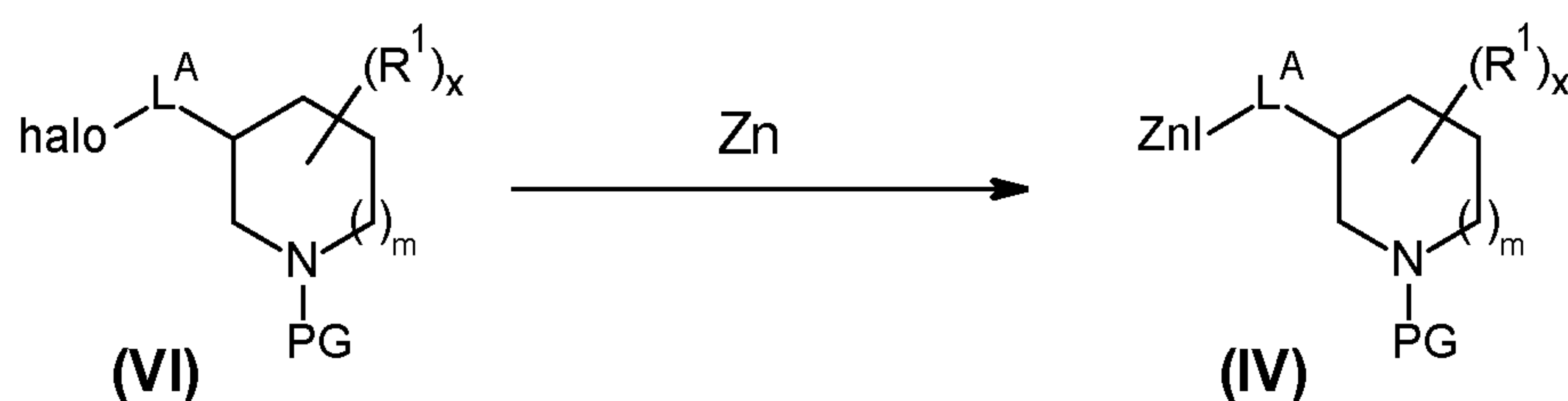
Reaction scheme 7
