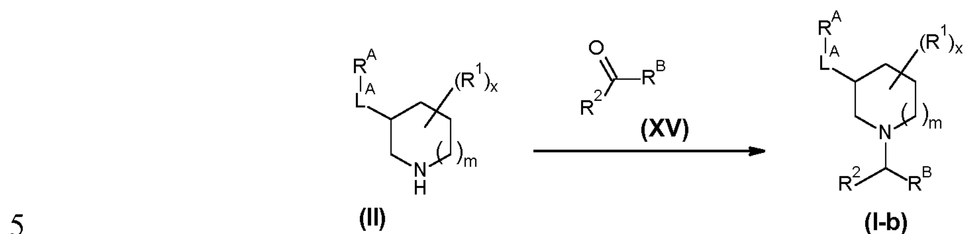
Reaction scheme 2
