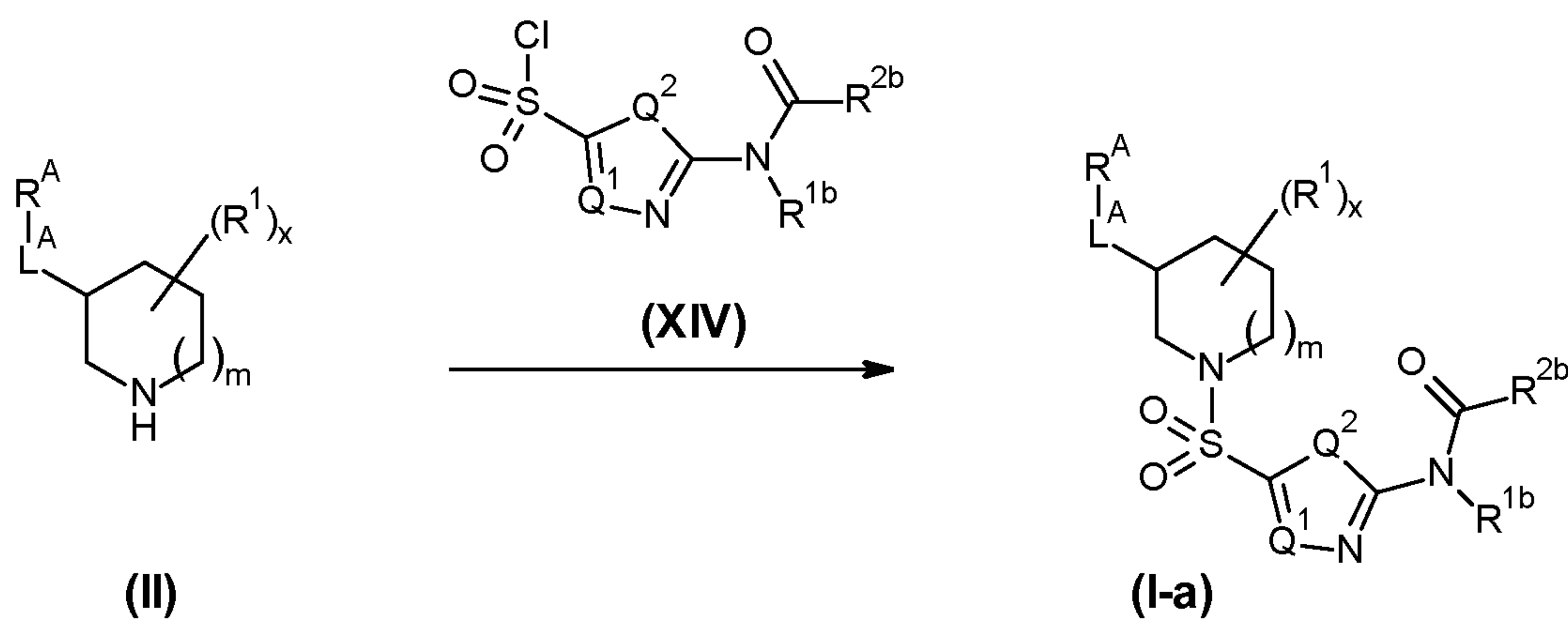
Reaction scheme 1
