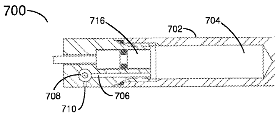
FIG. 7B (Side View)
