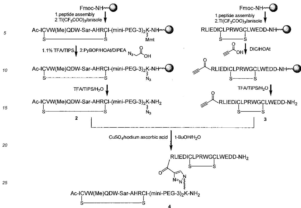
Peptide 17-ABP ("4" in the scheme above)
