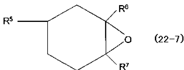
[Chemical Formula 37]
