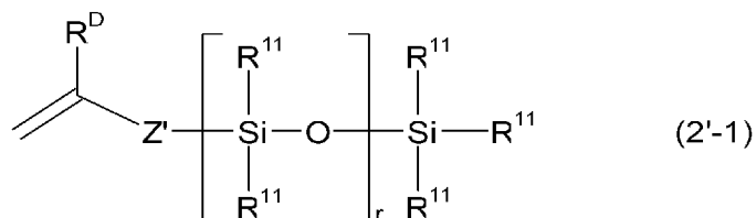
[Chemical Formula 24]
