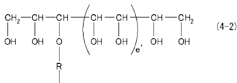
[Chemical Formula 17]
