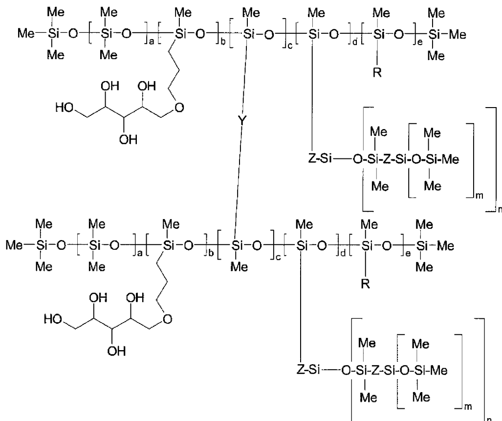
[Chemical Formula 40]
