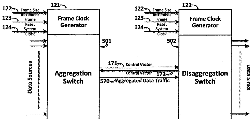
Key Details of an Aggregation / Disaggregation Switch Pair
