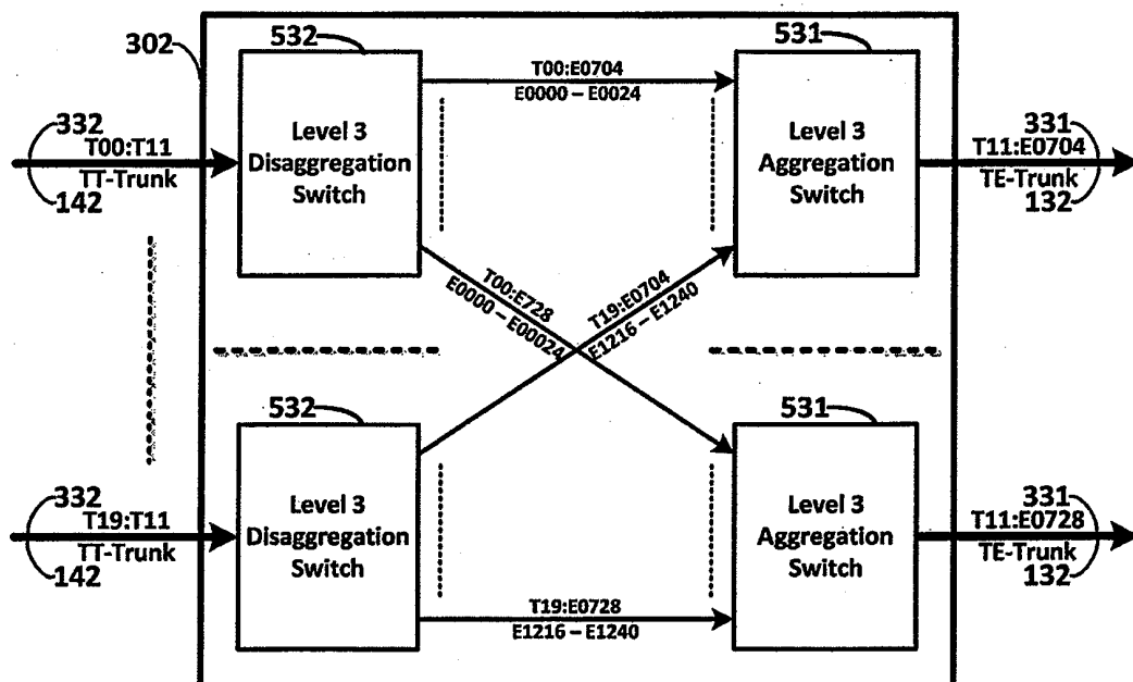
Destination T-Node 11 example using a Crossconnect Switch to finish the Many-to-One Mapping from 20 T-Nodes to the 25 E-Node children of T-Node 11
