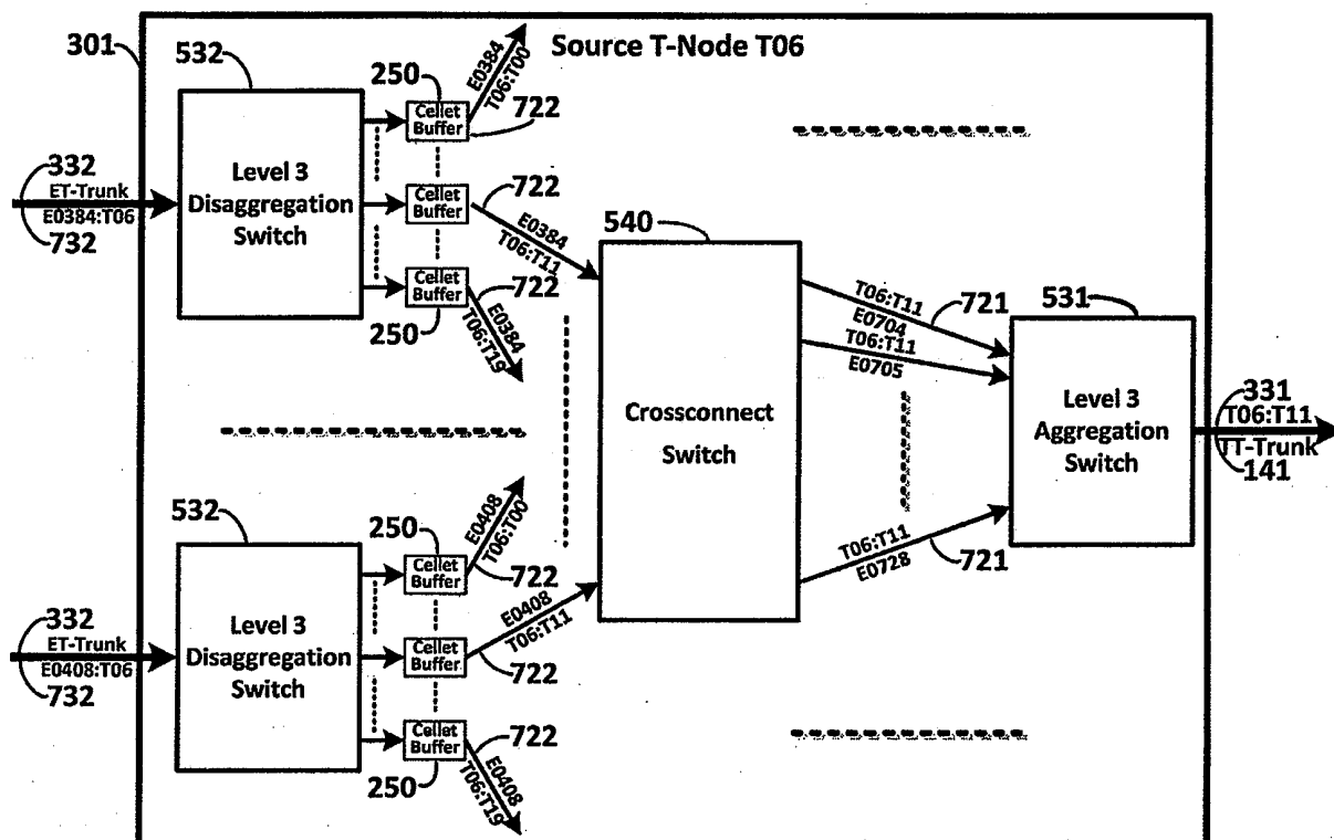
Source T-Node 06 example using a Crossconnect Switch to initiate reorienting each of the 25 Level 2 aggregations of 499 paths from One-to-Many to Many-to-One
