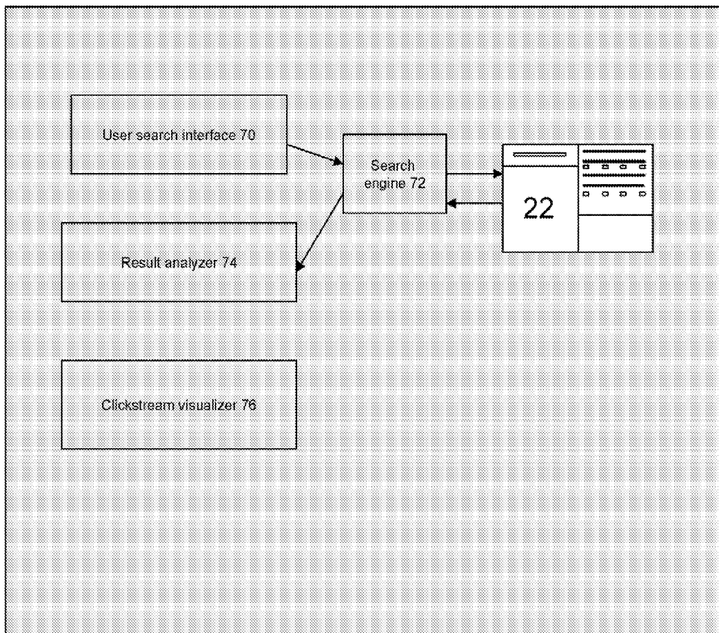
Standalone architecture
