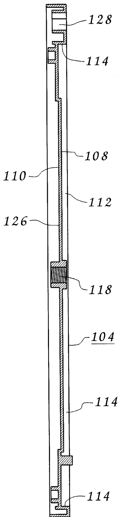
FIG. 11 PRIOR ART
