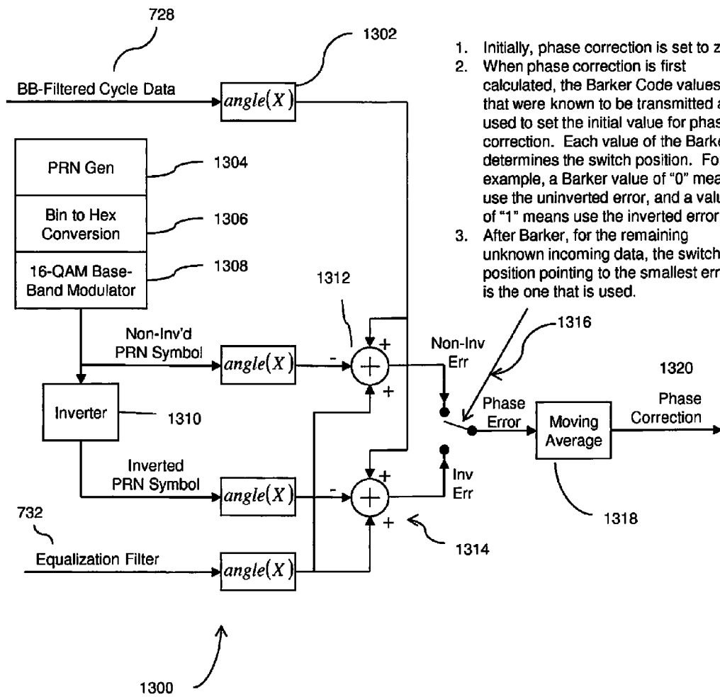
Figure 13 Phase Correction
